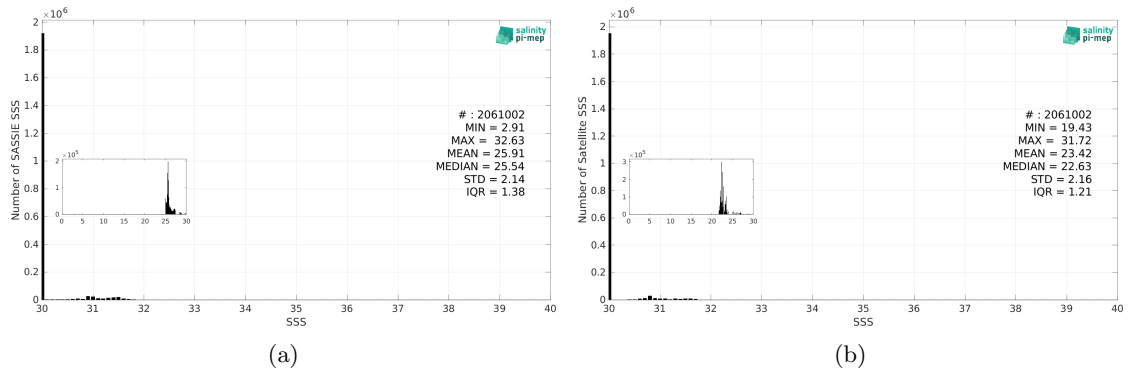
Figure 3: Histograms of SSS from SASSIE (a) and ISAS v7 - Monthly (Ifremer-LOPS-CMEMS) (b) considering all match-up pairs per bins of 0.1 over the Global Ocean Pi-MEP region and for the full satellite product period.
