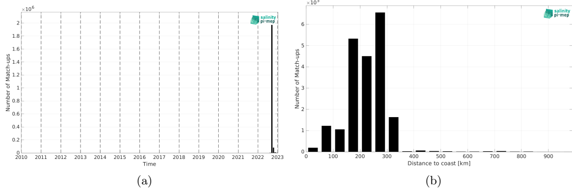
Figure 2: Number of match-ups between SASSIE and ISAS v7 - Monthly (Ifremer-LOPS-CMEMS) SSS as a function of time (a) and as function of the distance to coast (b) over the Global Ocean Pi-MEP region and for the full satellite product period.
