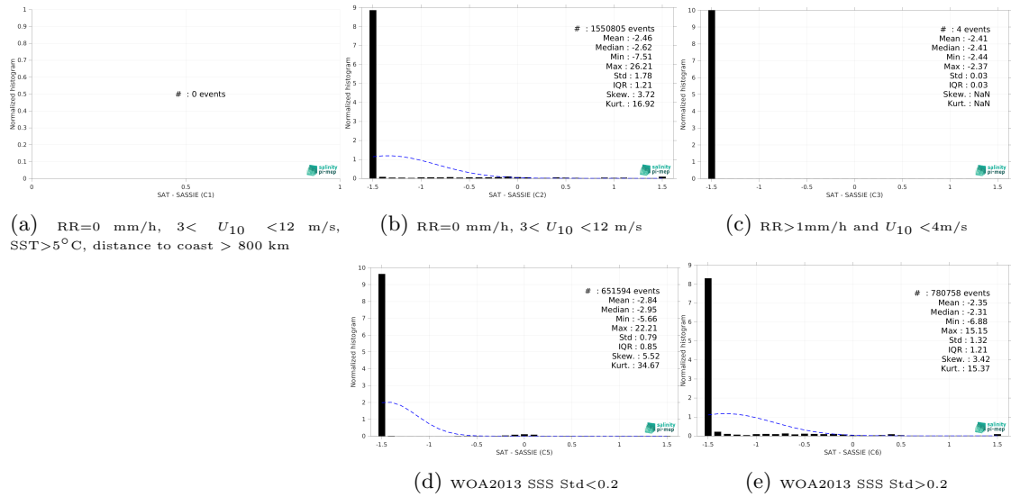
Figure 15: Normalized histogram of \Delta SSS (ISAS v7 - Monthly (Ifremer-LOPS-CMEMS) - SASSIE) for 5 different subdatasets corresponding to: RR=0 mm/h, 3 < U_{10} < 12 m/s, SST>5°C, distance to coast > 800 km (a), RR=0 mm/h, 3 < U_{10} < 12 m/s (b), RR>1mm/h and U_{10} < 4 m/s (c), WOA2013 SSS Std<0.2 (d), WOA2013 SSS Std>0.2 (e).
