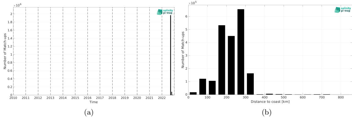
Figure 2: Number of match-ups between SASSIE and ISAS SSS as a function of time (a) and as function of the distance to coast (b) over the Global Ocean Pi-MEP region and for the full satellite product period.
