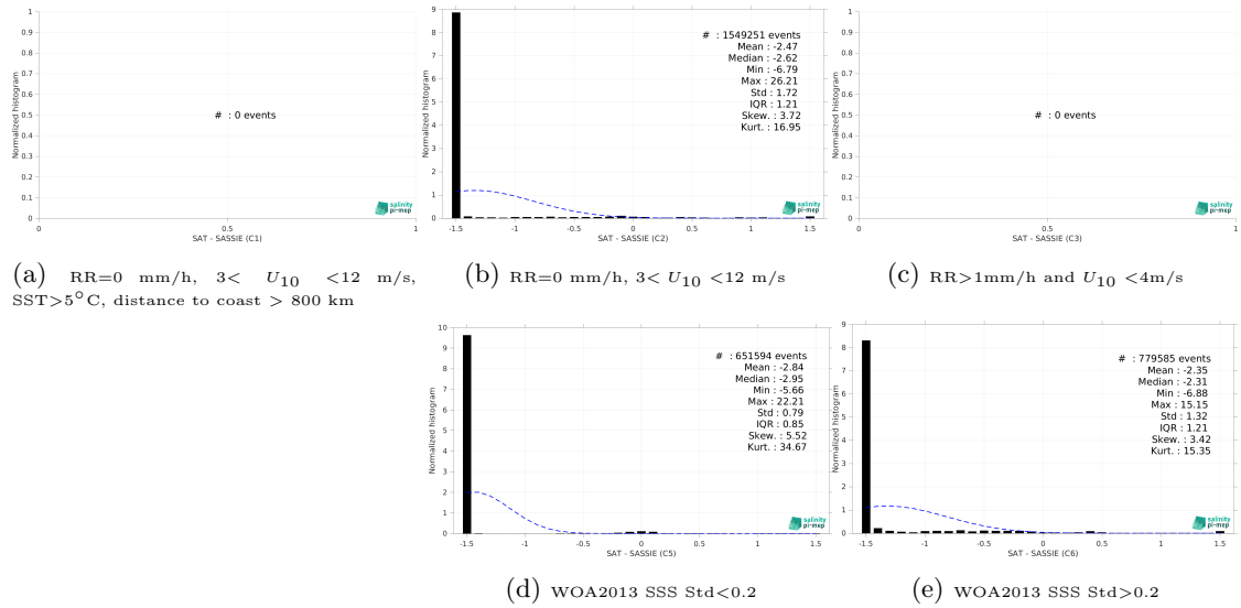
Figure 15: Normalized histogram of \Delta SSS (ISAS - SASSIE) for 5 different subdatasets corresponding to: RR=0 mm/h, 3 < U_{10} < 12 m/s, SST>5°C, distance to coast > 800 km (a), RR=0 mm/h, 3 < U_{10} < 12 m/s (b), RR>1mm/h and U_{10} < 4 m/s (c), WOA2013 SSS Std<0.2 (d), WOA2013 SSS Std>0.2 (e).
