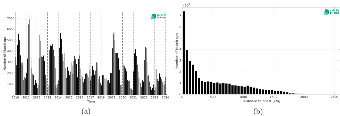
Figure 2: Number of match-ups between Marine mammals and ISAS SSS as a function of time (a) and as function of the distance to coast (b) over the Global Ocean Pi-MEP region and for the full satellite product period.
