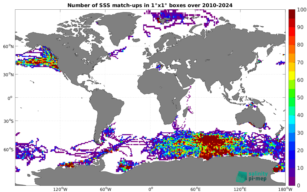
Figure 5: Number of SSS match-ups between Marine mammals SSS and the ISAS SSS product for the Global Ocean Pi-MEP region over 1^\circ \times 1^\circ boxes and for the full satellite product period.
