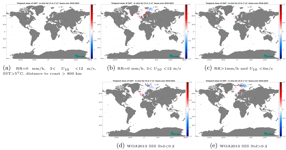
Figure 14: Temporal mean gridded over spatial boxes of size 1^\circ \times 1^\circ of \Delta SSS (ISAS v7 - Monthly (Ifremer-LOPS-CMEMS) - ICES) for 5 different subdatasets corresponding to:RR=0 mm/h, 3 < U_{10} < 12 m/s, SST > 5^\circ\text{C} , distance to coast > 800 km (a), RR=0 mm/h, 3 < U_{10} < 12 m/s (b), RR > 1 mm/h and U_{10} < 4 m/s (c), WOA2013 SSS Std < 0.2 (d), WOA2013 SSS Std > 0.2 (e).
