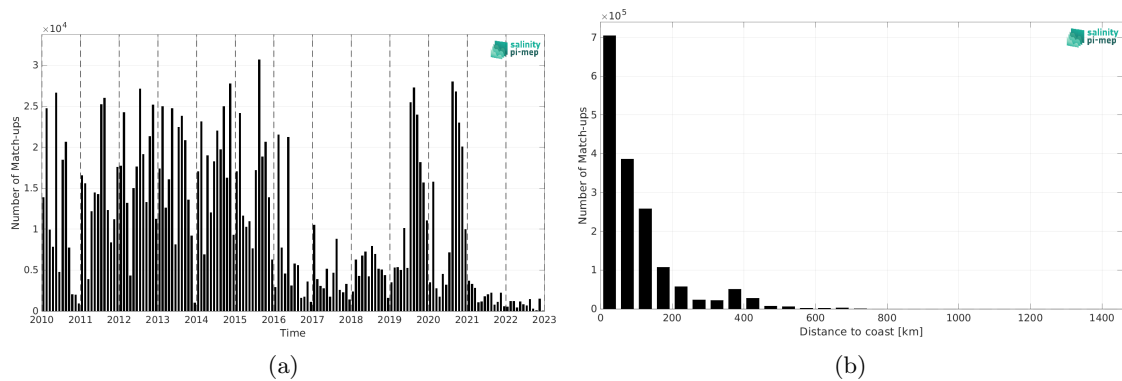
Figure 2: Number of match-ups between ICES and ISAS v7 - Monthly (Ifremer-LOPS-CMEMS) SSS as a function of time (a) and as function of the distance to coast (b) over the Global Ocean Pi-MEP region and for the full satellite product period.
