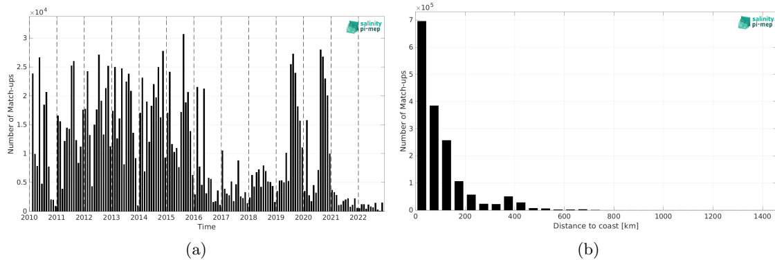
Figure 2: Number of match-ups between ICES and ISAS SSS as a function of time (a) and as function of the distance to coast (b) over the Global Ocean Pi-MEP region and for the full satellite product period.
