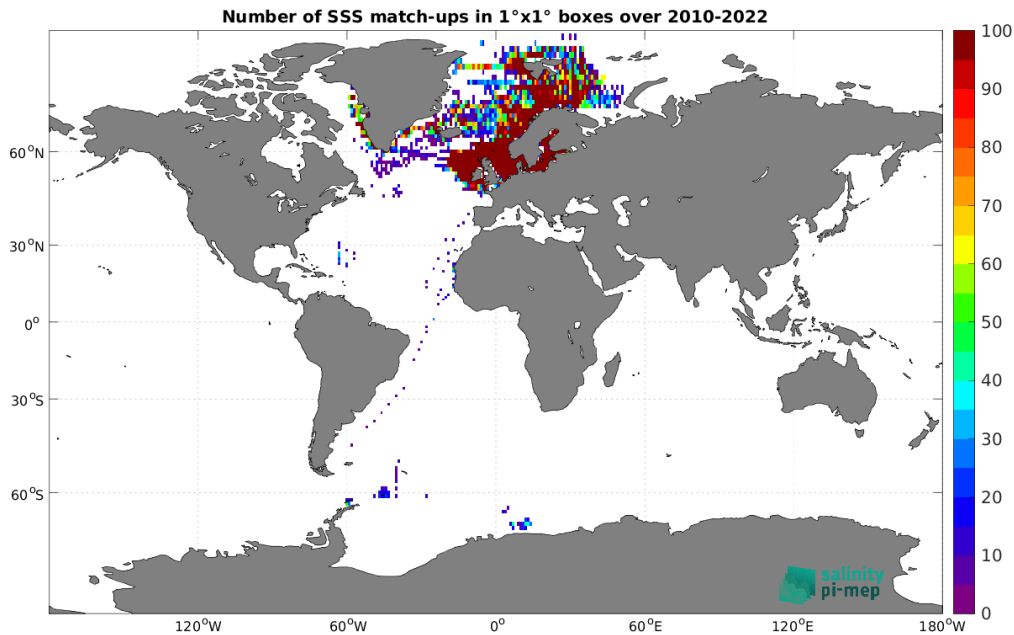
Figure 5: Number of SSS match-ups between ICES SSS and the ISAS SSS product for the Global Ocean Pi-MEP region over 1^\circ \times 1^\circ boxes and for the full satellite product period.
