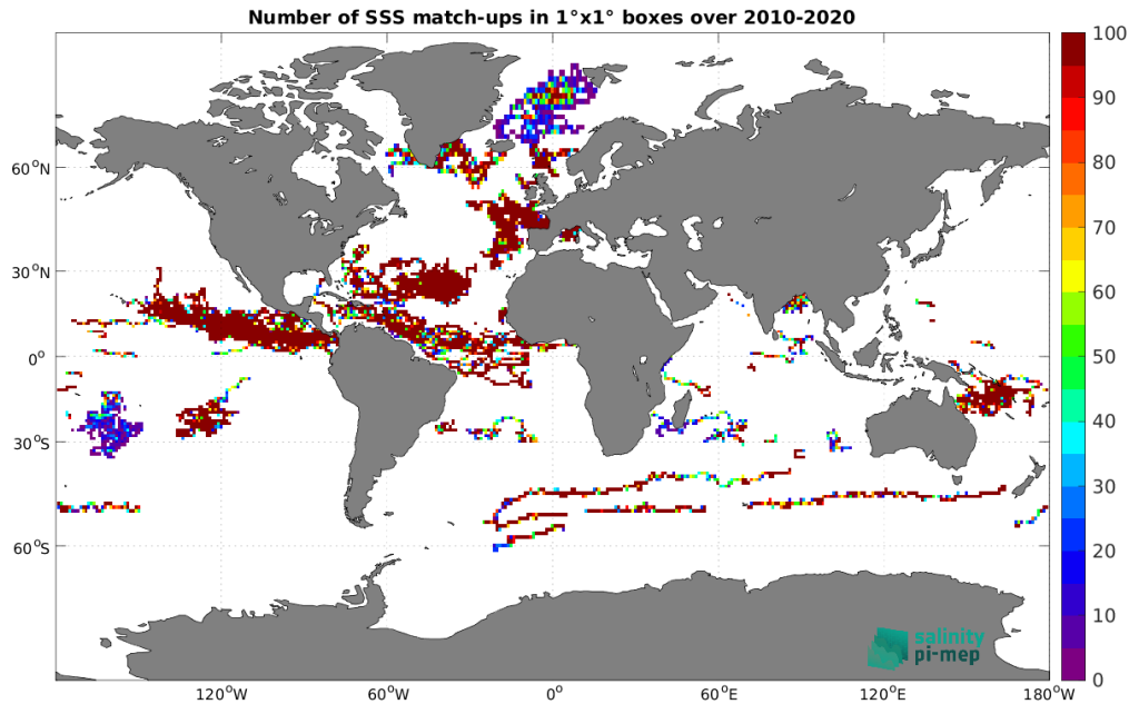
Figure 4: Number of SSS match-ups between Surface drifters SSS and the ISAS v7 - Monthly (Ifremer-LOPS-CMEMS) SSS product for the Global Ocean Pi-MEP region over 1^\circ \times 1^\circ boxes and for the full satellite product period.
