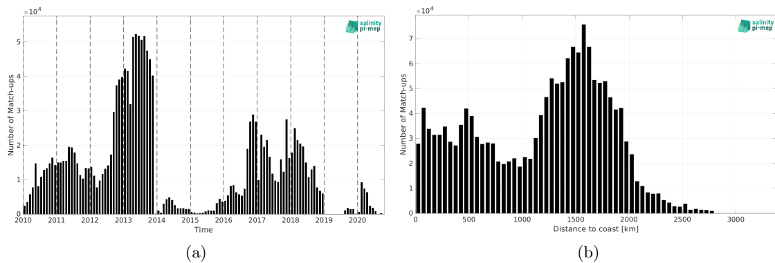
Figure 2: Number of match-ups between Surface drifters and ISAS v7 - Monthly (Ifremer-LOPS-CMEMS) SSS as a function of time (a) and as function of the distance to coast (b) over the Global Ocean Pi-MEP region and for the full satellite product period.
