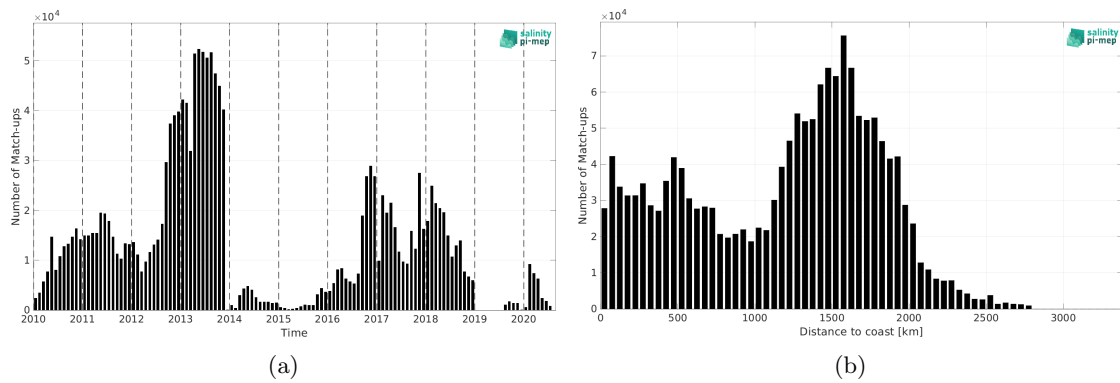
Figure 2: Number of match-ups between Surface drifters and ISAS SSS as a function of time (a) and as function of the distance to coast (b) over the Global Ocean Pi-MEP region and for the full satellite product period.
