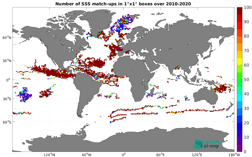
Figure 4: Number of SSS match-ups between Surface drifters SSS and the ISAS SSS product for the Global Ocean Pi-MEP region over 1^\circ \times 1^\circ boxes and for the full satellite product period.
