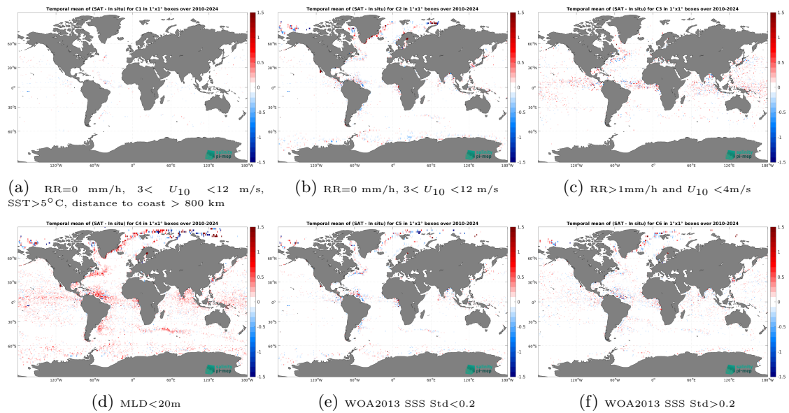
Figure 14: Temporal mean gridded over spatial boxes of size 1^\circ \times 1^\circ of \Delta SSS (ISAS v7 - Monthly (Ifremer-LOPS-CMEMS) - Argo) for 6 different subdatasets corresponding to:RR=0 mm/h, 3 < U_{10} < 12 m/s, SST>5°C, distance to coast > 800 km (a), RR=0 mm/h, 3 < U_{10} < 12 m/s (b), RR>1mm/h and U_{10} < 4 m/s (c),MLD<20m (d),WOA2013 SSS Std<0.2 (e),WOA2013 SSS Std>0.2 (f).
