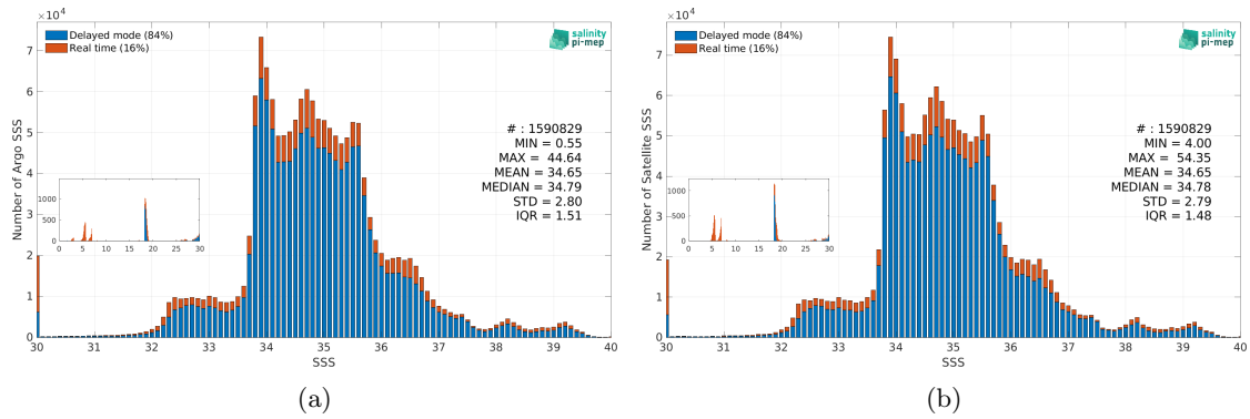
Figure 3: Histograms of SSS from Argo (a) and ISAS v7 - Monthly (Ifremer-LOPS-CMEMS) (b) considering all match-up pairs per bins of 0.1 over the Global Ocean Pi-MEP region and for the full satellite product period.
