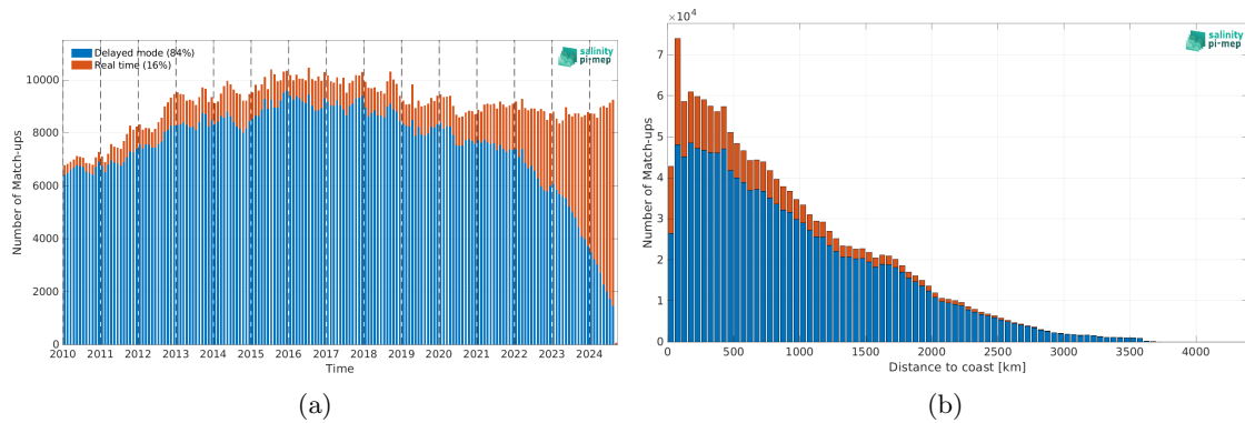
Figure 2: Number of match-ups between Argo and ISAS v7 - Monthly (Ifremer-LOPS-CMEMS) SSS as a function of time (a) and as function of the distance to coast (b) over the Global Ocean Pi-MEP region and for the full satellite product period.
