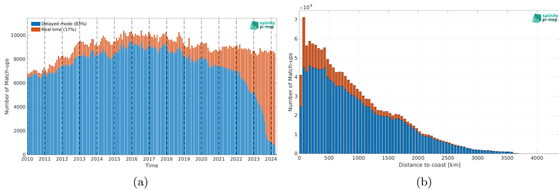
Figure 2: Number of match-ups between Argo and ISAS SSS as a function of time (a) and as function of the distance to coast (b) over the Global Ocean Pi-MEP region and for the full satellite product period.
