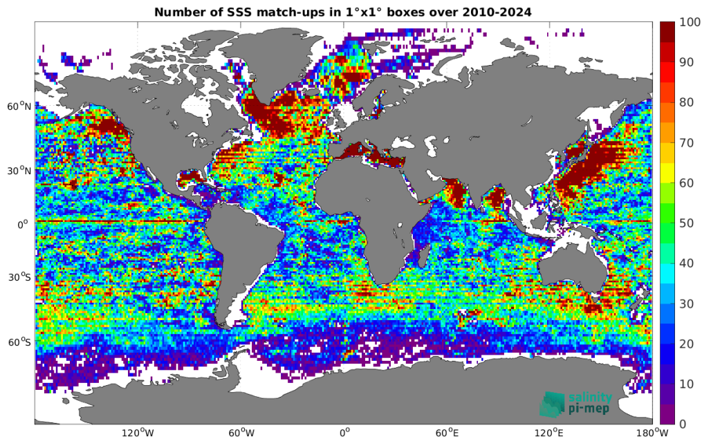
Figure 5: Number of SSS match-ups between Argo SSS and the ISAS SSS product for the Global Ocean Pi-MEP region over 1^\circ \times 1^\circ boxes and for the full satellite product period.
