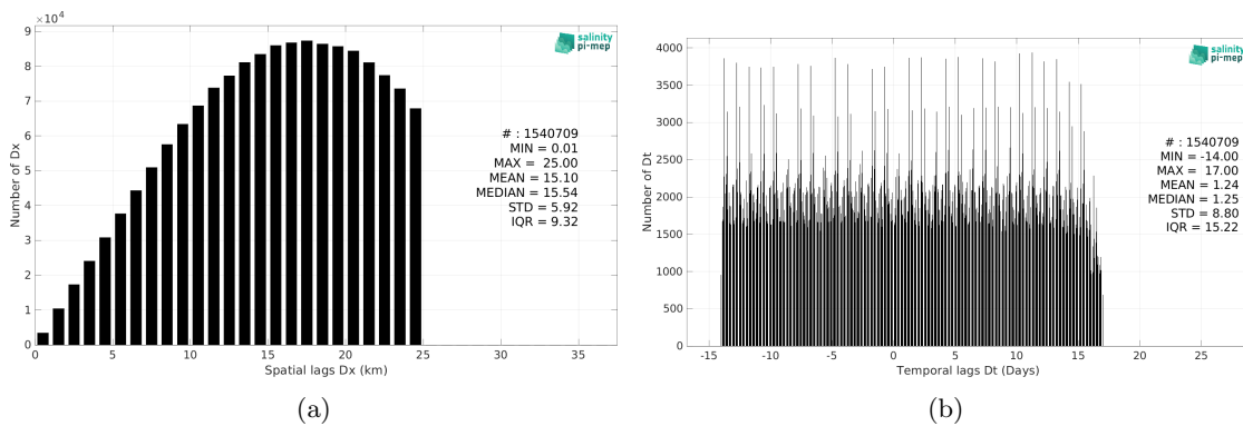
Figure 6: Histograms of the spatial (a) and temporal (b) lags between the location/time of the Argo measurement and the date of the corresponding ISAS SSS pixel.
