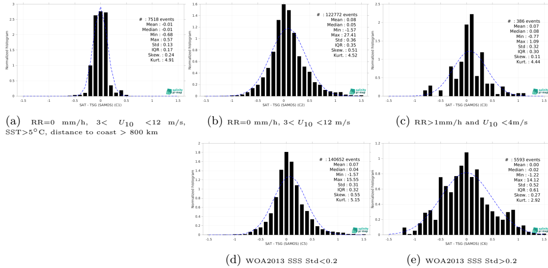
Figure 15: Normalized histogram of \Delta\text{SSS} (CCI SSS L4 POLAR SH Merged-OI v4.41 - 7-day running (ESA) - TSG (SAMOS)) for 5 different subdatasets corresponding to: RR=0 mm/h, 3 < U_{10} < 12 m/s, SST>5°C, distance to coast > 800 km (a), RR=0 mm/h, 3 < U_{10} < 12 m/s (b), RR>1mm/h and U_{10} < 4 m/s (c), WOA2013 SSS Std<0.2 (d), WOA2013 SSS Std>0.2 (e).
