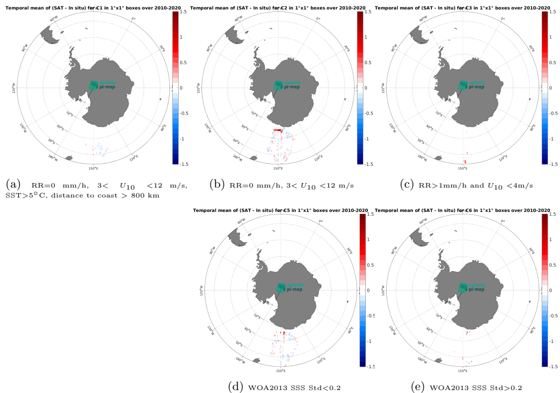
Figure 14: Temporal mean gridded over spatial boxes of size 1^\circ \times 1^\circ of \Delta SSS (CCI SSS L4 POLAR SH Merged-OI v4.41 - 7-day running (ESA) - TSG (LEGOS-Survostral)) for 5 different subdatasets corresponding to:RR=0 mm/h, 3 < U_{10} < 12 m/s, SST > 5^\circ\text{C} , distance to coast > 800 km (a), RR=0 mm/h, 3 < U_{10} < 12 m/s (b), RR > 1 mm/h and U_{10} < 4 m/s (c), WOA2013 SSS Std < 0.2 (d), WOA2013 SSS Std > 0.2 (e).
