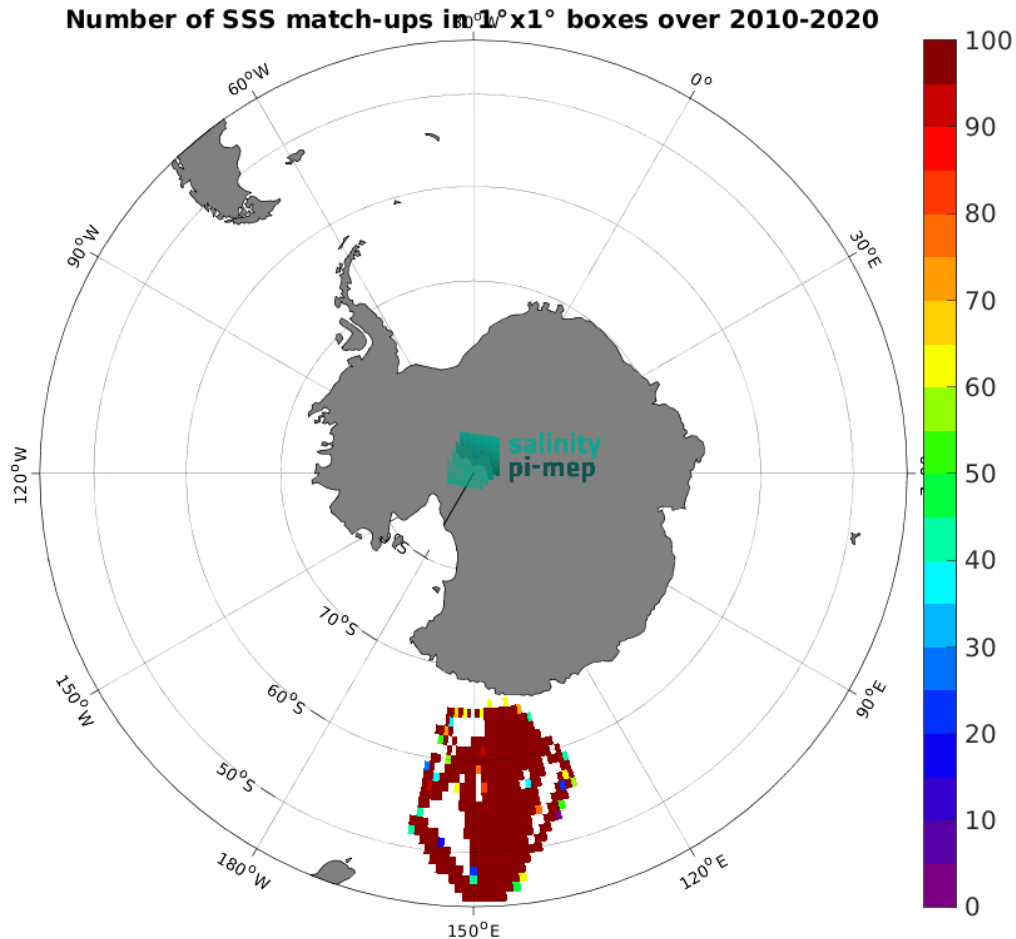
Figure 5: Number of SSS match-ups between TSG (LEGOS-Survostral) SSS and the CCI SSS L4 POLAR SH Merged-OI v4.41 - 7-day running (ESA) SSS product for the Global Ocean Pi-MEP region over 1^\circ \times 1^\circ boxes and for the full satellite product period.
