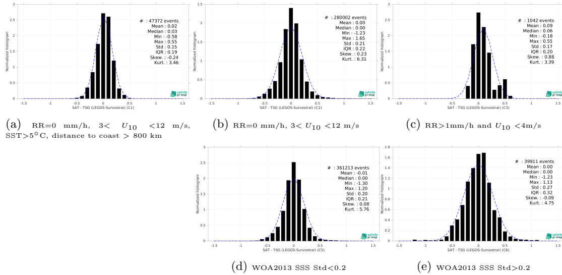
Figure 15: Normalized histogram of \Delta\text{SSS} (CCI SSS L4 POLAR SH Merged-OI v4.41 - 7-day running (ESA) - TSG (LEGOS-Survostral)) for 5 different subdatasets corresponding to: RR=0 mm/h, 3 < U_{10} < 12 m/s, SST>5°C, distance to coast > 800 km (a), RR=0 mm/h, 3 < U_{10} < 12 m/s (b), RR>1mm/h and U_{10} < 4 m/s (c), WOA2013 SSS Std<0.2 (d), WOA2013 SSS Std>0.2 (e).
