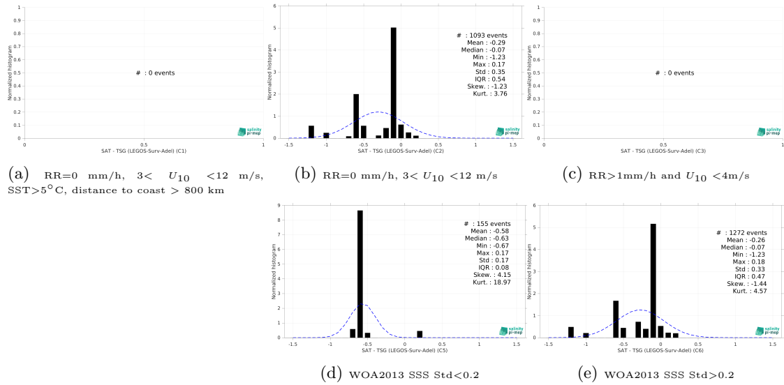
Figure 15: Normalized histogram of \Delta SSS (CCI SSS L4 POLAR SH Merged-OI v4.41 - 7-day running (ESA) - TSG (LEGOS-Surv-Adel)) for 5 different subdatasets corresponding to: RR=0 mm/h, 3 < U_{10} < 12 m/s, SST > 5°C, distance to coast > 800 km (a), RR=0 mm/h, 3 < U_{10} < 12 m/s (b), RR > 1mm/h and U_{10} < 4 m/s (c), WOA2013 SSS Std < 0.2 (d), WOA2013 SSS Std > 0.2 (e).
