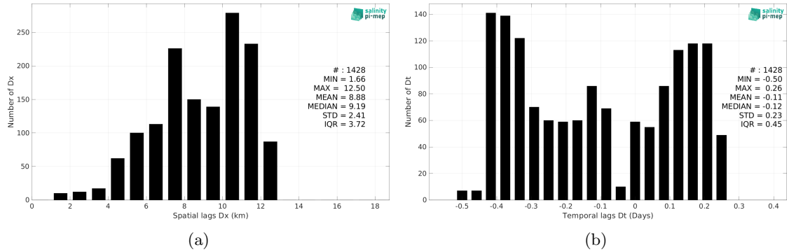
Figure 6: Histograms of the spatial (a) and temporal (b) lags between the location/time of the TSG (LEGOS-Surv-Adel) measurement and the date of the corresponding CCI SSS L4 POLAR SH Merged-OI v4.41 - 7-day running (ESA) SSS pixel.
