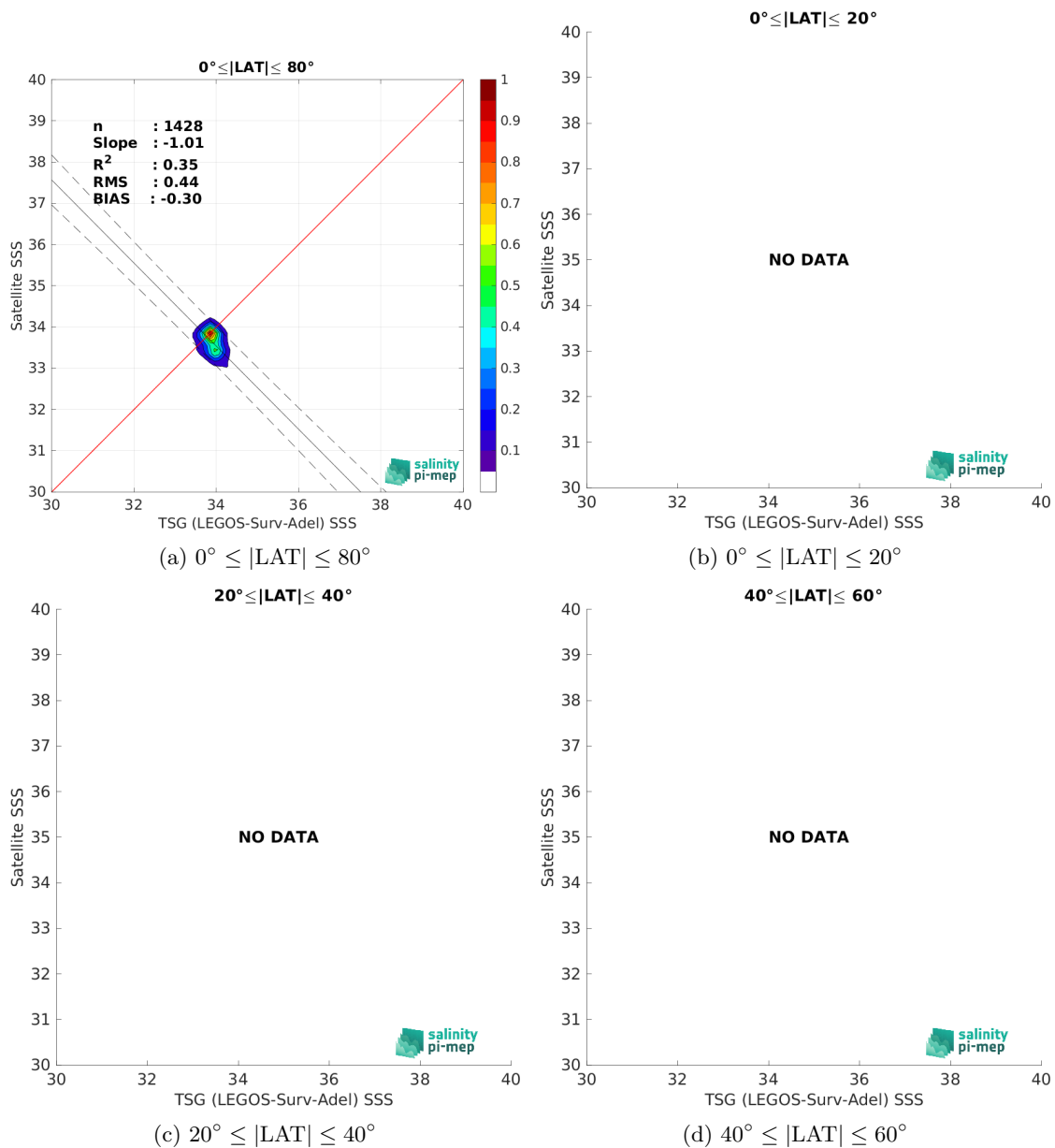
Figure 10: Contour maps of the concentration of CCI SSS L4 POLAR SH Merged-OI v4.41 - 7-day running (ESA) SSS (y-axis) versus TSG (LEGOS-Surv-Adel) SSS (x-axis) at match-up pairs for different latitude bands. For each plot, the red line shows x=y . The black thin and dashed lines indicate a linear fit through the data cloud and the \pm 95\% confidence levels, respectively. The number match-up pairs n , the slope and R^2 coefficient of the linear fit, the root mean square (RMS) and the mean bias between satellite and in situ data are indicated for each latitude band in each plots.
