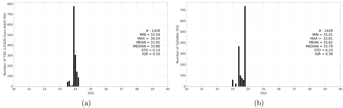
Figure 3: Histograms of SSS from TSG (LEGOS-Surv-Adel) (a) and CCI SSS L4 POLAR SH Merged-OI v4.41 - 7-day running (ESA) (b) considering all match-up pairs per bins of 0.1 over the Global Ocean Pi-MEP region and for the full satellite product period.
