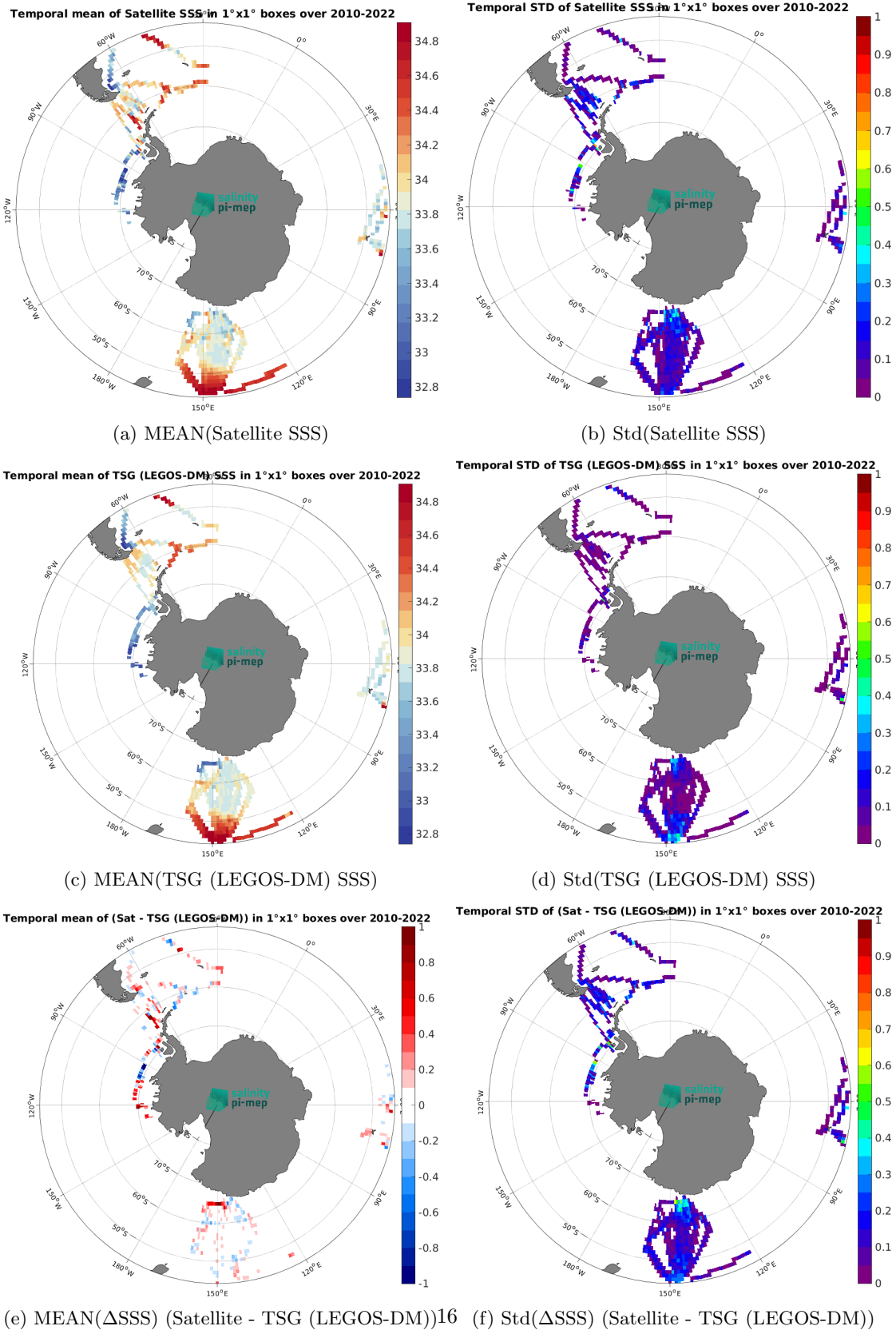
Figure 7: Temporal mean (left) and Std (right) of SSS from CCI SSS L4 POLAR SH Merged-OI v4.41 - 7-day running (ESA) (top), TSG (LEGOS-DM) (middle), and of \Delta SSS (Satellite - TSG (LEGOS-DM)). Only match-up pairs are used to generate these maps.
