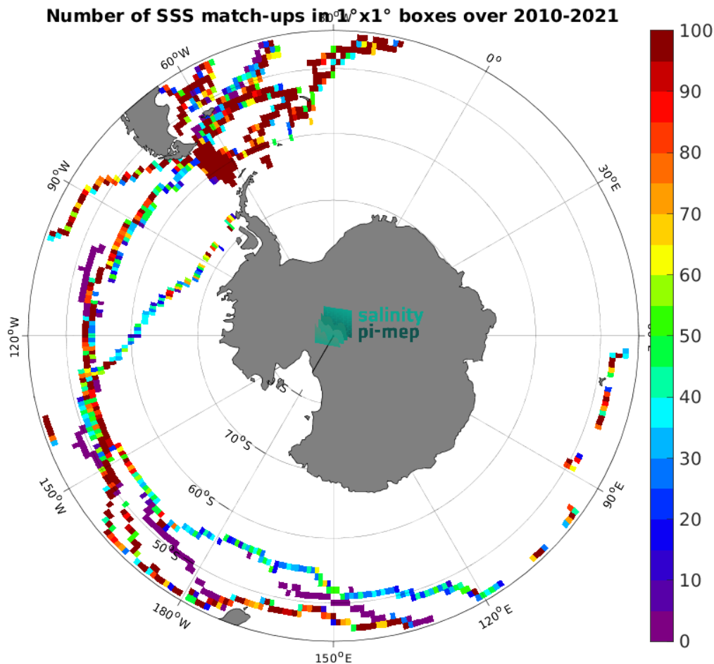
Figure 5: Number of SSS match-ups between TSG (GOSUD-Sailing-ship) SSS and the CCI SSS L4 POLAR SH Merged-OI v4.41 - 7-day running (ESA) SSS product for the Global Ocean Pi-MEP region over 1^\circ \times 1^\circ boxes and for the full satellite product period.
