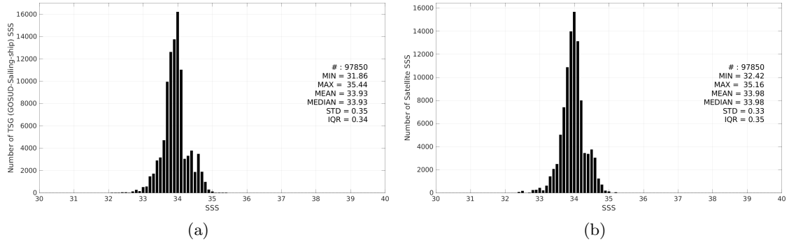
Figure 3: Histograms of SSS from TSG (GOSUD-Sailing-ship) (a) and CCI SSS L4 POLAR SH Merged-OI v4.41 - 7-day running (ESA) (b) considering all match-up pairs per bins of 0.1 over the Global Ocean Pi-MEP region and for the full satellite product period.
