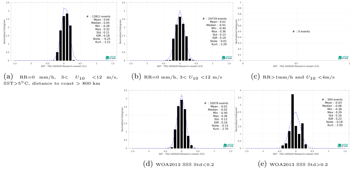
Figure 15: Normalized histogram of \Delta SSS (CCI SSS L4 POLAR SH Merged-OI v4.41 - 7-day running (ESA) - TSG (GOSUD-Research-vessel)) for 5 different subdatasets corresponding to: RR=0 mm/h, 3 < U_{10} < 12 m/s, SST>5°C, distance to coast > 800 km (a), RR=0 mm/h, 3 < U_{10} < 12 m/s (b), RR>1mm/h and U_{10} < 4 m/s (c), WOA2013 SSS Std<0.2 (d), WOA2013 SSS Std>0.2 (e).
