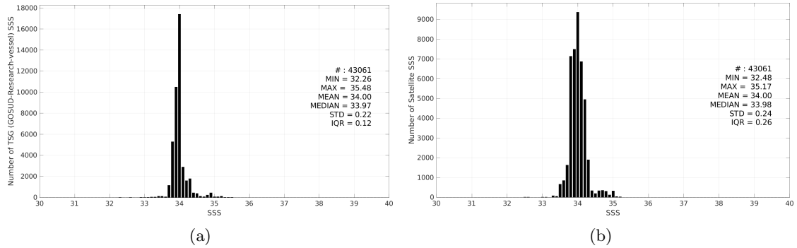
Figure 3: Histograms of SSS from TSG (GOSUD-Research-vessel) (a) and CCI SSS L4 POLAR SH Merged-OI v4.41 - 7-day running (ESA) (b) considering all match-up pairs per bins of 0.1 over the Global Ocean Pi-MEP region and for the full satellite product period.
