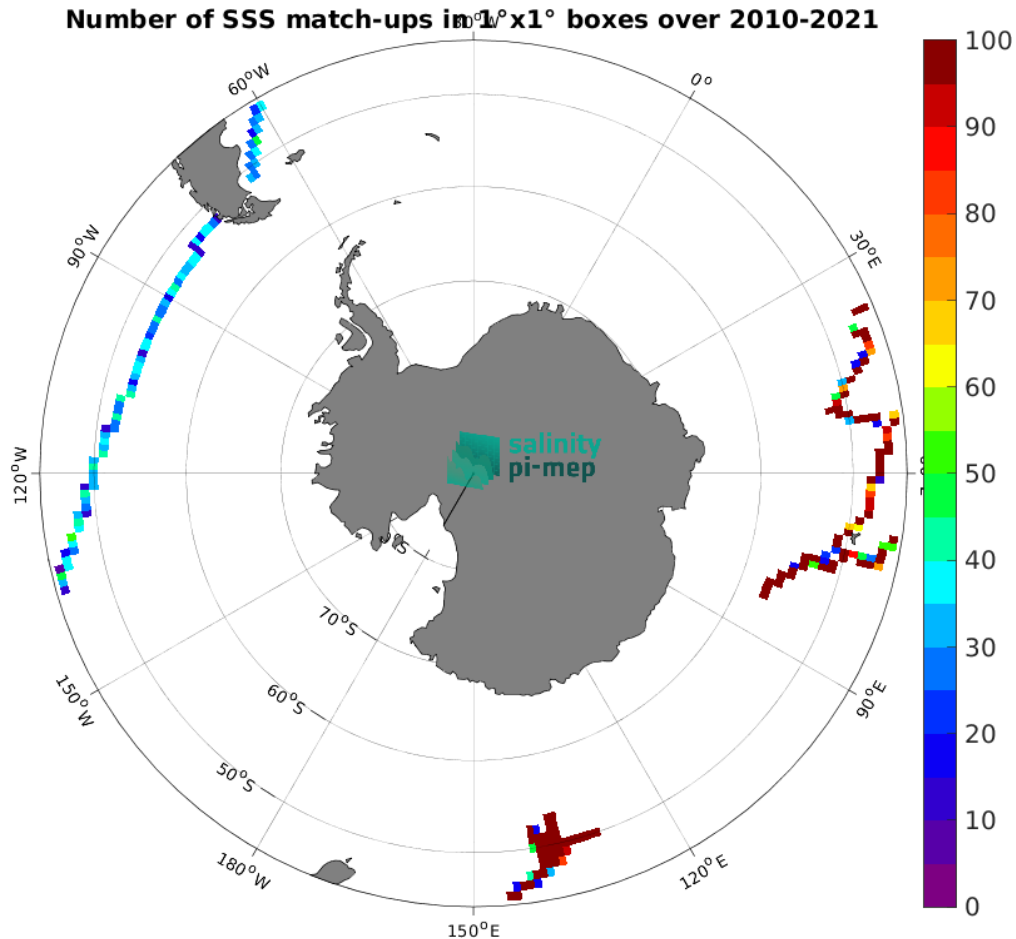
Figure 5: Number of SSS match-ups between TSG (GOSUD-Research-vessel) SSS and the CCI SSS L4 POLAR SH Merged-OI v4.41 - 7-day running (ESA) SSS product for the Global Ocean Pi-MEP region over 1^\circ \times 1^\circ boxes and for the full satellite product period.
