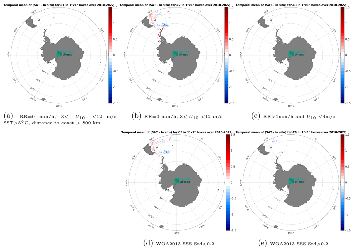
Figure 14: Temporal mean gridded over spatial boxes of size 1^\circ \times 1^\circ of \Delta SSS (CCI SSS L4 POLAR SH Merged-OI v4.41 - 7-day running (ESA) - TSG (CSIC-UTM)) for 5 different subdatasets corresponding to:RR=0 mm/h, 3 < U_{10} < 12 m/s, SST >5^\circ\text{C} , distance to coast > 800 km (a), RR=0 mm/h, 3 < U_{10} < 12 m/s (b), RR >1 mm/h and U_{10} < 4 m/s (c), WOA2013 SSS Std <0.2 (d), WOA2013 SSS Std >0.2 (e).
