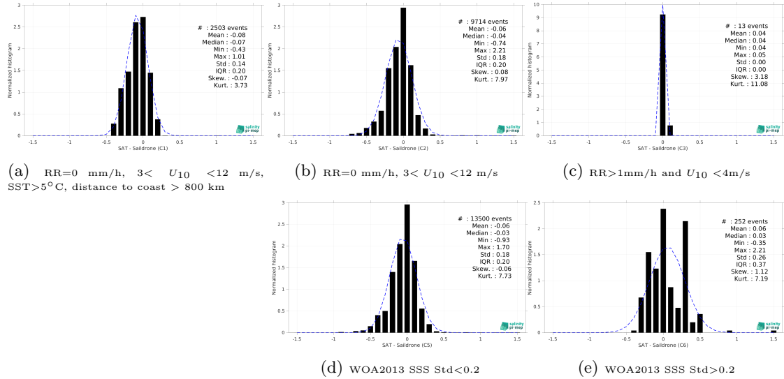
Figure 15: Normalized histogram of \Delta\text{SSS} (CCI SSS L4 POLAR SH Merged-OI v4.41 - 7-day running (ESA) - Saldrone) for 5 different subdatasets corresponding to: RR=0 mm/h, 3 < U_{10} < 12 m/s, SST > 5^\circ\text{C} , distance to coast > 800 km (a), RR=0 mm/h, 3 < U_{10} < 12 m/s (b), RR > 1\text{mm/h} and U_{10} < 4\text{m/s} (c), WOA2013 SSS Std < 0.2 (d), WOA2013 SSS Std > 0.2 (e).
