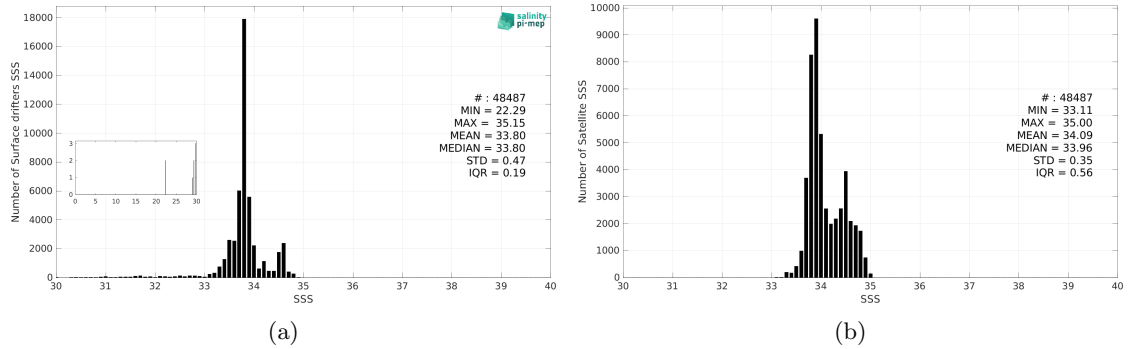
Figure 3: Histograms of SSS from Surface drifters (a) and CCI SSS L4 POLAR SH Merged-OI v4.41 - 7-day running (ESA) (b) considering all match-up pairs per bins of 0.1 over the Global Ocean Pi-MEP region and for the full satellite product period.
