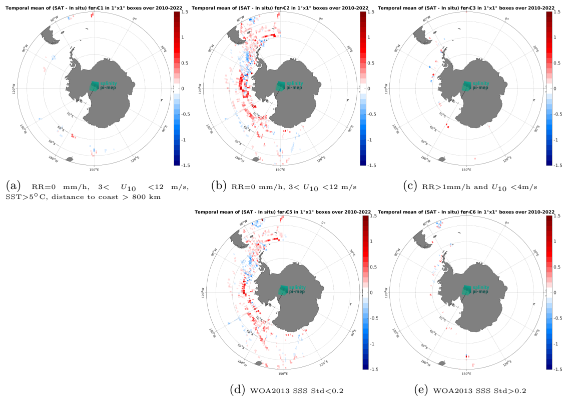
Figure 14: Temporal mean gridded over spatial boxes of size 1^\circ \times 1^\circ of \Delta SSS (CCI SSS L4 POLAR SH Merged-OI v4.41 - 30-day running (ESA) - TSG (SAMOS)) for 5 different subdatasets corresponding to:RR=0 mm/h, 3 < U_{10} < 12 m/s, SST >5^\circ\text{C} , distance to coast > 800 km (a), RR=0 mm/h, 3 < U_{10} < 12 m/s (b), RR >1 mm/h and U_{10} < 4 m/s (c), WOA2013 SSS Std <0.2 (d), WOA2013 SSS Std >0.2 (e).
