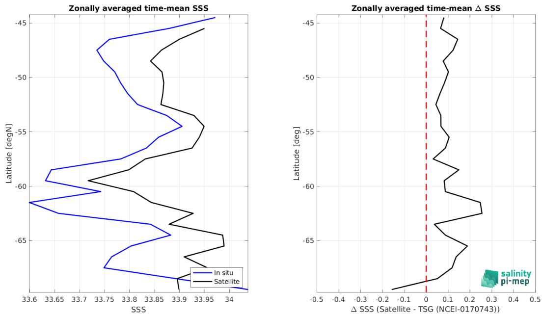
Figure 9: Left panel: Zonal mean SSS from CCI SSS L4 POLAR SH Merged-OI v4.41 - 30-day running (ESA) satellite product (black) and from TSG (NCEI-0170743) (blue). Right panel: Zonal mean of \Delta SSS (Satellite - TSG (NCEI-0170743)) for all the collected Pi-MEP match-up pairs estimated over the full satellite product period.
