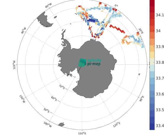
(c) MEAN(TSG (NCEI-0170743) SSS)
