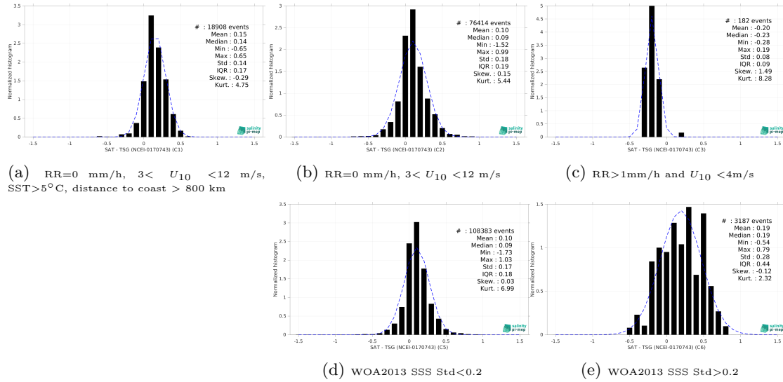
Figure 15: Normalized histogram of \Delta SSS (CCI SSS L4 POLAR SH Merged-OI v4.41 - 30-day running (ESA) - TSG (NCEI-0170743)) for 5 different subdatasets corresponding to: RR=0 mm/h, 3 < U_{10} < 12 m/s, SST>5°C, distance to coast > 800 km (a), RR=0 mm/h, 3 < U_{10} < 12 m/s (b), RR>1mm/h and U_{10} < 4 m/s (c), WOA2013 SSS Std<0.2 (d), WOA2013 SSS Std>0.2 (e).
