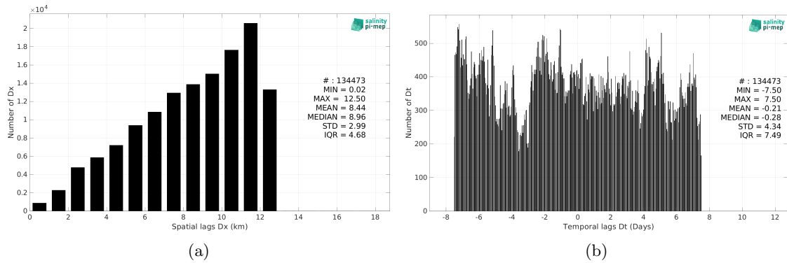
Figure 6: Histograms of the spatial (a) and temporal (b) lags between the location/time of the TSG (NCEI-0170743) measurement and the date of the corresponding CCI SSS L4 POLAR SH Merged-OI v4.41 - 30-day running (ESA) SSS pixel.
