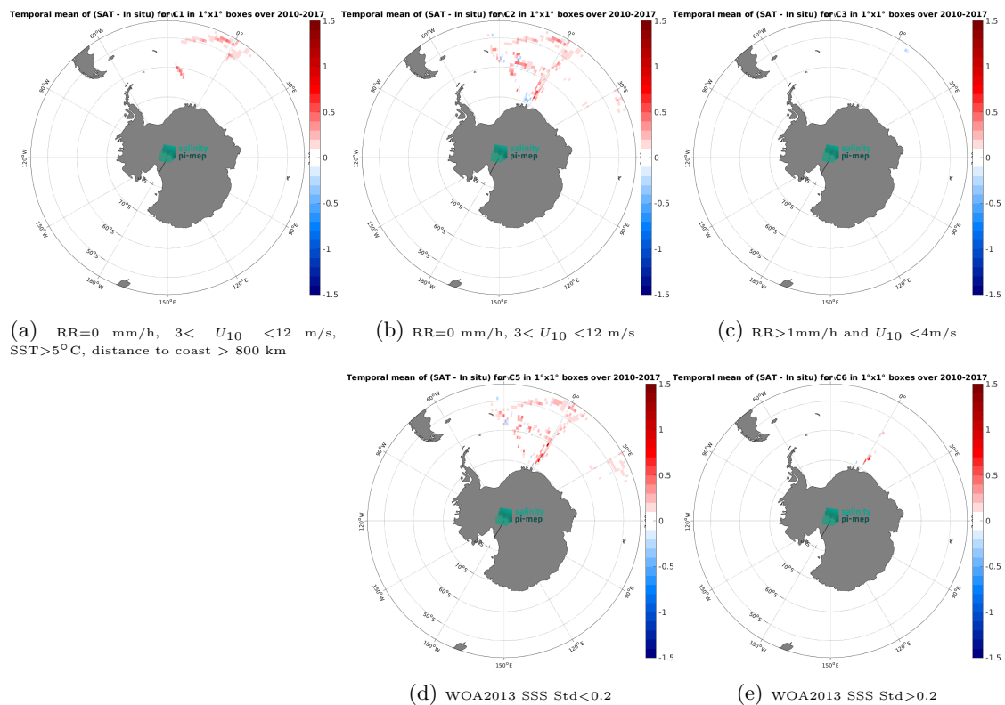
Figure 14: Temporal mean gridded over spatial boxes of size 1^\circ \times 1^\circ of \Delta SSS (CCI SSS L4 POLAR SH Merged-OI v4.41 - 30-day running (ESA) - TSG (NCEI-0170743)) for 5 different subdatasets corresponding to:RR=0 mm/h, 3 < U_{10} < 12 m/s, SST >5^\circ C, distance to coast > 800 km (a), RR=0 mm/h, 3 < U_{10} < 12 m/s (b), RR >1 mm/h and U_{10} < 4 m/s (c), WOA2013 SSS Std <0.2 (d), WOA2013 SSS Std >0.2 (e).
