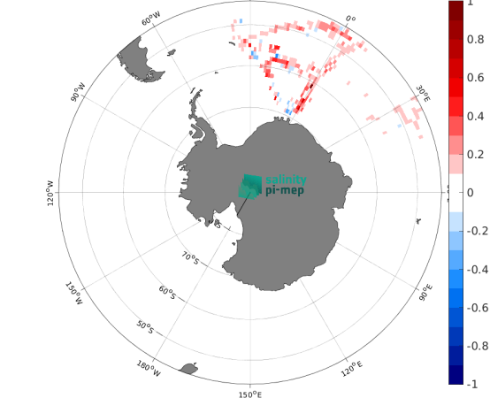
(e) MEAN( \Delta SSS) (Satellite - TSG (NCEI-0170743))
