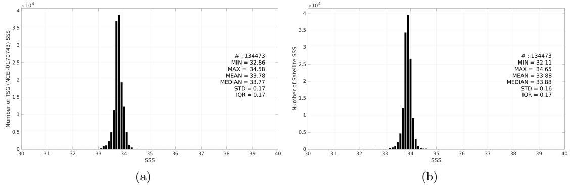
Figure 3: Histograms of SSS from TSG (NCEI-0170743) (a) and CCI SSS L4 POLAR SH Merged-OI v4.41 - 30-day running (ESA) (b) considering all match-up pairs per bins of 0.1 over the Global Ocean Pi-MEP region and for the full satellite product period.
