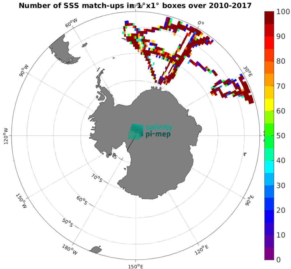
Figure 5: Number of SSS match-ups between TSG (NCEI-0170743) SSS and the CCI SSS L4 POLAR SH Merged-OI v4.41 - 30-day running (ESA) SSS product for the Global Ocean Pi-MEP region over 1^\circ \times 1^\circ boxes and for the full satellite product period.
