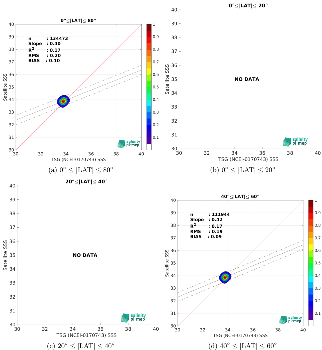
Figure 10: Contour maps of the concentration of CCI SSS L4 POLAR SH Merged-OI v4.41 - 30-day running (ESA) SSS (y-axis) versus TSG (NCEI-0170743) SSS (x-axis) at match-up pairs for different latitude bands. For each plot, the red line shows x=y . The black thin and dashed lines indicate a linear fit through the data cloud and the \pm 95\% confidence levels, respectively. The number match-up pairs n , the slope and R^2 coefficient of the linear fit, the root mean square (RMS) and the mean bias between satellite and in situ data are indicated for each latitude band in each plots.
