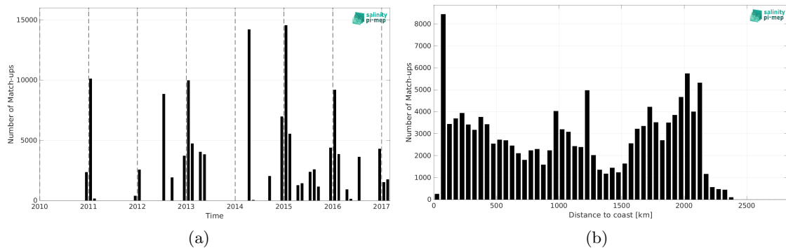
Figure 2: Number of match-ups between TSG (NCEI-0170743) and CCI SSS L4 POLAR SH Merged-OI v4.41 - 30-day running (ESA) SSS as a function of time (a) and as function of the distance to coast (b) over the Global Ocean Pi-MEP region and for the full satellite product period.
