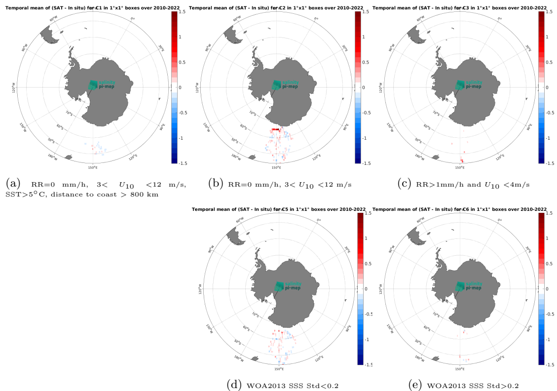
Figure 14: Temporal mean gridded over spatial boxes of size 1^\circ \times 1^\circ of \Delta SSS (CCI SSS L4 POLAR SH Merged-OI v4.41 - 30-day running (ESA) - TSG (LEGOS-Survostral)) for 5 different subdatasets corresponding to:RR=0 mm/h, 3 < U_{10} < 12 m/s, SST>5°C, distance to coast > 800 km (a), RR=0 mm/h, 3 < U_{10} < 12 m/s (b), RR>1mm/h and U_{10} < 4 m/s (c), WOA2013 SSS Std<0.2 (d), WOA2013 SSS Std>0.2 (e).
