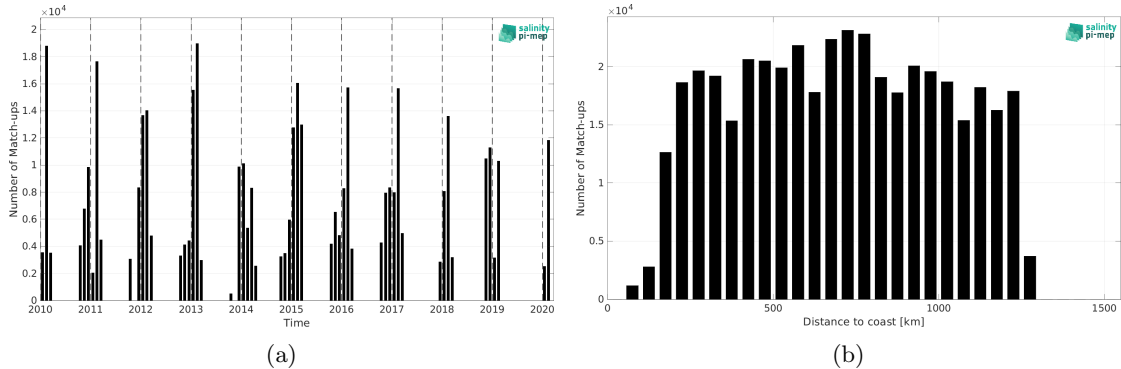
Figure 2: Number of match-ups between TSG (LEGOS-Survostral) and CCI SSS L4 POLAR SH Merged-OI v4.41 - 30-day running (ESA) SSS as a function of time (a) and as function of the distance to coast (b) over the Global Ocean Pi-MEP region and for the full satellite product period.
