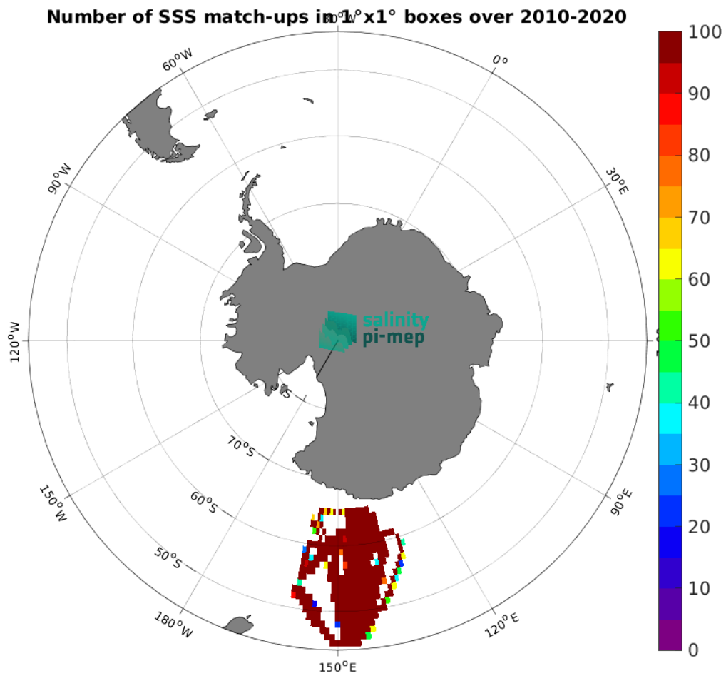
Figure 5: Number of SSS match-ups between TSG (LEGOS-Survostral) SSS and the CCI SSS L4 POLAR SH Merged-OI v4.41 - 30-day running (ESA) SSS product for the Global Ocean Pi-MEP region over 1^\circ \times 1^\circ boxes and for the full satellite product period.
