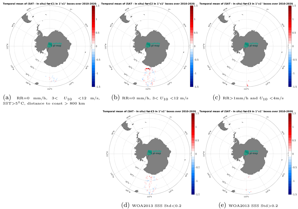
Figure 14: Temporal mean gridded over spatial boxes of size 1^\circ \times 1^\circ of \Delta\text{SSS} (CCI SSS L4 POLAR SH Merged-OI v4.41 - 30-day running (ESA) - TSG (LEGOS-Survostral)) for 5 different subdatasets corresponding to:RR=0 mm/h, 3 < U_{10} < 12 m/s, SST >5^\circ\text{C} , distance to coast > 800 km (a), RR=0 mm/h, 3 < U_{10} < 12 m/s (b), RR >1 mm/h and U_{10} < 4 m/s (c), WOA2013 SSS Std <0.2 (d), WOA2013 SSS Std >0.2 (e).
