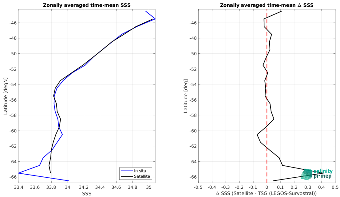
Figure 9: Left panel: Zonal mean SSS from CCI SSS L4 POLAR SH Merged-OI v4.41 - 30-day running (ESA) satellite product (black) and from TSG (LEGOS-Survostral) (blue). Right panel: Zonal mean of \Delta SSS (Satellite - TSG (LEGOS-Survostral)) for all the collected Pi-MEP match-up pairs estimated over the full satellite product period.
