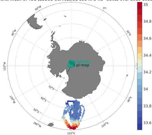
(c) MEAN(TSG (LEGOS-Survostral) SSS)
