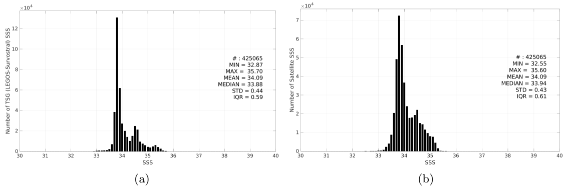
Figure 3: Histograms of SSS from TSG (LEGOS-Survostral) (a) and CCI SSS L4 POLAR SH Merged-OI v4.41 - 30-day running (ESA) (b) considering all match-up pairs per bins of 0.1 over the Global Ocean Pi-MEP region and for the full satellite product period.
