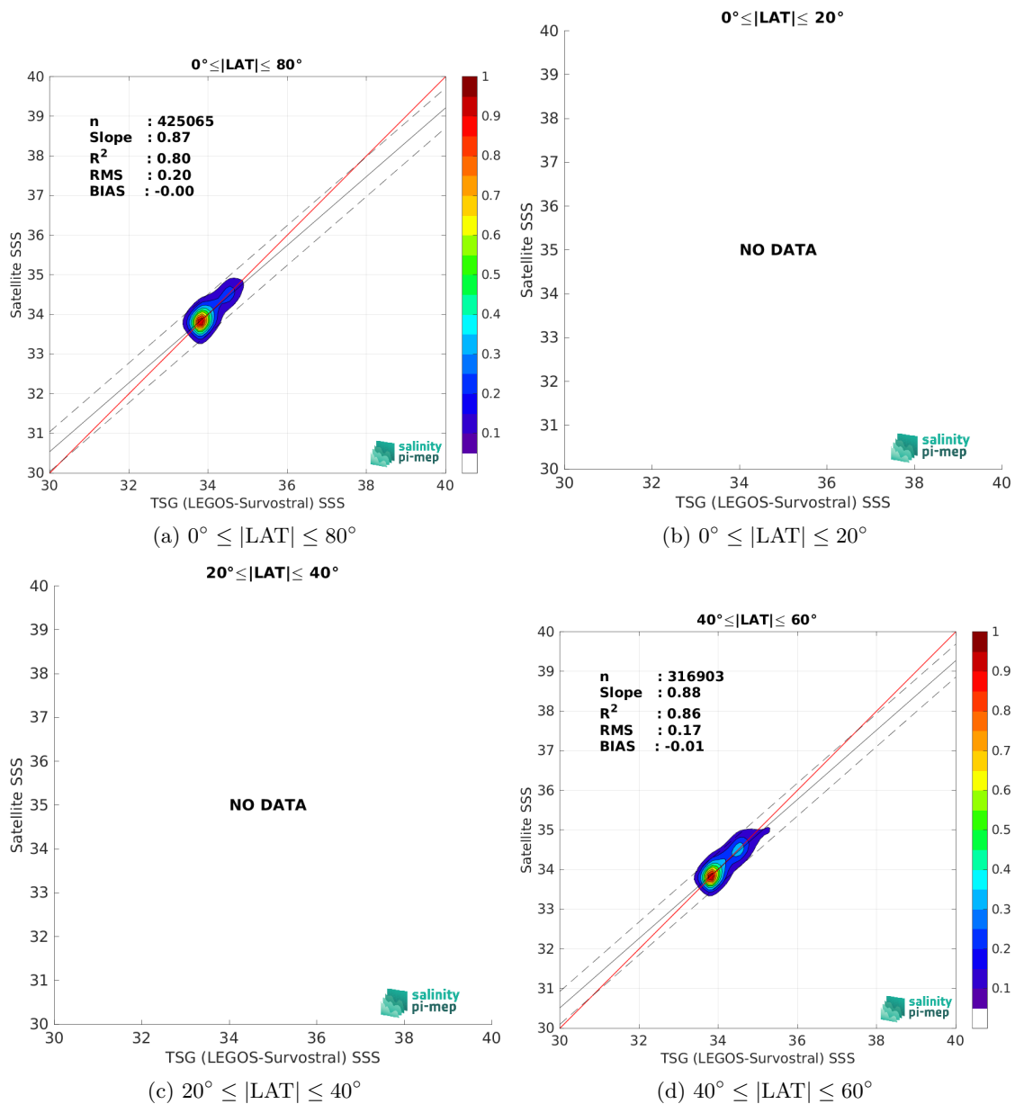
Figure 10: Contour maps of the concentration of CCI SSS L4 POLAR SH Merged-OI v4.41 - 30-day running (ESA) SSS (y-axis) versus TSG (LEGOS-Survostral) SSS (x-axis) at match-up pairs for different latitude bands. For each plot, the red line shows x=y . The black thin and dashed lines indicate a linear fit through the data cloud and the \pm 95\% confidence levels, respectively. The number match-up pairs n , the slope and R^2 coefficient of the linear fit, the root mean square (RMS) and the mean bias between satellite and in situ data are indicated for each latitude band in each plots.
