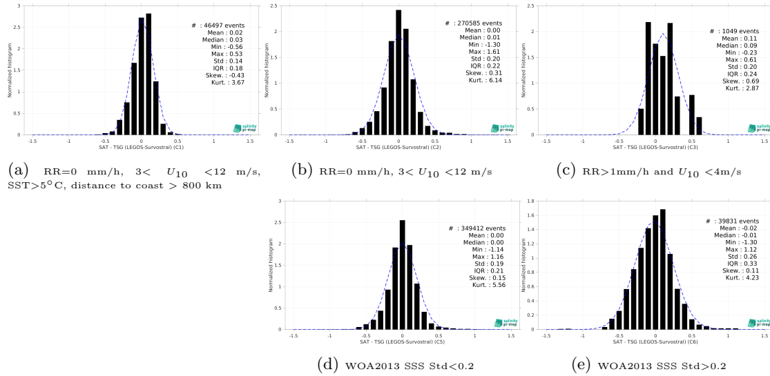
Figure 15: Normalized histogram of \Delta SSS (CCI SSS L4 POLAR SH Merged-OI v4.41 - 30-day running (ESA) - TSG (LEGOS-Survostral)) for 5 different subdatasets corresponding to: RR=0 mm/h, 3 < U_{10} < 12 m/s, SST>5°C, distance to coast > 800 km (a), RR=0 mm/h, 3 < U_{10} < 12 m/s (b), RR>1mm/h and U_{10} < 4 m/s (c), WOA2013 SSS Std<0.2 (d), WOA2013 SSS Std>0.2 (e).
