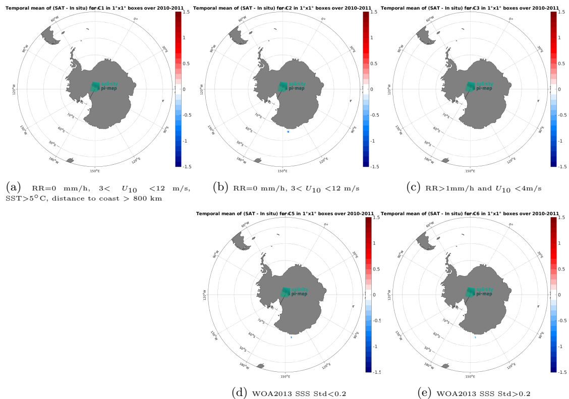
Figure 14: Temporal mean gridded over spatial boxes of size 1^\circ \times 1^\circ of \Delta SSS (CCI SSS L4 POLAR SH Merged-OI v4.41 - 30-day running (ESA) - TSG (LEGOS-Surv-Adel)) for 5 different subdatasets corresponding to: RR=0 mm/h, 3 < U_{10} < 12 m/s, SST > 5^\circ\text{C} , distance to coast > 800 km (a), RR=0 mm/h, 3 < U_{10} < 12 m/s (b), RR > 1 mm/h and U_{10} < 4 m/s (c), WOA2013 SSS Std < 0.2 (d), WOA2013 SSS Std > 0.2 (e).
