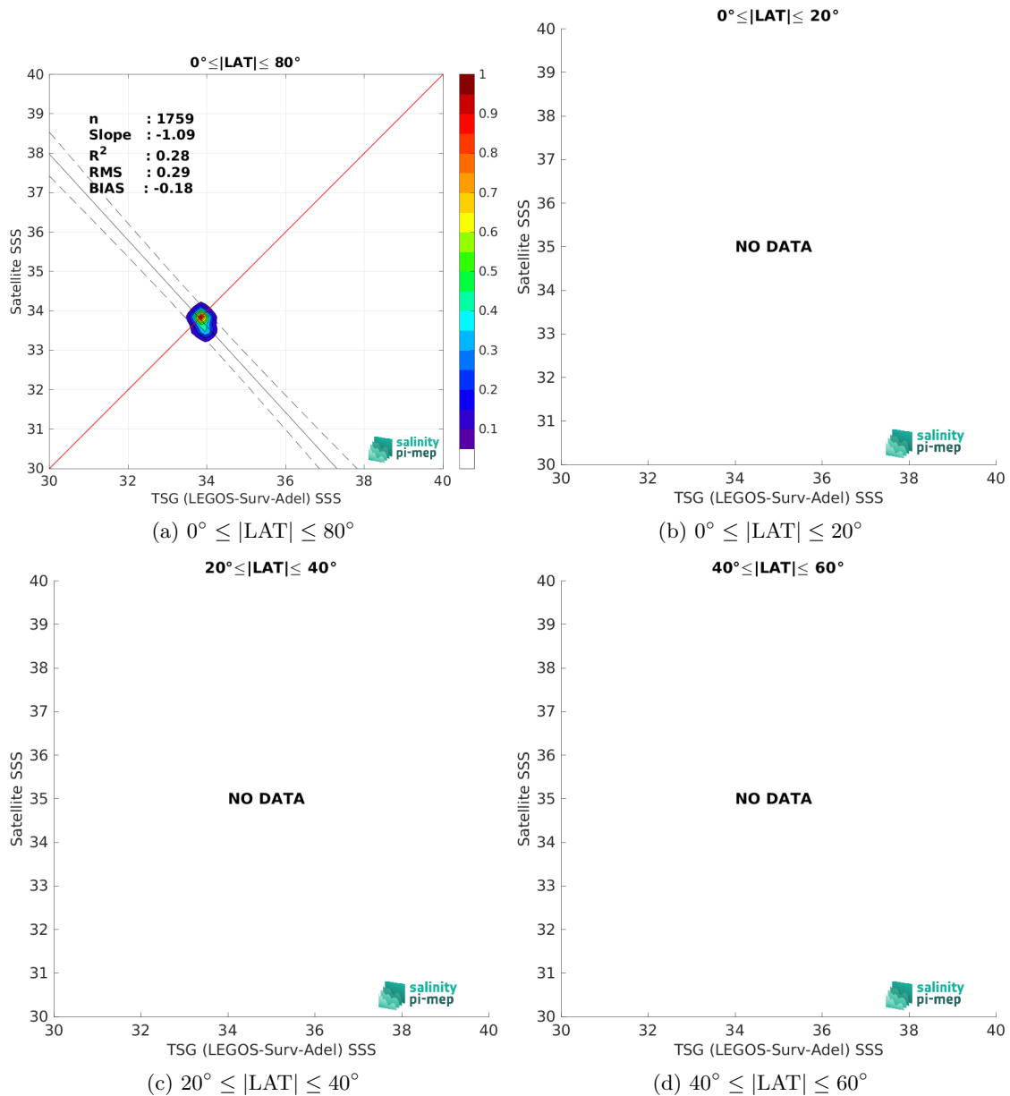
Figure 10: Contour maps of the concentration of CCI SSS L4 POLAR SH Merged-OI v4.41 - 30-day running (ESA) SSS (y-axis) versus TSG (LEGOS-Surv-Adel) SSS (x-axis) at match-up pairs for different latitude bands. For each plot, the red line shows x=y . The black thin and dashed lines indicate a linear fit through the data cloud and the \pm 95\% confidence levels, respectively. The number match-up pairs n , the slope and R^2 coefficient of the linear fit, the root mean square (RMS) and the mean bias between satellite and in situ data are indicated for each latitude band in each plots.
