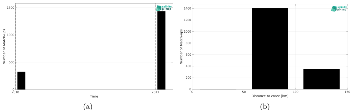
Figure 2: Number of match-ups between TSG (LEGOS-Surv-Adel) and CCI SSS L4 POLAR SH Merged-OI v4.41 - 30-day running (ESA) SSS as a function of time (a) and as function of the distance to coast (b) over the Global Ocean Pi-MEP region and for the full satellite product period.
