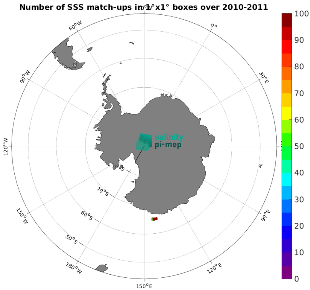
Figure 5: Number of SSS match-ups between TSG (LEGOS-Surv-Adel) SSS and the CCI SSS L4 POLAR SH Merged-OI v4.41 - 30-day running (ESA) SSS product for the Global Ocean Pi-MEP region over 1^\circ \times 1^\circ boxes and for the full satellite product period.
