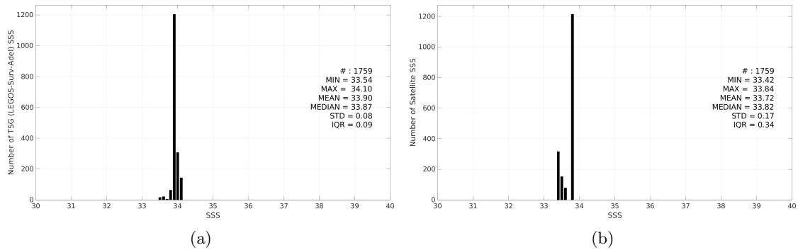
Figure 3: Histograms of SSS from TSG (LEGOS-Surv-Adel) (a) and CCI SSS L4 POLAR SH Merged-OI v4.41 - 30-day running (ESA) (b) considering all match-up pairs per bins of 0.1 over the Global Ocean Pi-MEP region and for the full satellite product period.
