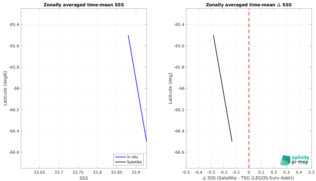
Figure 9: Left panel: Zonal mean SSS from CCI SSS L4 POLAR SH Merged-OI v4.41 - 30-day running (ESA) satellite product (black) and from TSG (LEGOS-Surv-Adel) (blue). Right panel: Zonal mean of \Delta SSS (Satellite - TSG (LEGOS-Surv-Adel)) for all the collected Pi-MEP match-up pairs estimated over the full satellite product period.
