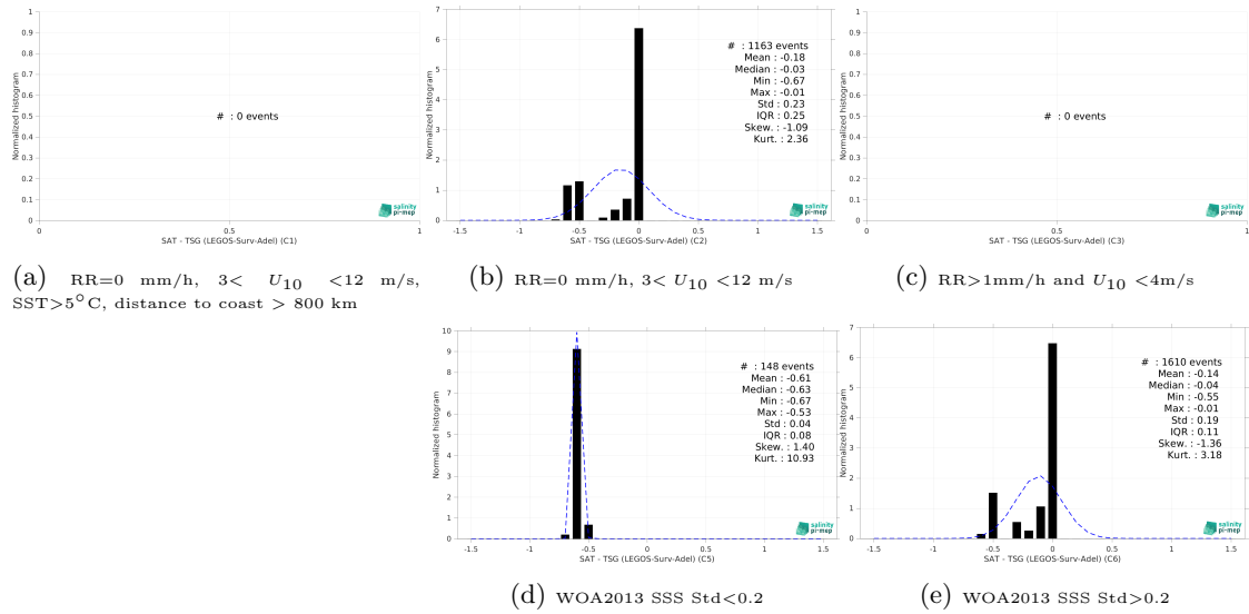
Figure 15: Normalized histogram of \Delta\text{SSS} (CCI SSS L4 POLAR SH Merged-OI v4.41 - 30-day running (ESA) - TSG (LEGOS-Surv-Adel)) for 5 different subdatasets corresponding to: RR=0 mm/h, 3 < U_{10} < 12 m/s, SST>5°C, distance to coast > 800 km (a), RR=0 mm/h, 3 < U_{10} < 12 m/s (b), RR>1mm/h and U_{10} < 4 m/s (c), WOA2013 SSS Std<0.2 (d), WOA2013 SSS Std>0.2 (e).
