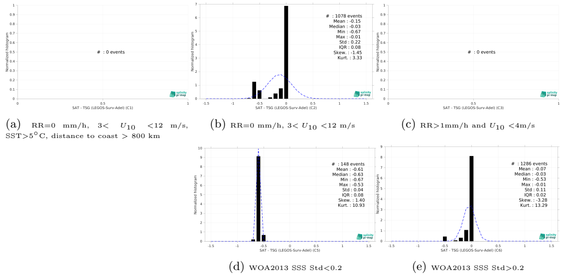
Figure 15: Normalized histogram of \Delta SSS (CCI SSS L4 POLAR SH Merged-OI v4.41 - 30-day running (ESA) - TSG (LEGOS-Surv-Adel)) for 5 different subdatasets corresponding to: RR=0 mm/h, 3 < U_{10} < 12 m/s, SST > 5°C, distance to coast > 800 km (a), RR=0 mm/h, 3 < U_{10} < 12 m/s (b), RR > 1mm/h and U_{10} < 4 m/s (c), WOA2013 SSS Std < 0.2 (d), WOA2013 SSS Std > 0.2 (e).
