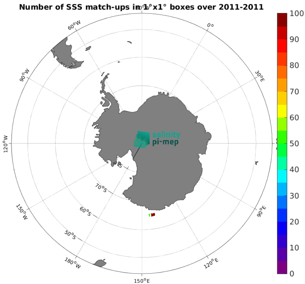
Figure 5: Number of SSS match-ups between TSG (LEGOS-Surv-Adel) SSS and the CCI SSS L4 POLAR SH Merged-OI v4.41 - 30-day running (ESA) SSS product for the Global Ocean Pi-MEP region over 1^{\circ} \times 1^{\circ} boxes and for the full satellite product period.
