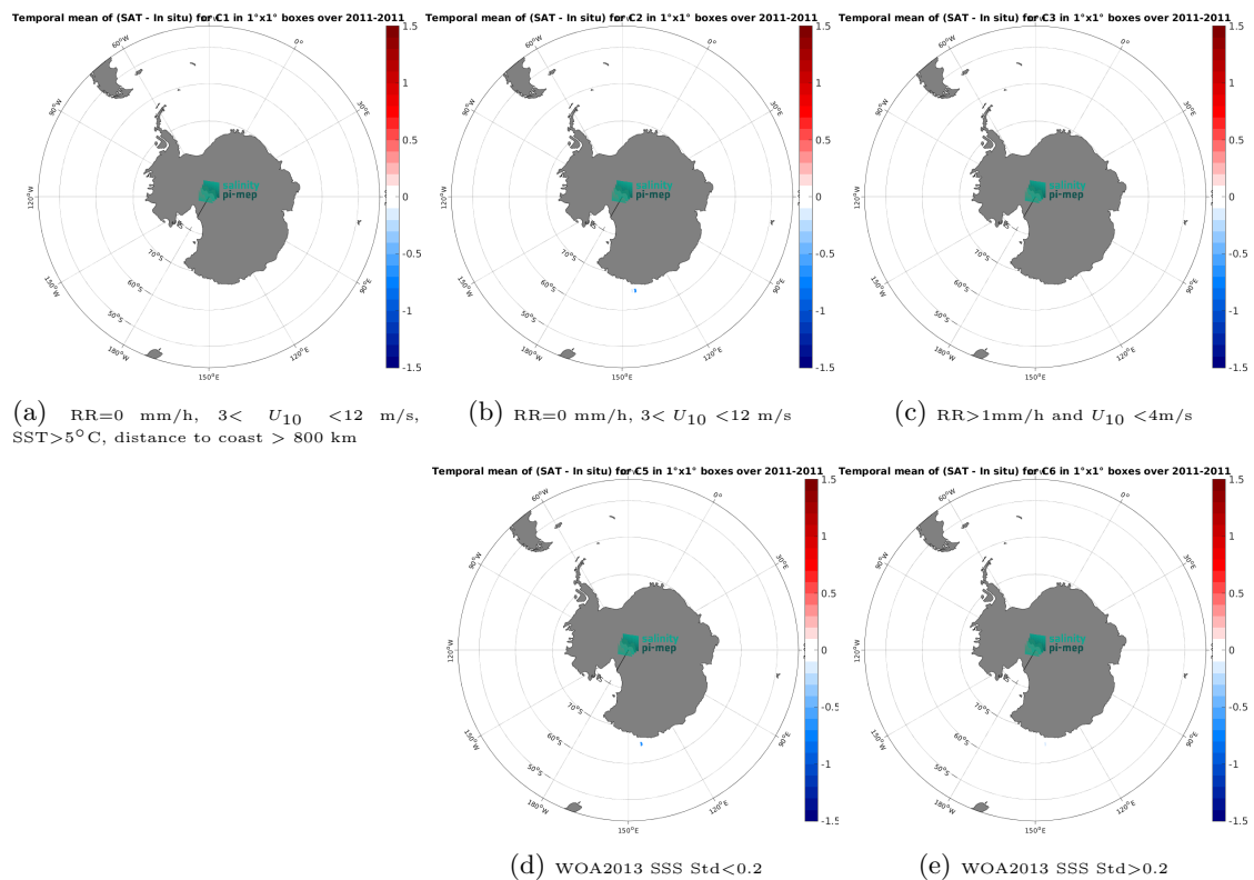
Figure 14: Temporal mean gridded over spatial boxes of size 1^\circ \times 1^\circ of \Delta\text{SSS} (CCI SSS L4 POLAR SH Merged-OI v4.41 - 30-day running (ESA) - TSG (LEGOS-Surv-Adel)) for 5 different subdatasets corresponding to:RR=0 mm/h, 3 < U_{10} < 12 m/s, SST >5^\circ\text{C} , distance to coast > 800 km (a), RR=0 mm/h, 3 < U_{10} < 12 m/s (b), RR >1 mm/h and U_{10} < 4 m/s (c), WOA2013 SSS Std <0.2 (d), WOA2013 SSS Std >0.2 (e).
