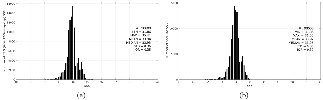
Figure 3: Histograms of SSS from TSG (GOSUD-Sailing-ship) (a) and CCI SSS L4 POLAR SH Merged-OI v4.41 - 30-day running (ESA) (b) considering all match-up pairs per bins of 0.1 over the Global Ocean Pi-MEP region and for the full satellite product period.
