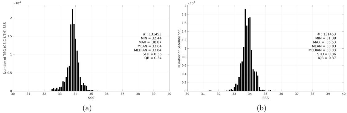
Figure 3: Histograms of SSS from TSG (CSIC-UTM) (a) and CCI SSS L4 POLAR SH Merged-OI v4.41 - 30-day running (ESA) (b) considering all match-up pairs per bins of 0.1 over the Global Ocean Pi-MEP region and for the full satellite product period.
