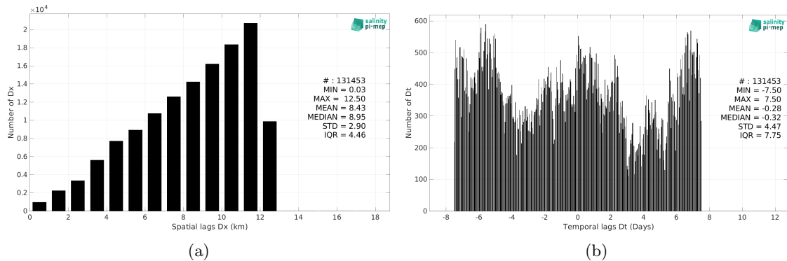
Figure 6: Histograms of the spatial (a) and temporal (b) lags between the location/time of the TSG (CSIC-UTM) measurement and the date of the corresponding CCI SSS L4 POLAR SH Merged-OI v4.41 - 30-day running (ESA) SSS pixel.
