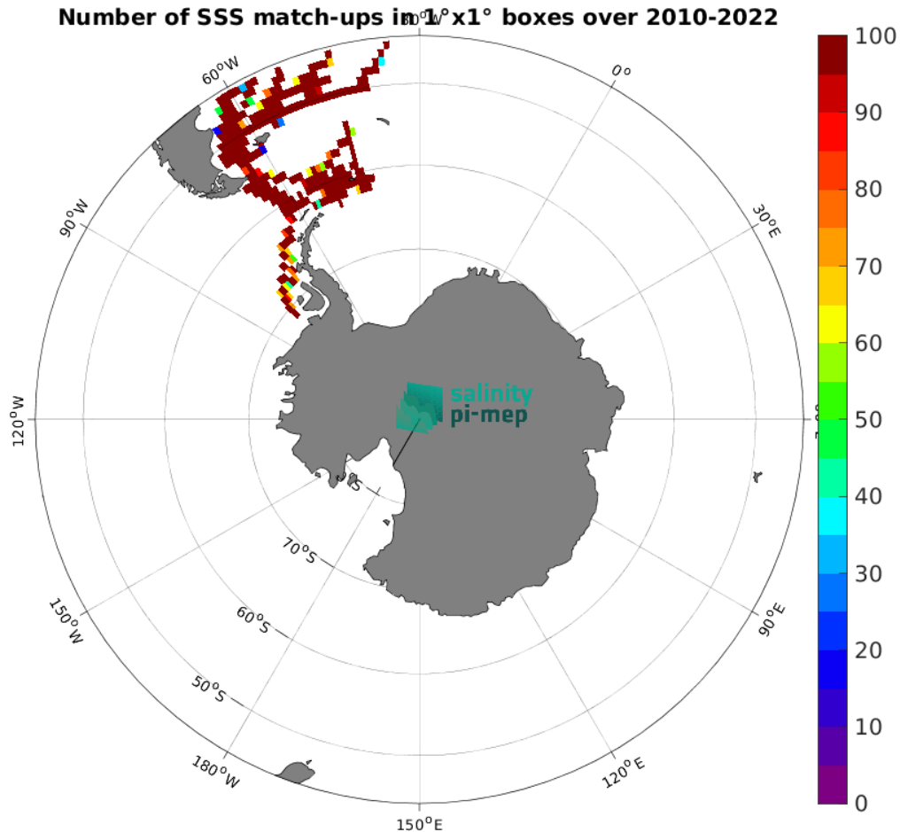
Figure 5: Number of SSS match-ups between TSG (CSIC-UTM) SSS and the CCI SSS L4 POLAR SH Merged-OI v4.41 - 30-day running (ESA) SSS product for the Global Ocean Pi-MEP region over 1^\circ \times 1^\circ boxes and for the full satellite product period.
