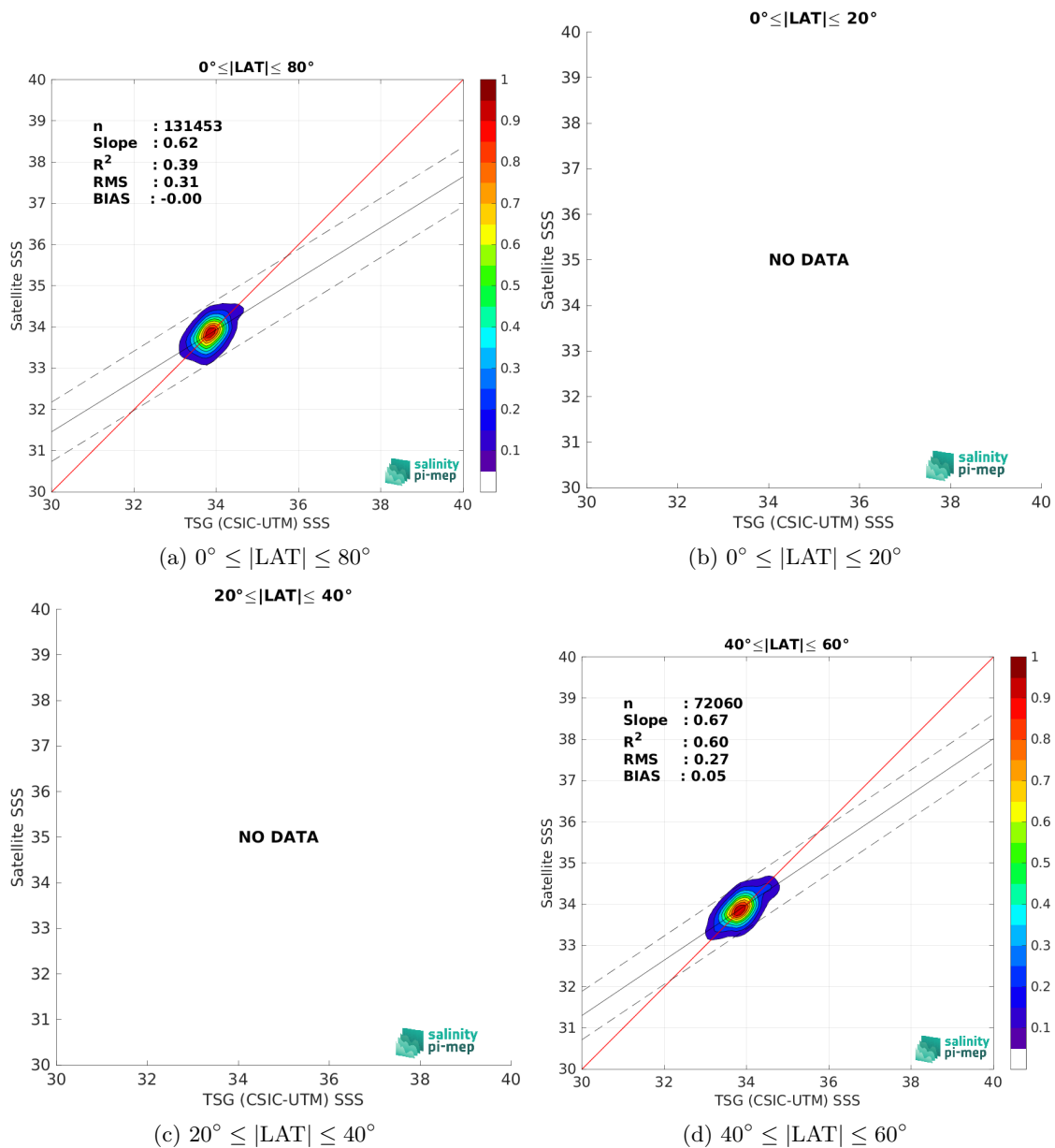
Figure 10: Contour maps of the concentration of CCI SSS L4 POLAR SH Merged-OI v4.41 - 30-day running (ESA) SSS (y-axis) versus TSG (CSIC-UTM) SSS (x-axis) at match-up pairs for different latitude bands. For each plot, the red line shows x=y . The black thin and dashed lines indicate a linear fit through the data cloud and the \pm 95\% confidence levels, respectively. The number match-up pairs n , the slope and R^2 coefficient of the linear fit, the root mean square (RMS) and the mean bias between satellite and in situ data are indicated for each latitude band in each plots.
