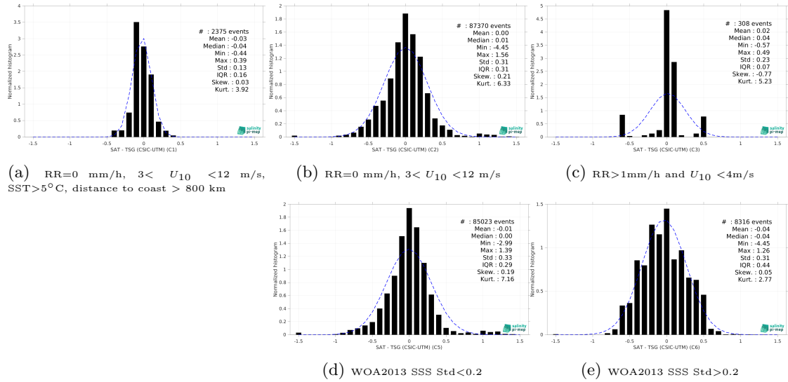
Figure 15: Normalized histogram of \Delta SSS (CCI SSS L4 POLAR SH Merged-OI v4.41 - 30-day running (ESA) - TSG (CSIC-UTM)) for 5 different subdatasets corresponding to: RR=0 mm/h, 3 < U_{10} < 12 m/s, SST>5°C, distance to coast > 800 km (a), RR=0 mm/h, 3 < U_{10} < 12 m/s (b), RR>1mm/h and U_{10} < 4 m/s (c), WOA2013 SSS Std<0.2 (d), WOA2013 SSS Std>0.2 (e).
