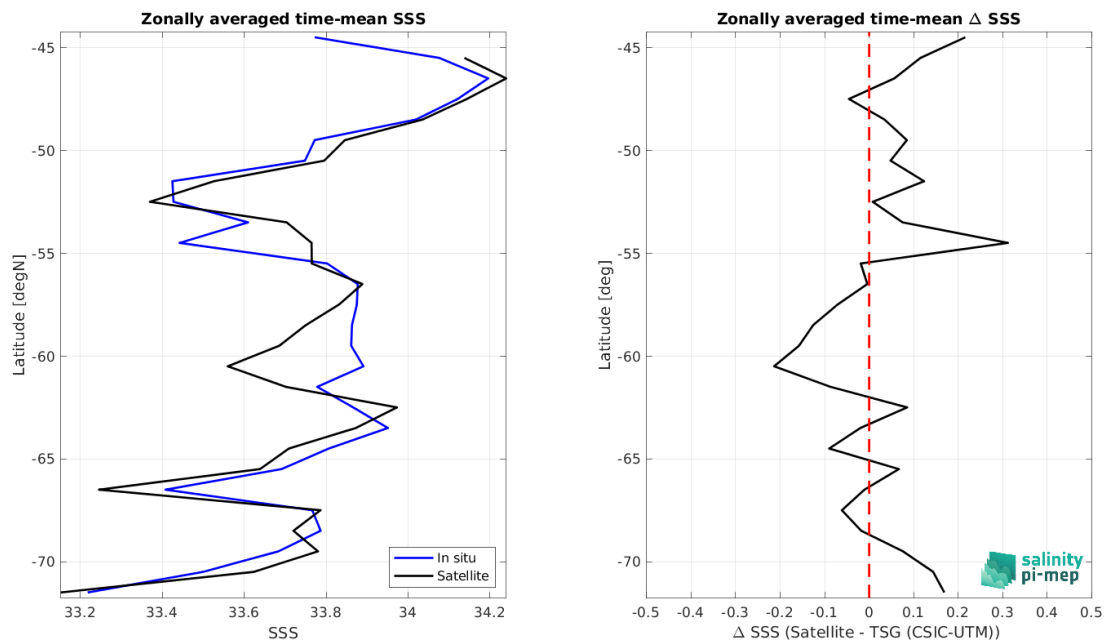
Figure 9: Left panel: Zonal mean SSS from CCI SSS L4 POLAR SH Merged-OI v4.41 - 30-day running (ESA) satellite product (black) and from TSG (CSIC-UTM) (blue). Right panel: Zonal mean of \Delta SSS (Satellite - TSG (CSIC-UTM)) for all the collected Pi-MEP match-up pairs estimated over the full satellite product period.
