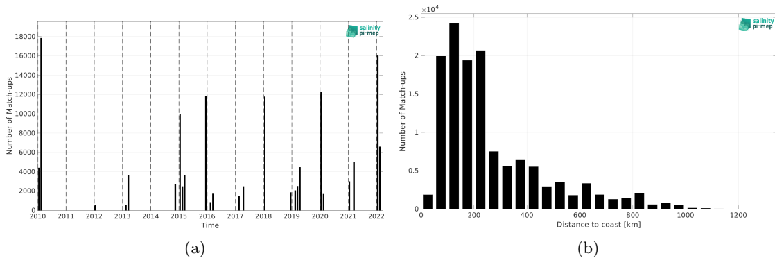
Figure 2: Number of match-ups between TSG (CSIC-UTM) and CCI SSS L4 POLAR SH Merged-OI v4.41 - 30-day running (ESA) SSS as a function of time (a) and as function of the distance to coast (b) over the Global Ocean Pi-MEP region and for the full satellite product period.
