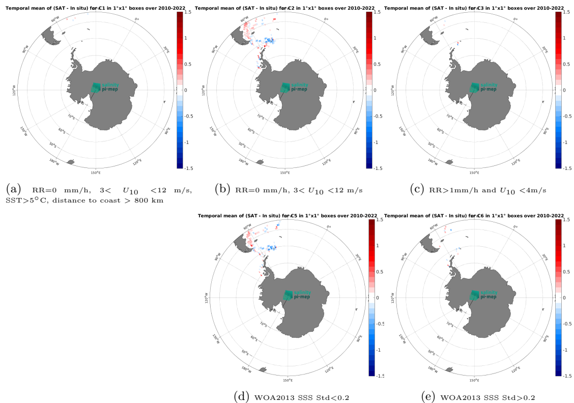
Figure 14: Temporal mean gridded over spatial boxes of size 1^\circ \times 1^\circ of \Delta\text{SSS} (CCI SSS L4 POLAR SH Merged-OI v4.41 - 30-day running (ESA) - TSG (CSIC-UTM)) for 5 different subdatasets corresponding to:RR=0 mm/h, 3 < U_{10} < 12 m/s, SST>5°C, distance to coast > 800 km (a), RR=0 mm/h, 3 < U_{10} < 12 m/s (b), RR>1mm/h and U_{10} < 4 m/s (c), WOA2013 SSS Std<0.2 (d), WOA2013 SSS Std>0.2 (e).
