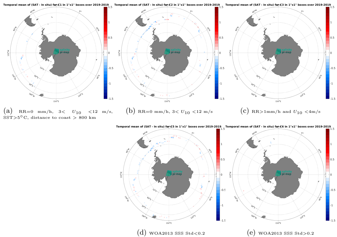
Figure 14: Temporal mean gridded over spatial boxes of size 1^\circ \times 1^\circ of \Delta\text{SSS} (CCI SSS L4 POLAR SH Merged-OI v4.41 - 30-day running (ESA) - Sailability) for 5 different subdatasets corresponding to:RR=0 mm/h, 3 < U_{10} < 12 m/s, SST>5°C, distance to coast > 800 km (a), RR=0 mm/h, 3 < U_{10} < 12 m/s (b), RR>1mm/h and U_{10} < 4 m/s (c), WOA2013 SSS Std<0.2 (d), WOA2013 SSS Std>0.2 (e).
