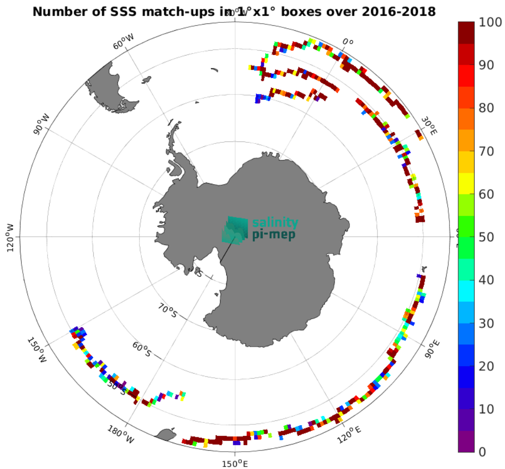
Figure 4: Number of SSS match-ups between Surface drifters SSS and the CCI SSS L4 POLAR SH Merged-OI v4.41 - 30-day running (ESA) SSS product for the Global Ocean Pi-MEP region over 1^\circ \times 1^\circ boxes and for the full satellite product period.
