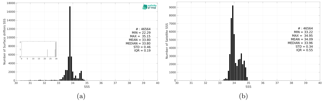
Figure 3: Histograms of SSS from Surface drifters (a) and CCI SSS L4 POLAR SH Merged-OI v4.41 - 30-day running (ESA) (b) considering all match-up pairs per bins of 0.1 over the Global Ocean Pi-MEP region and for the full satellite product period.
