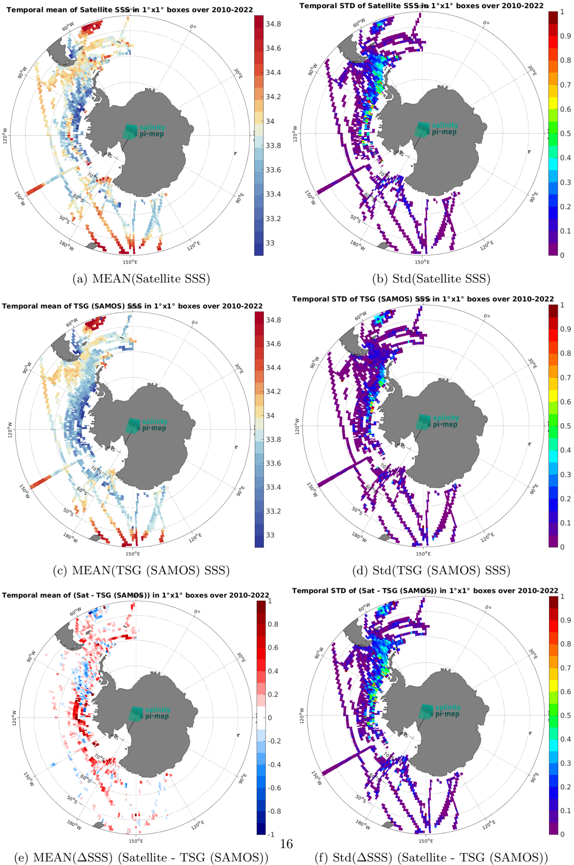
Figure 6: Temporal mean (left) and Std (right) of SSS from CCI SSS L4 POLAR SH Merged-OI v4.4 - 7-day running (ESA) (top), TSG (SAMOS) (middle), and of \Delta SSS (Satellite - TSG (SAMOS)). Only match-up pairs are used to generate these maps.
