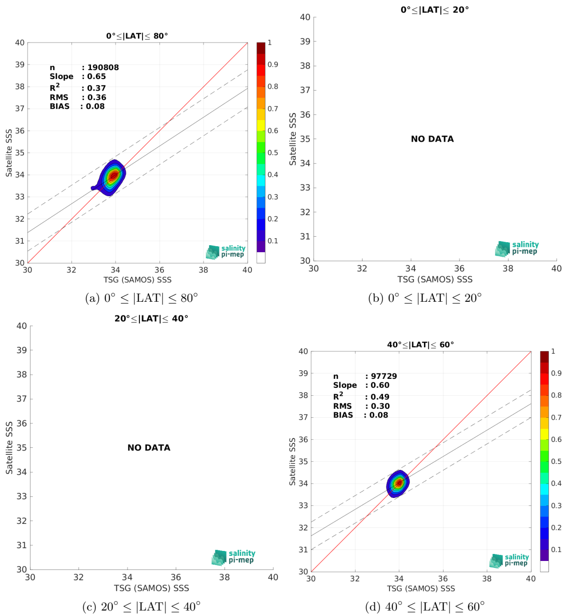
Figure 9: Contour maps of the concentration of CCI SSS L4 POLAR SH Merged-OI v4.4 - 7-day running (ESA) SSS (y-axis) versus TSG (SAMOS) SSS (x-axis) at match-up pairs for different latitude bands. For each plot, the red line shows x=y . The black thin and dashed lines indicate a linear fit through the data cloud and the \pm 95\% confidence levels, respectively. The number match-up pairs n , the slope and R^2 coefficient of the linear fit, the root mean square (RMS) and the mean bias between satellite and in situ data are indicated for each latitude band in each plots.
