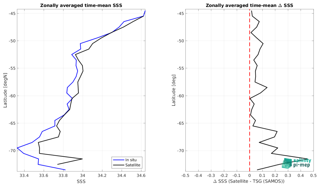
Figure 8: Left panel: Zonal mean SSS from CCI SSS L4 POLAR SH Merged-OI v4.4 - 7-day running (ESA) satellite product (black) and from TSG (SAMOS) (blue). Right panel: Zonal mean of \Delta SSS (Satellite - TSG (SAMOS)) for all the collected Pi-MEP match-up pairs estimated over the full satellite product period.
