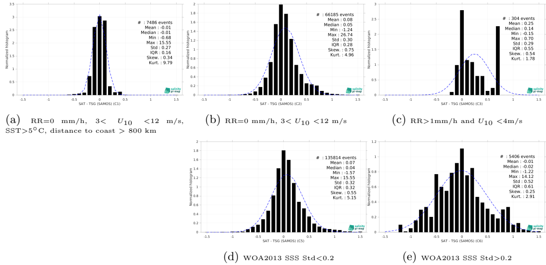
Figure 13: Normalized histogram of \Delta\text{SSS} (CCI SSS L4 POLAR SH Merged-OI v4.4 - 7-day running (ESA) - TSG (SAMOS)) for 5 different subdatasets corresponding to: RR=0 mm/h, 3 < U_{10} < 12 m/s, SST>5°C, distance to coast > 800 km (a), RR=0 mm/h, 3 < U_{10} < 12 m/s (b), RR>1mm/h and U_{10} < 4 m/s (c), WOA2013 SSS Std<0.2 (d), WOA2013 SSS Std>0.2 (e).
