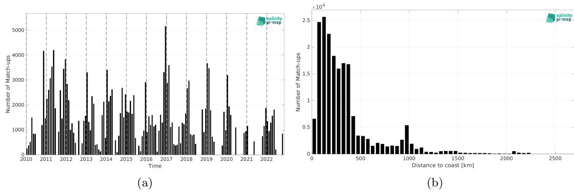
Figure 1: Number of match-ups between TSG (SAMOS) and CCI SSS L4 POLAR SH Merged-OI v4.4 - 7-day running (ESA) SSS as a function of time (a) and as function of the distance to coast (b) over the Global Ocean Pi-MEP region and for the full satellite product period.
