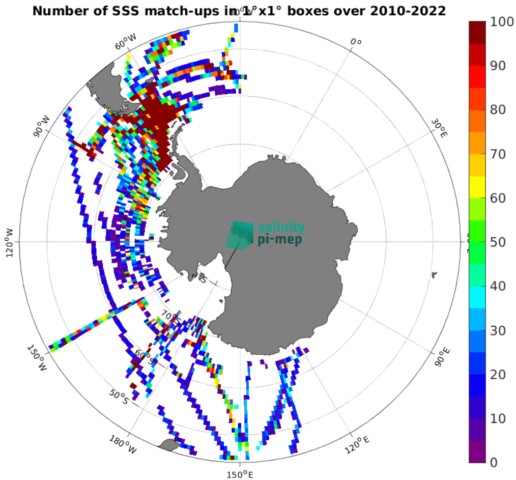
Figure 4: Number of SSS match-ups between TSG (SAMOS) SSS and the CCI SSS L4 POLAR SH Merged-OI v4.4 - 7-day running (ESA) SSS product for the Global Ocean Pi-MEP region over 1^\circ \times 1^\circ boxes and for the full satellite product period.
