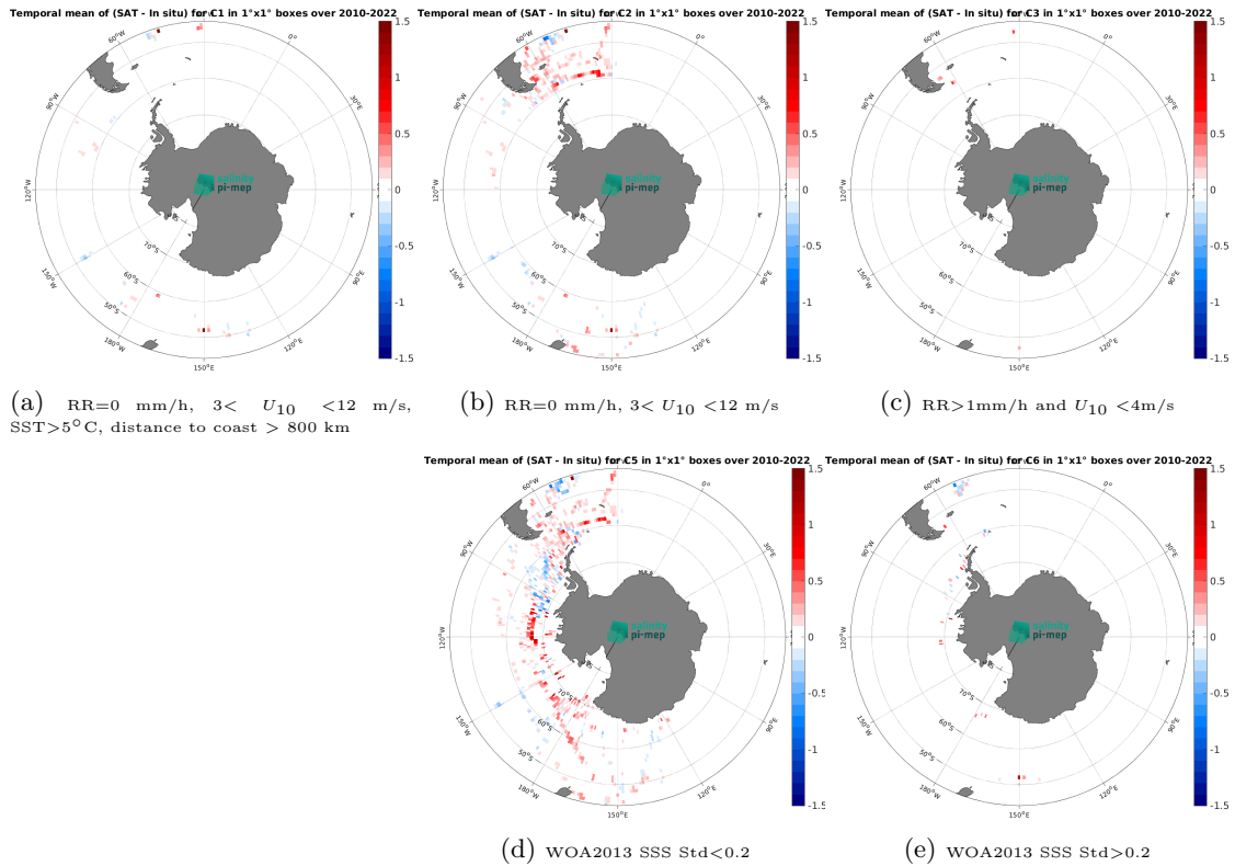
Figure 12: Temporal mean gridded over spatial boxes of size 1^{\circ}\times 1^{\circ} of \Delta\text{SSS} (CCI SSS L4 POLAR SH Merged-OI v4.4 - 7-day running (ESA) - TSG (SAMOS)) for 5 different subdatasets corresponding to: RR=0 mm/h, 3 < U_{10} < 12 m/s, SST > 5^{\circ}\text{C} , distance to coast > 800 km (a), RR=0 mm/h, 3 < U_{10} < 12 m/s (b), RR > 1 mm/h and U_{10} < 4 m/s (c), WOA2013 SSS Std < 0.2 (d), WOA2013 SSS Std > 0.2 (e).
