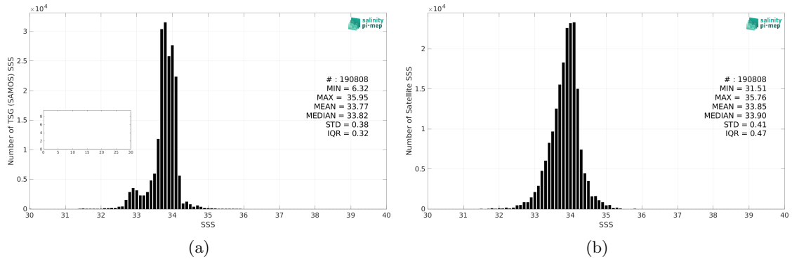
Figure 2: Histograms of SSS from TSG (SAMOS) (a) and CCI SSS L4 POLAR SH Merged-OI v4.4 - 7-day running (ESA) (b) considering all match-up pairs per bins of 0.1 over the Global Ocean Pi-MEP region and for the full satellite product period.
