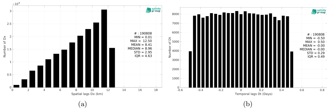
Figure 5: Histograms of the spatial (a) and temporal (b) lags between the location/time of the TSG (SAMOS) measurement and the date of the corresponding CCI SSS L4 POLAR SH Merged-OI v4.4 - 7-day running (ESA) SSS pixel.
