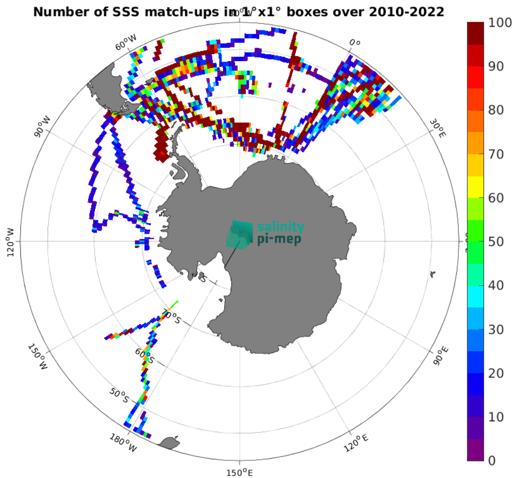
Figure 4: Number of SSS match-ups between TSG (Polarstern) SSS and the CCI SSS L4 POLAR SH Merged-OI v4.4 - 7-day running (ESA) SSS product for the Global Ocean Pi-MEP region over 1^\circ \times 1^\circ boxes and for the full satellite product period.
