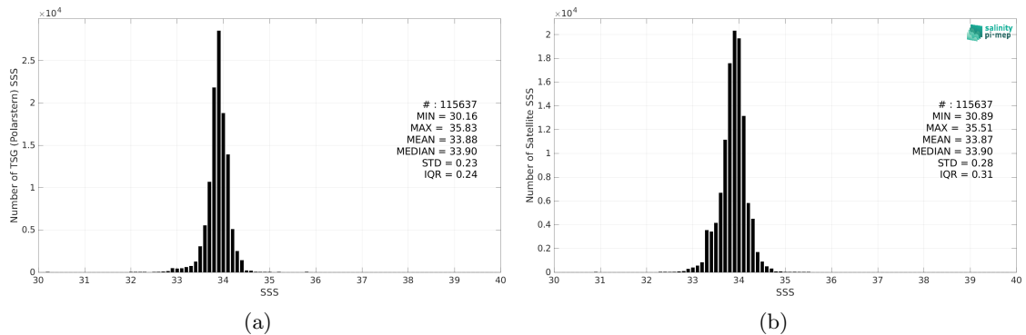
Figure 2: Histograms of SSS from TSG (Polarstern) (a) and CCI SSS L4 POLAR SH Merged-OI v4.4 - 7-day running (ESA) (b) considering all match-up pairs per bins of 0.1 over the Global Ocean Pi-MEP region and for the full satellite product period.
