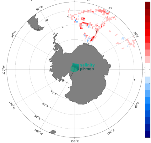
(e) MEAN( \Delta SSS) (Satellite - TSG (NCEI-0170743))
