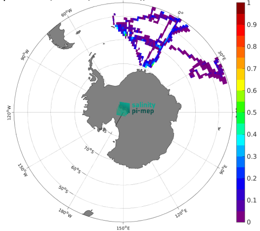
(f) Std( \Delta SSS) (Satellite - TSG (NCEI-0170743))
