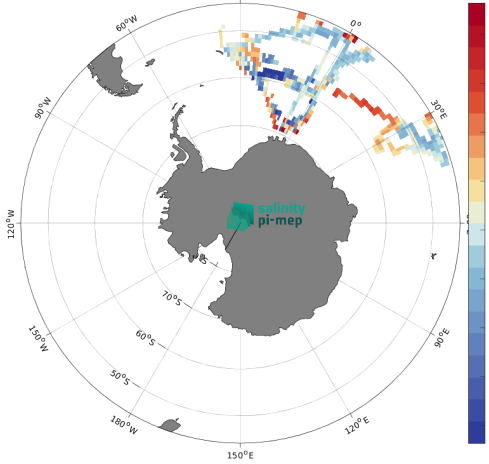
(c) MEAN(TSG (NCEI-0170743) SSS)
