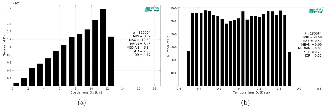
Figure 5: Histograms of the spatial (a) and temporal (b) lags between the location/time of the TSG (NCEI-0170743) measurement and the date of the corresponding CCI SSS L4 POLAR SH Merged-OI v4.4 - 7-day running (ESA) SSS pixel.
