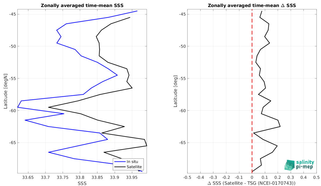
Figure 8: Left panel: Zonal mean SSS from CCI SSS L4 POLAR SH Merged-OI v4.4 - 7-day running (ESA) satellite product (black) and from TSG (NCEI-0170743) (blue). Right panel: Zonal mean of \Delta SSS (Satellite - TSG (NCEI-0170743)) for all the collected Pi-MEP match-up pairs estimated over the full satellite product period.
