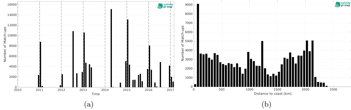
Figure 1: Number of match-ups between TSG (NCEI-0170743) and CCI SSS L4 POLAR SH Merged-OI v4.4 - 7-day running (ESA) SSS as a function of time (a) and as function of the distance to coast (b) over the Global Ocean Pi-MEP region and for the full satellite product period.
