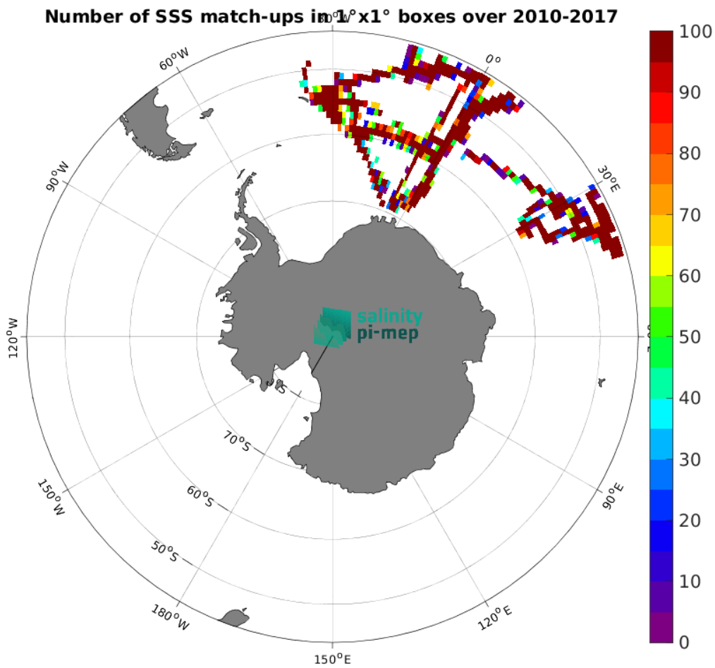
Figure 4: Number of SSS match-ups between TSG (NCEI-0170743) SSS and the CCI SSS L4 POLAR SH Merged-OI v4.4 - 7-day running (ESA) SSS product for the Global Ocean Pi-MEP region over 1^\circ \times 1^\circ boxes and for the full satellite product period.
