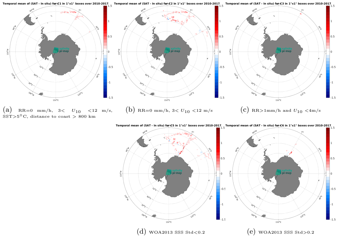
Figure 12: Temporal mean gridded over spatial boxes of size 1^{\circ}\times 1^{\circ} of \Delta\text{SSS} (CCI SSS L4 POLAR SH Merged-OI v4.4 - 7-day running (ESA) - TSG (NCEI-0170743)) for 5 different subdatasets corresponding to:RR=0 mm/h, 3 < U_{10} < 12 m/s, SST >5^{\circ}\text{C} , distance to coast > 800 km (a), RR=0 mm/h, 3 < U_{10} < 12 m/s (b), RR >1 mm/h and U_{10} < 4 m/s (c), WOA2013 SSS Std <0.2 (d), WOA2013 SSS Std >0.2 (e).
