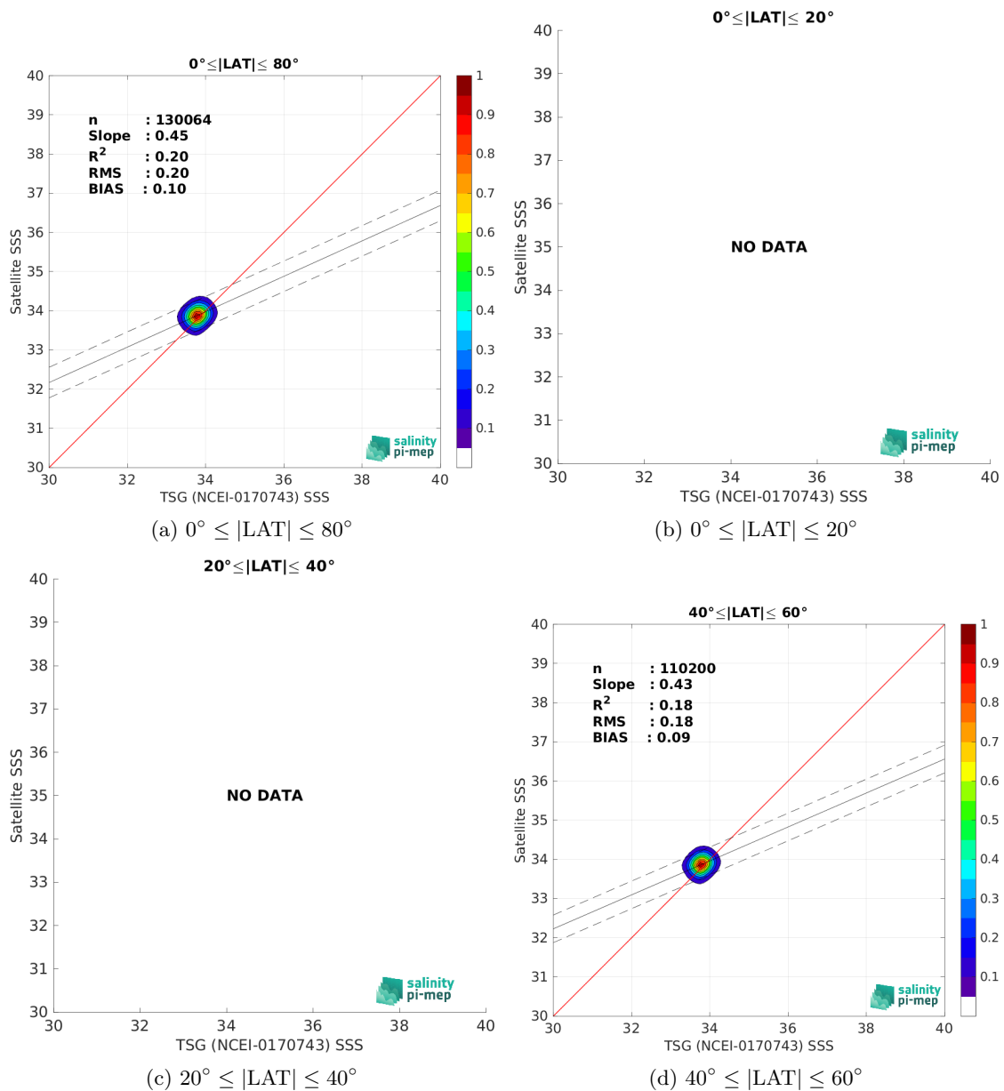
Figure 9: Contour maps of the concentration of CCI SSS L4 POLAR SH Merged-OI v4.4 - 7-day running (ESA) SSS (y-axis) versus TSG (NCEI-0170743) SSS (x-axis) at match-up pairs for different latitude bands. For each plot, the red line shows x=y . The black thin and dashed lines indicate a linear fit through the data cloud and the \pm 95\% confidence levels, respectively. The number match-up pairs n , the slope and R^2 coefficient of the linear fit, the root mean square (RMS) and the mean bias between satellite and in situ data are indicated for each latitude band in each plots.
