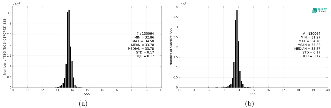
Figure 2: Histograms of SSS from TSG (NCEI-0170743) (a) and CCI SSS L4 POLAR SH Merged-OI v4.4 - 7-day running (ESA) (b) considering all match-up pairs per bins of 0.1 over the Global Ocean Pi-MEP region and for the full satellite product period.
