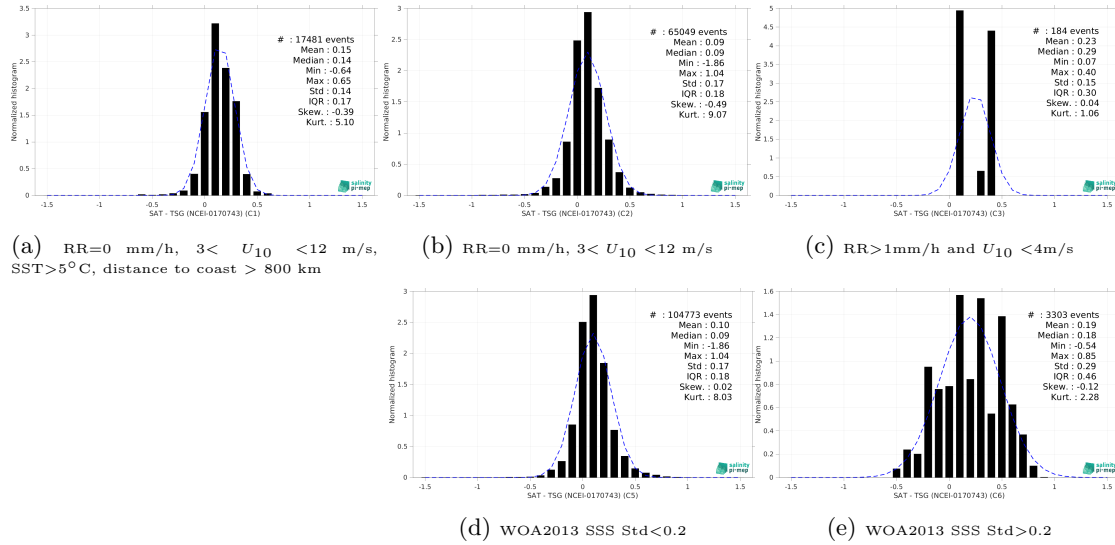
Figure 13: Normalized histogram of \Delta SSS (CCI SSS L4 POLAR SH Merged-OI v4.4 - 7-day running (ESA) - TSG (NCEI-0170743)) for 5 different subdatasets corresponding to: RR=0 mm/h, 3 < U_{10} < 12 m/s, SST>5°C, distance to coast > 800 km (a), RR=0 mm/h, 3 < U_{10} < 12 m/s (b), RR>1mm/h and U_{10} < 4 m/s (c), WOA2013 SSS Std<0.2 (d), WOA2013 SSS Std>0.2 (e).
