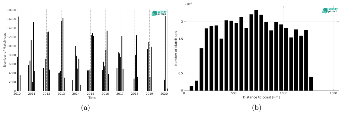
Figure 1: Number of match-ups between TSG (LEGOS-Survostral) and CCI SSS L4 POLAR SH Merged-OI v4.4 - 7-day running (ESA) SSS as a function of time (a) and as function of the distance to coast (b) over the Global Ocean Pi-MEP region and for the full satellite product period.
