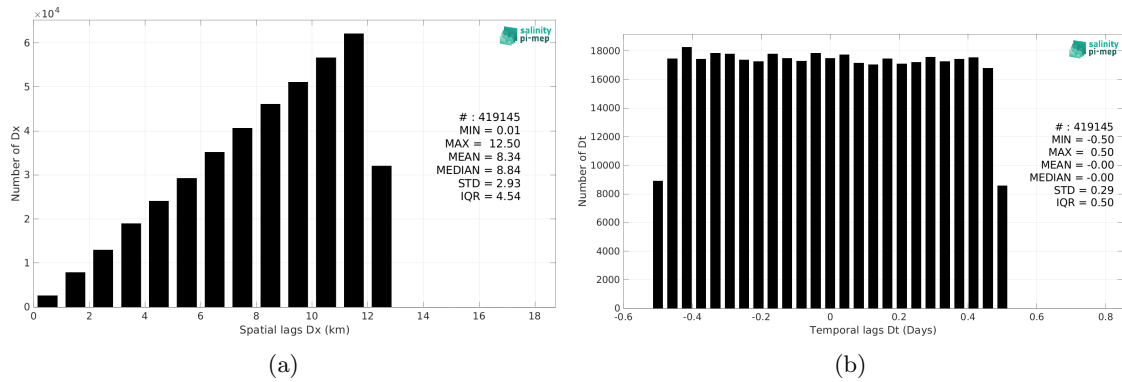
Figure 5: Histograms of the spatial (a) and temporal (b) lags between the location/time of the TSG (LEGOS-Survostral) measurement and the date of the corresponding CCI SSS L4 POLAR SH Merged-OI v4.4 - 7-day running (ESA) SSS pixel.
