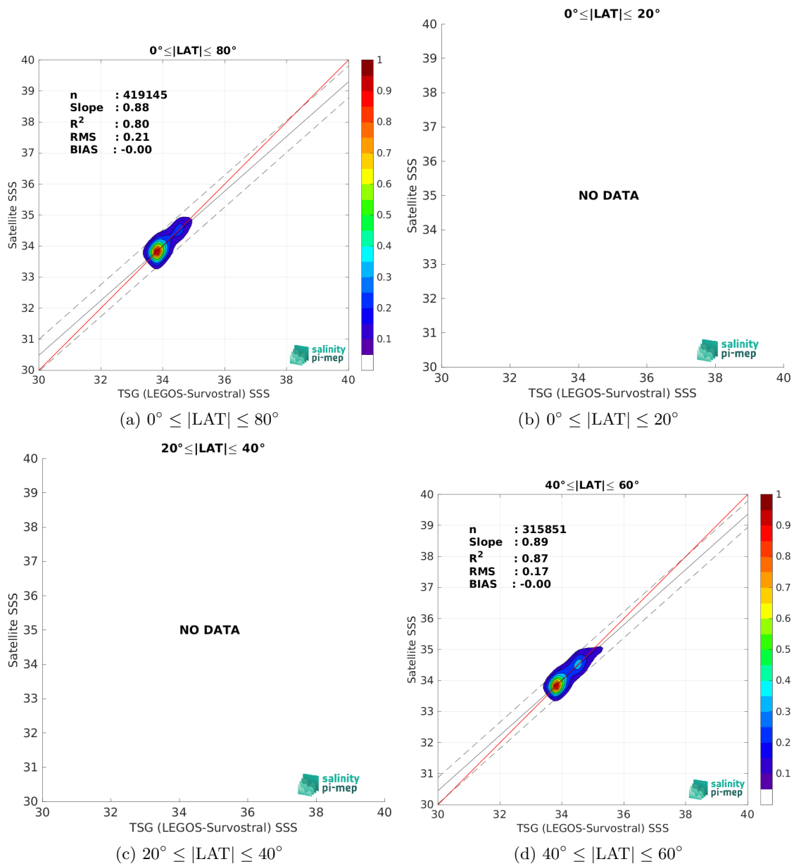
Figure 9: Contour maps of the concentration of CCI SSS L4 POLAR SH Merged-OI v4.4 - 7-day running (ESA) SSS (y-axis) versus TSG (LEGOS-Survostral) SSS (x-axis) at match-up pairs for different latitude bands. For each plot, the red line shows x=y . The black thin and dashed lines indicate a linear fit through the data cloud and the \pm 95\% confidence levels, respectively. The number match-up pairs n , the slope and R^2 coefficient of the linear fit, the root mean square (RMS) and the mean bias between satellite and in situ data are indicated for each latitude band in each plots.
