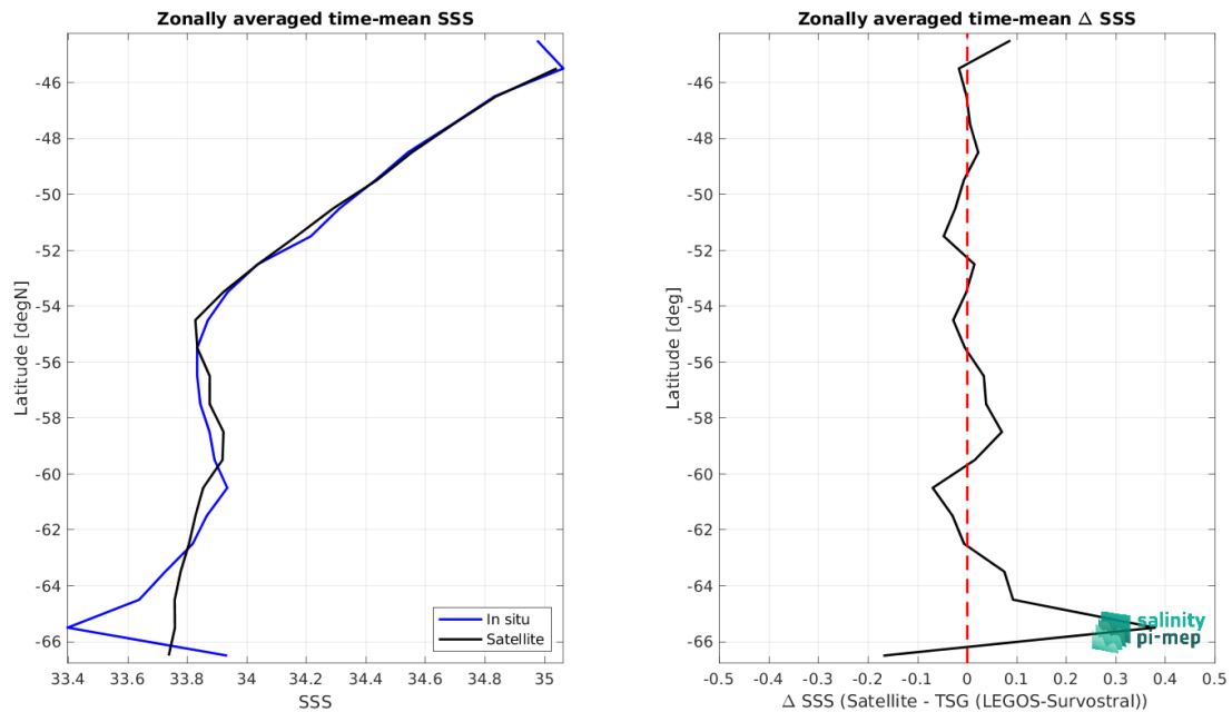
Figure 8: Left panel: Zonal mean SSS from CCI SSS L4 POLAR SH Merged-OI v4.4 - 7-day running (ESA) satellite product (black) and from TSG (LEGOS-Survostral) (blue). Right panel: Zonal mean of \Delta SSS (Satellite - TSG (LEGOS-Survostral)) for all the collected Pi-MEP match-up pairs estimated over the full satellite product period.
