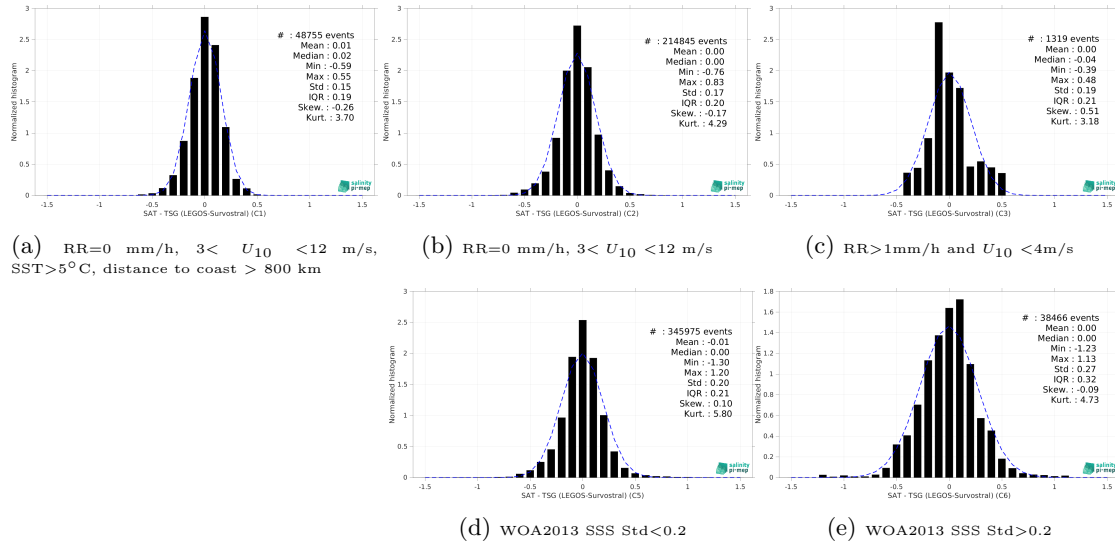
Figure 13: Normalized histogram of \Delta\text{SSS} (CCI SSS L4 POLAR SH Merged-OI v4.4 - 7-day running (ESA) - TSG (LEGOS-Survostral)) for 5 different subdatasets corresponding to: RR=0 mm/h, 3 < U_{10} < 12 m/s, SST>5°C, distance to coast > 800 km (a), RR=0 mm/h, 3 < U_{10} < 12 m/s (b), RR>1mm/h and U_{10} < 4 m/s (c), WOA2013 SSS Std<0.2 (d), WOA2013 SSS Std>0.2 (e).
