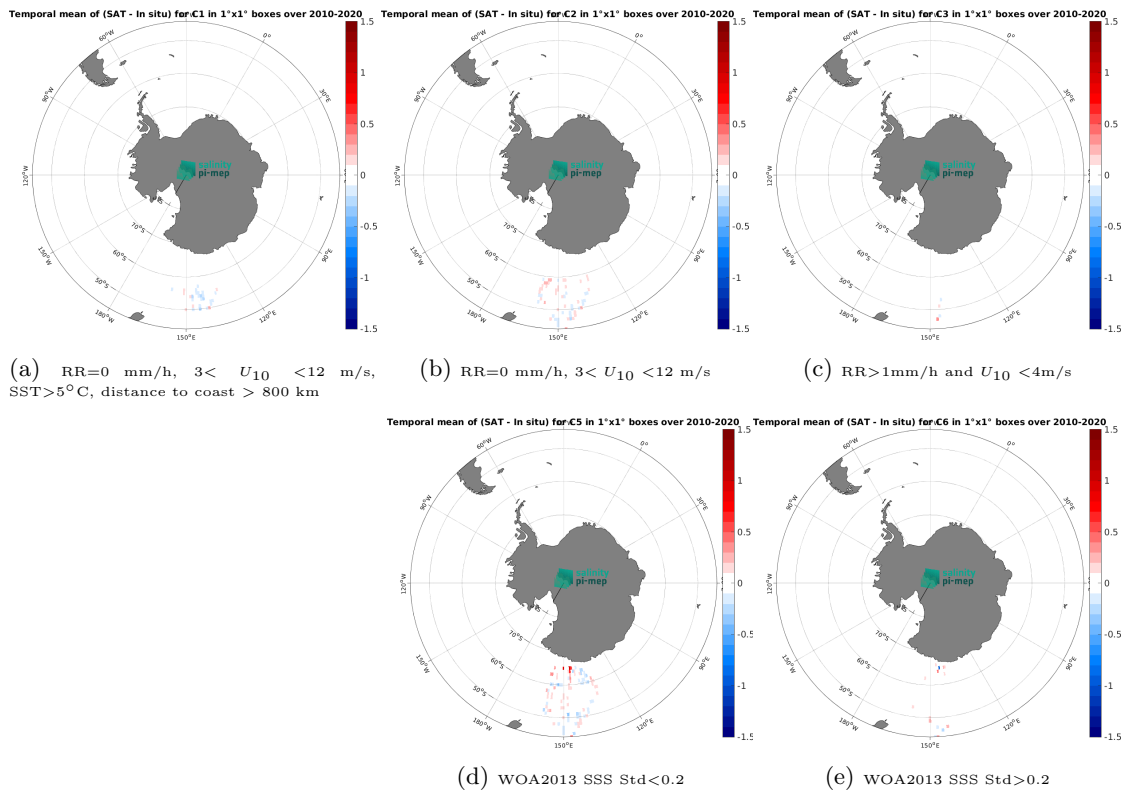
Figure 12: Temporal mean gridded over spatial boxes of size 1^\circ \times 1^\circ of \Delta SSS (CCI SSS L4 POLAR SH Merged-OI v4.4 - 7-day running (ESA) - TSG (LEGOS-Survostral)) for 5 different subdatasets corresponding to:RR=0 mm/h, 3 < U_{10} < 12 m/s, SST>5°C, distance to coast > 800 km (a), RR=0 mm/h, 3 < U_{10} < 12 m/s (b), RR>1mm/h and U_{10} < 4 m/s (c), WOA2013 SSS Std<0.2 (d), WOA2013 SSS Std>0.2 (e).
