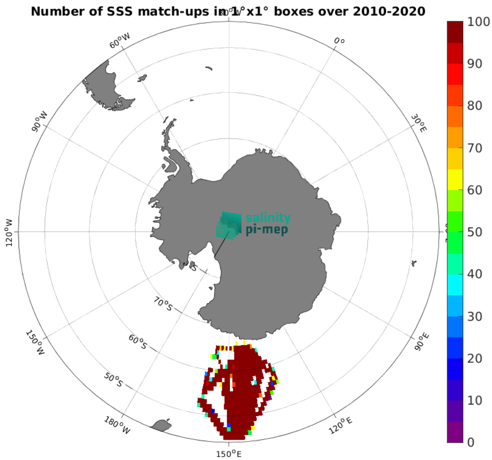
Figure 4: Number of SSS match-ups between TSG (LEGOS-Survostral) SSS and the CCI SSS L4 POLAR SH Merged-OI v4.4 - 7-day running (ESA) SSS product for the Global Ocean Pi-MEP region over 1^\circ \times 1^\circ boxes and for the full satellite product period.
