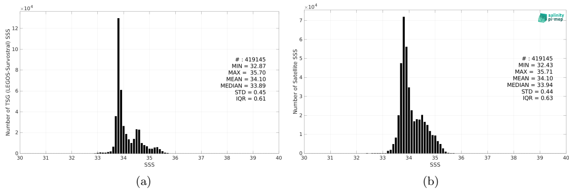
Figure 2: Histograms of SSS from TSG (LEGOS-Survostral) (a) and CCI SSS L4 POLAR SH Merged-OI v4.4 - 7-day running (ESA) (b) considering all match-up pairs per bins of 0.1 over the Global Ocean Pi-MEP region and for the full satellite product period.
