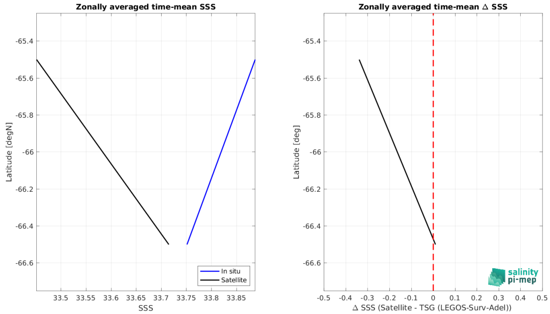
Figure 8: Left panel: Zonal mean SSS from CCI SSS L4 POLAR SH Merged-OI v4.4 - 7-day running (ESA) satellite product (black) and from TSG (LEGOS-Surv-Adel) (blue). Right panel: Zonal mean of \Delta SSS (Satellite - TSG (LEGOS-Surv-Adel)) for all the collected Pi-MEP match-up pairs estimated over the full satellite product period.
