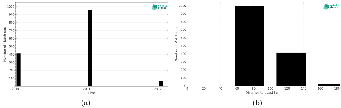
Figure 1: Number of match-ups between TSG (LEGOS-Surv-Adel) and CCI SSS L4 POLAR SH Merged-OI v4.4 - 7-day running (ESA) SSS as a function of time (a) and as function of the distance to coast (b) over the Global Ocean Pi-MEP region and for the full satellite product period.
