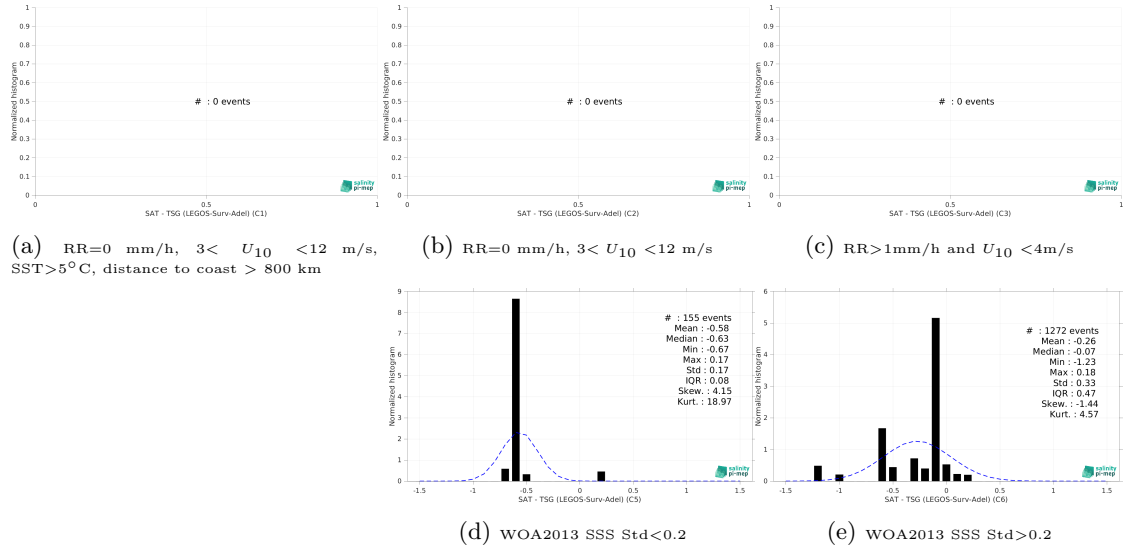
Figure 13: Normalized histogram of \Delta\text{SSS} (CCI SSS L4 POLAR SH Merged-OI v4.4 - 7-day running (ESA) - TSG (LEGOS-Surv-Adel)) for 5 different subdatasets corresponding to: RR=0 mm/h, 3 < U_{10} < 12 m/s, SST>5°C, distance to coast > 800 km (a), RR=0 mm/h, 3 < U_{10} < 12 m/s (b), RR>1mm/h and U_{10} < 4 m/s (c), WOA2013 SSS Std<0.2 (d), WOA2013 SSS Std>0.2 (e).
