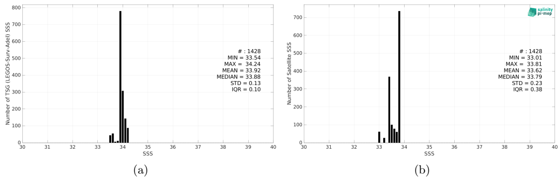
Figure 2: Histograms of SSS from TSG (LEGOS-Surv-Adel) (a) and CCI SSS L4 POLAR SH Merged-OI v4.4 - 7-day running (ESA) (b) considering all match-up pairs per bins of 0.1 over the Global Ocean Pi-MEP region and for the full satellite product period.
