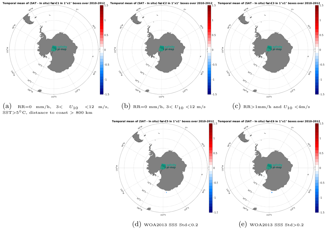
Figure 12: Temporal mean gridded over spatial boxes of size 1°×1° of \Delta SSS (CCI SSS L4 POLAR SH Merged-OI v4.4 - 7-day running (ESA) - TSG (LEGOS-Surv-Adel)) for 5 different subdatasets corresponding to:RR=0 mm/h, 3 < U_{10} < 12 m/s, SST>5°C, distance to coast > 800 km (a), RR=0 mm/h, 3 < U_{10} < 12 m/s (b), RR>1mm/h and U_{10} < 4 m/s (c), WOA2013 SSS Std<0.2 (d), WOA2013 SSS Std>0.2 (e).
