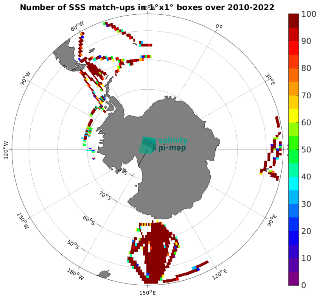
Figure 4: Number of SSS match-ups between TSG (LEGOS-DM) SSS and the CCI SSS L4 POLAR SH Merged-OI v4.4 - 7-day running (ESA) SSS product for the Global Ocean Pi-MEP region over 1^\circ \times 1^\circ boxes and for the full satellite product period.
