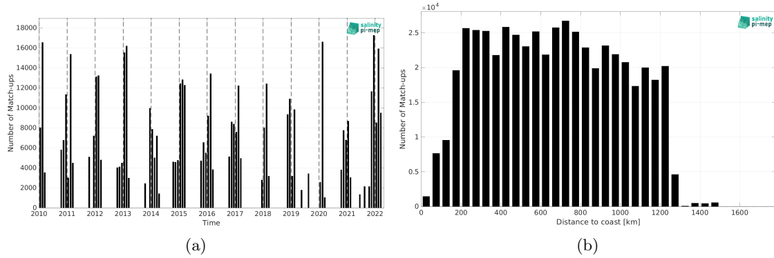
Figure 1: Number of match-ups between TSG (LEGOS-DM) and CCI SSS L4 POLAR SH Merged-OI v4.4 - 7-day running (ESA) SSS as a function of time (a) and as function of the distance to coast (b) over the Global Ocean Pi-MEP region and for the full satellite product period.
