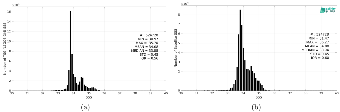
Figure 2: Histograms of SSS from TSG (LEGOS-DM) (a) and CCI SSS L4 POLAR SH Merged-OI v4.4 - 7-day running (ESA) (b) considering all match-up pairs per bins of 0.1 over the Global Ocean Pi-MEP region and for the full satellite product period.
