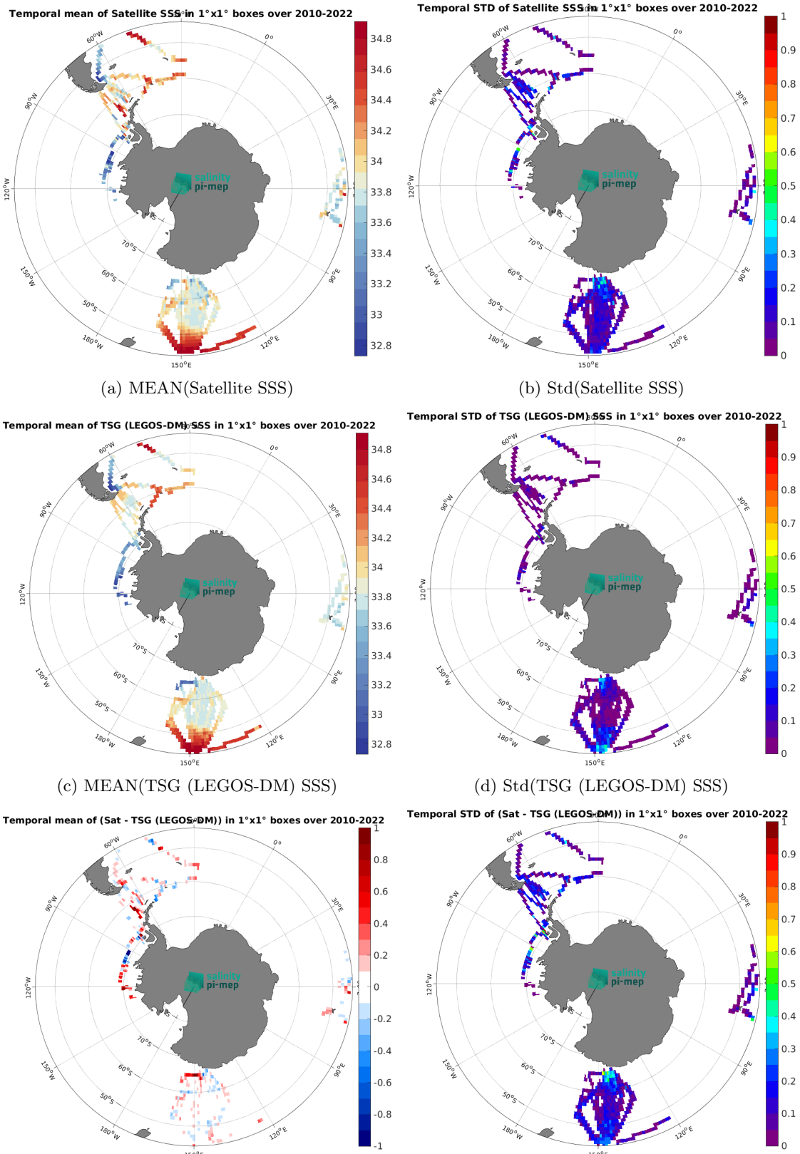
Figure 6: Temporal mean (left) and Std (right) of SSS from CCI SSS L4 POLAR SH Merged-OI v4.4 - 7-day running (ESA) (top), TSG (LEGOS-DM) (middle), and of \Delta SSS (Satellite - TSG (LEGOS-DM)). Only match-up pairs are used to generate these maps.
