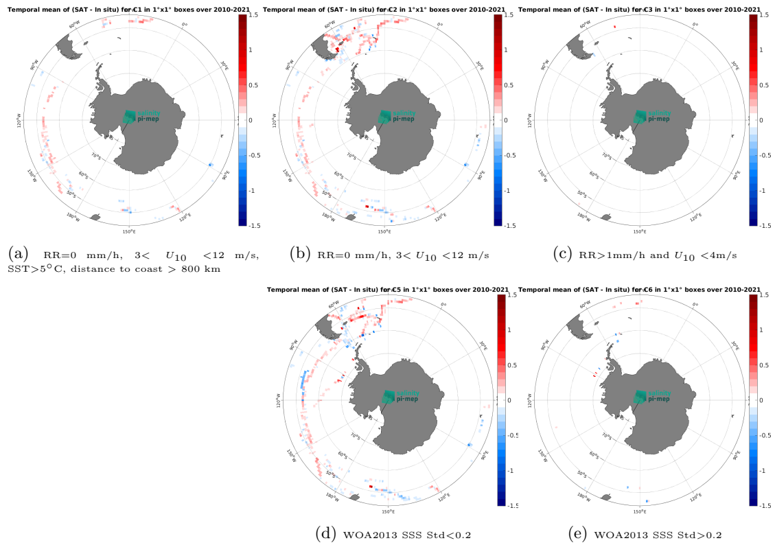
Figure 12: Temporal mean gridded over spatial boxes of size 1^\circ \times 1^\circ of \Delta SSS (CCI SSS L4 POLAR SH Merged-OI v4.4 - 7-day running (ESA) - TSG (GOSUD-Sailing-ship)) for 5 different subdatasets corresponding to:RR=0 mm/h, 3 < U_{10} < 12 m/s, SST>5°C, distance to coast > 800 km (a), RR=0 mm/h, 3 < U_{10} < 12 m/s (b), RR>1mm/h and U_{10} < 4 m/s (c), WOA2013 SSS Std<0.2 (d), WOA2013 SSS Std>0.2 (e).
