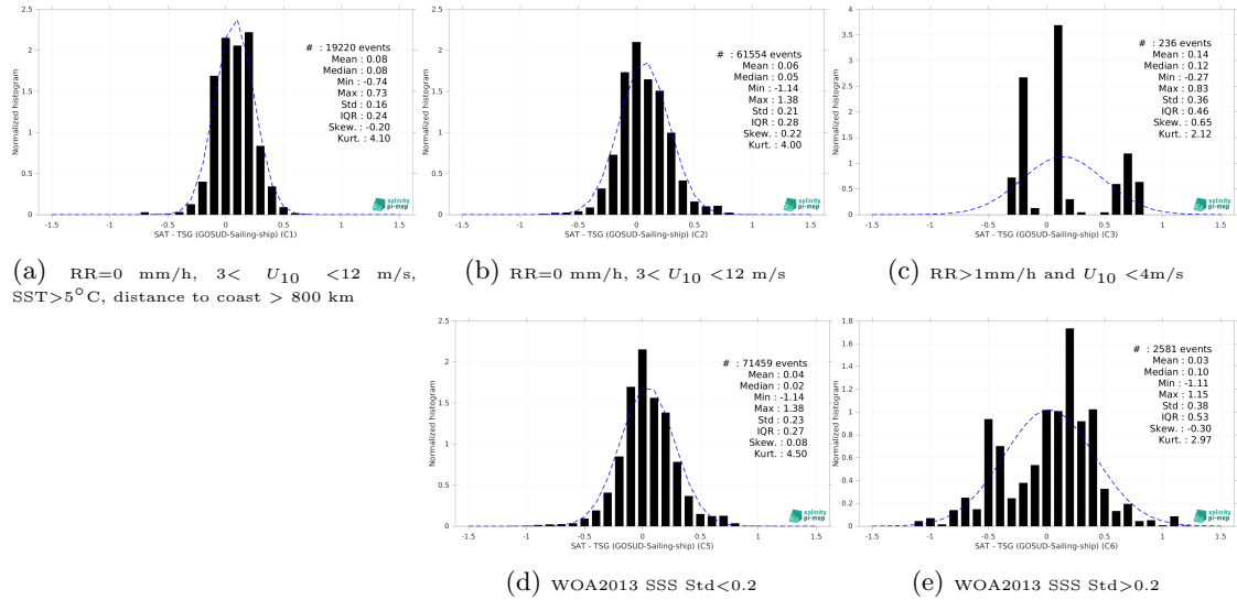
Figure 13: Normalized histogram of \Delta SSS (CCI SSS L4 POLAR SH Merged-OI v4.4 - 7-day running (ESA) - TSG (GOSUD-Sailing-ship)) for 5 different subdatasets corresponding to: RR=0 mm/h, 3 < U_{10} < 12 m/s, SST>5°C, distance to coast > 800 km (a), RR=0 mm/h, 3 < U_{10} < 12 m/s (b), RR>1mm/h and U_{10} < 4 m/s (c), WOA2013 SSS Std<0.2 (d), WOA2013 SSS Std>0.2 (e).
