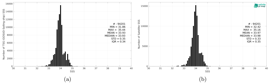
Figure 2: Histograms of SSS from TSG (GOSUD-Sailing-ship) (a) and CCI SSS L4 POLAR SH Merged-OI v4.4 - 7-day running (ESA) (b) considering all match-up pairs per bins of 0.1 over the Global Ocean Pi-MEP region and for the full satellite product period.
