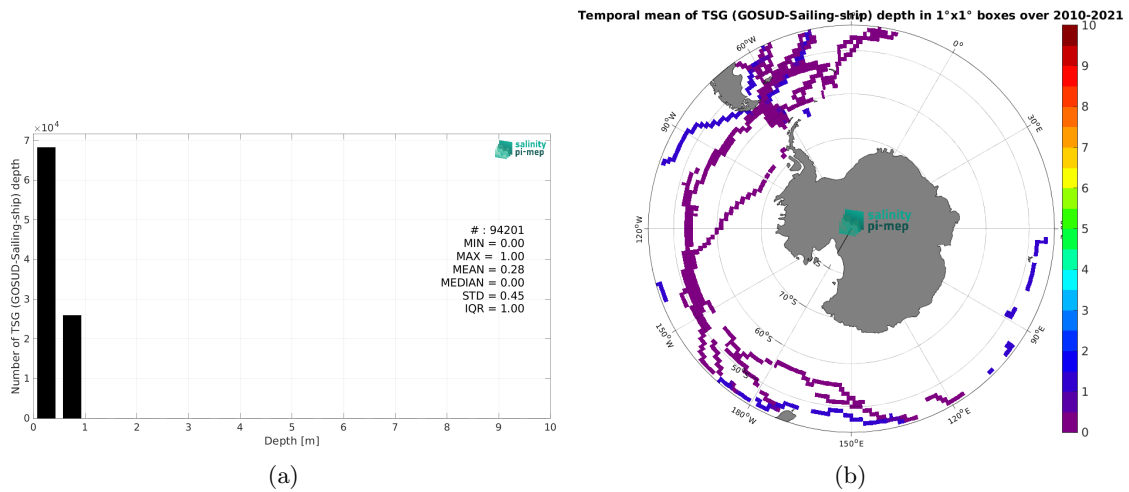
Figure 3: Histograms of the depth of the upper level SSS measurements from TSG (GOSUD-Sailing-ship) in the Match-up DataBase for the Global Ocean Pi-MEP region (a) and temporal mean spatial distribution of pressure of the in situ SSS data over 1^\circ \times 1^\circ boxes and for the full satellite product period (b).
