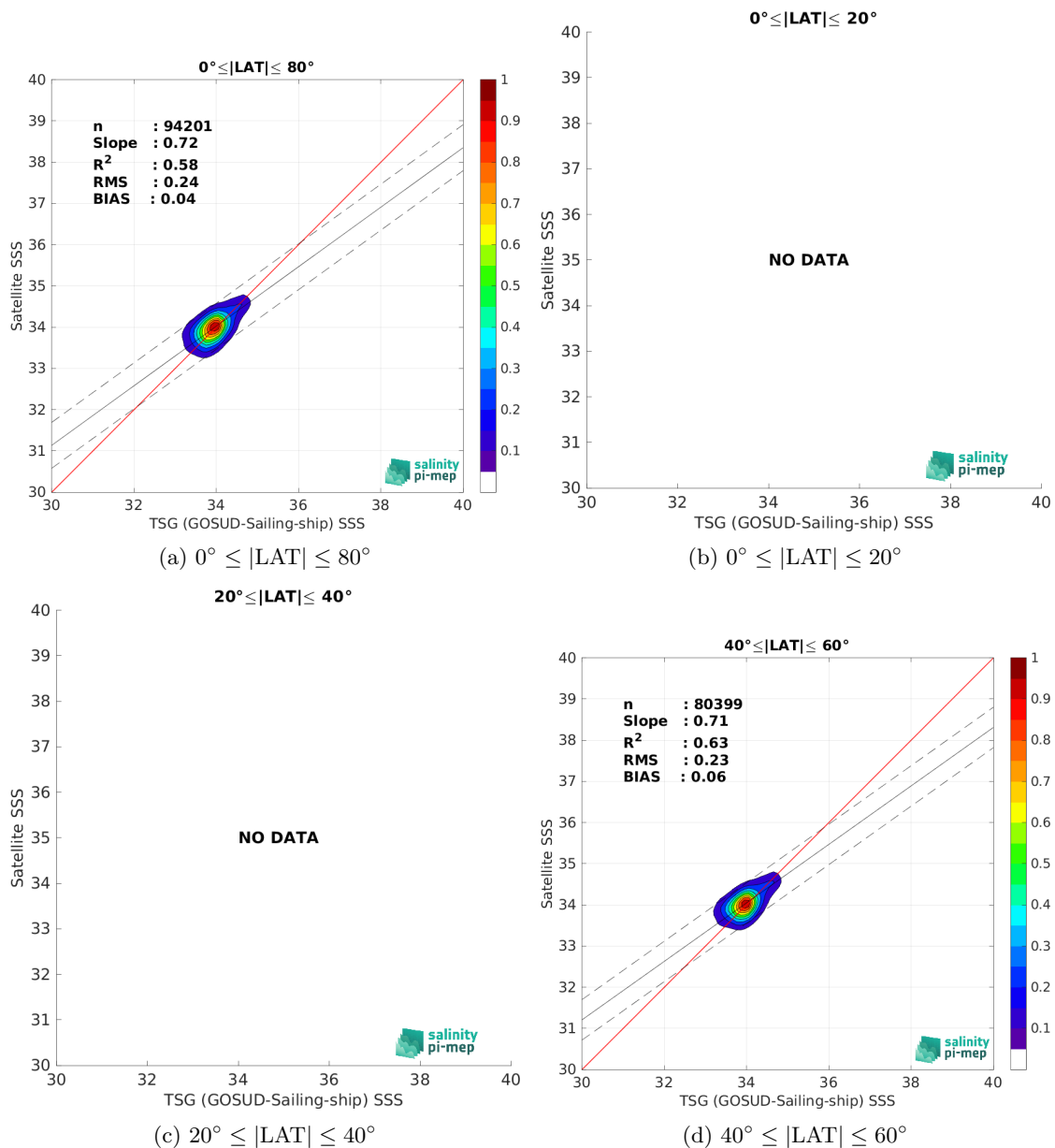
Figure 9: Contour maps of the concentration of CCI SSS L4 POLAR SH Merged-OI v4.4 - 7-day running (ESA) SSS (y-axis) versus TSG (GOSUD-Sailing-ship) SSS (x-axis) at match-up pairs for different latitude bands. For each plot, the red line shows x=y . The black thin and dashed lines indicate a linear fit through the data cloud and the \pm 95\% confidence levels, respectively. The number match-up pairs n , the slope and R^2 coefficient of the linear fit, the root mean square (RMS) and the mean bias between satellite and in situ data are indicated for each latitude band in each plots.
