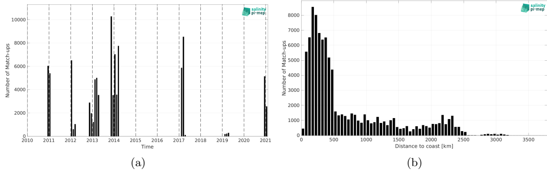
Figure 1: Number of match-ups between TSG (GOSUD-Sailing-ship) and CCI SSS L4 POLAR SH Merged-OI v4.4 - 7-day running (ESA) SSS as a function of time (a) and as function of the distance to coast (b) over the Global Ocean Pi-MEP region and for the full satellite product period.
