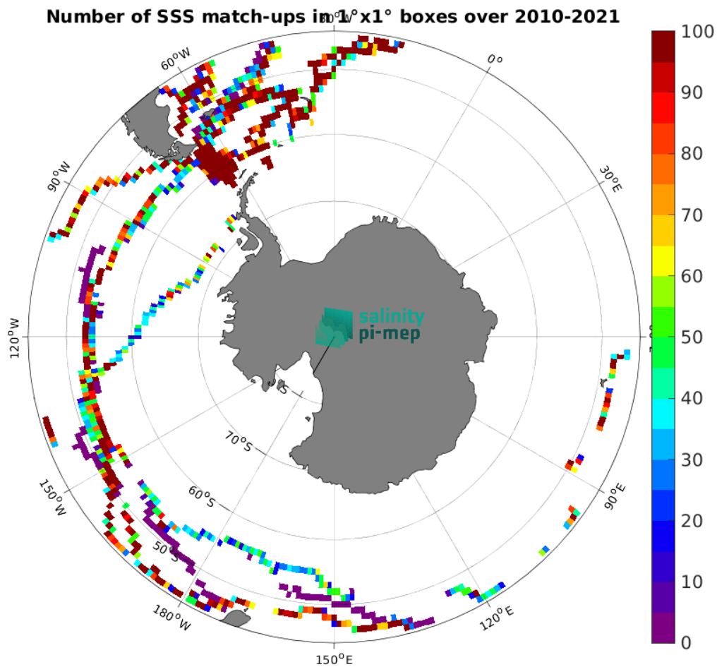
Figure 4: Number of SSS match-ups between TSG (GOSUD-Sailing-ship) SSS and the CCI SSS L4 POLAR SH Merged-OI v4.4 - 7-day running (ESA) SSS product for the Global Ocean Pi-MEP region over 1^{\circ} \times 1^{\circ} boxes and for the full satellite product period.
