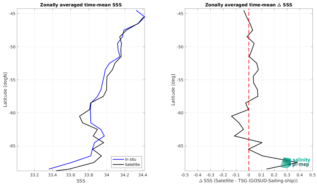
Figure 8: Left panel: Zonal mean SSS from CCI SSS L4 POLAR SH Merged-OI v4.4 - 7-day running (ESA) satellite product (black) and from TSG (GOSUD-Sailing-ship) (blue). Right panel: Zonal mean of \Delta SSS (Satellite - TSG (GOSUD-Sailing-ship)) for all the collected Pi-MEP match-up pairs estimated over the full satellite product period.
