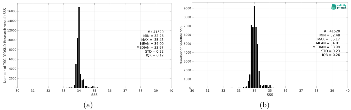
Figure 2: Histograms of SSS from TSG (GOSUD-Research-vessel) (a) and CCI SSS L4 POLAR SH Merged-OI v4.4 - 7-day running (ESA) (b) considering all match-up pairs per bins of 0.1 over the Global Ocean Pi-MEP region and for the full satellite product period.
