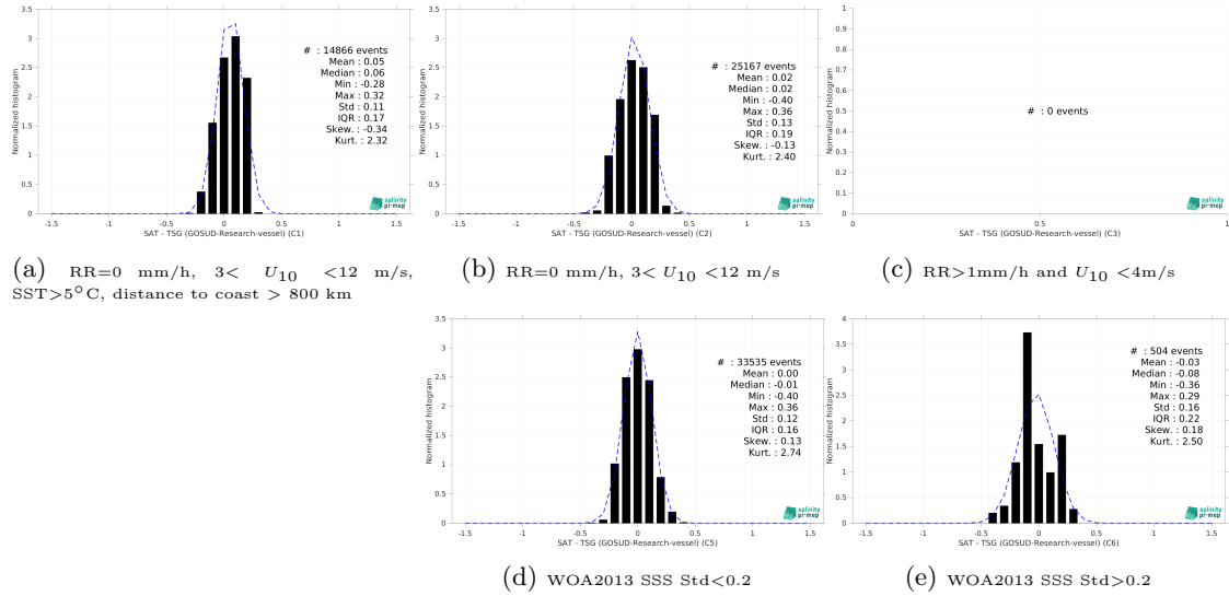
Figure 13: Normalized histogram of \Delta SSS (CCI SSS L4 POLAR SH Merged-OI v4.4 - 7-day running (ESA) - TSG (GOSUD-Research-vessel)) for 5 different subdatasets corresponding to: RR=0 mm/h, 3 < U_{10} < 12 m/s, SST>5°C, distance to coast > 800 km (a), RR=0 mm/h, 3 < U_{10} < 12 m/s (b), RR>1mm/h and U_{10} < 4 m/s (c), WOA2013 SSS Std<0.2 (d), WOA2013 SSS Std>0.2 (e).
