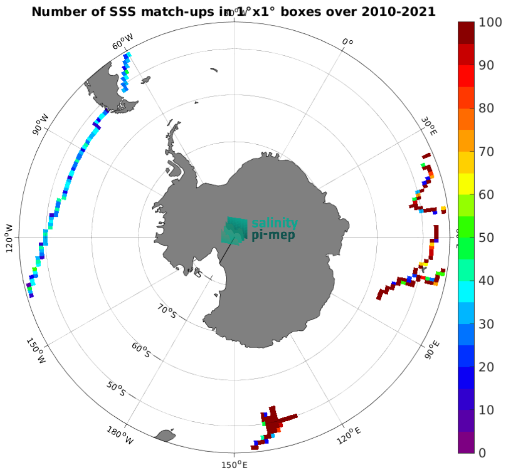
Figure 4: Number of SSS match-ups between TSG (GOSUD-Research-vessel) SSS and the CCI SSS L4 POLAR SH Merged-OI v4.4 - 7-day running (ESA) SSS product for the Global Ocean Pi-MEP region over 1^{\circ} \times 1^{\circ} boxes and for the full satellite product period.
