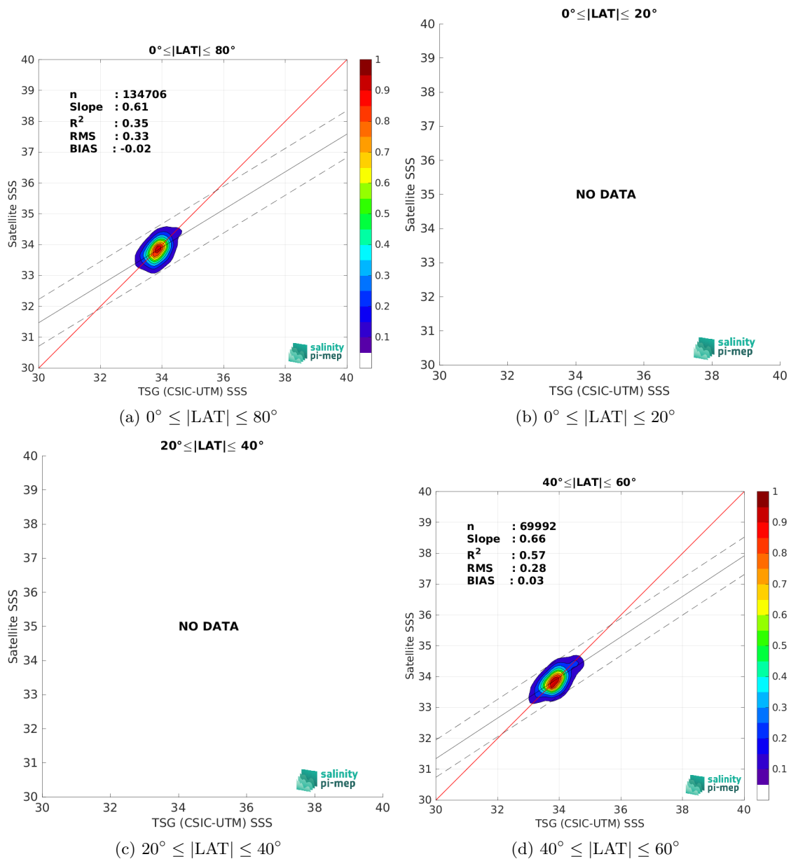
Figure 9: Contour maps of the concentration of CCI SSS L4 POLAR SH Merged-OI v4.4 - 7-day running (ESA) SSS (y-axis) versus TSG (CSIC-UTM) SSS (x-axis) at match-up pairs for different latitude bands. For each plot, the red line shows x=y . The black thin and dashed lines indicate a linear fit through the data cloud and the \pm 95\% confidence levels, respectively. The number match-up pairs n , the slope and R^2 coefficient of the linear fit, the root mean square (RMS) and the mean bias between satellite and in situ data are indicated for each latitude band in each plots.
