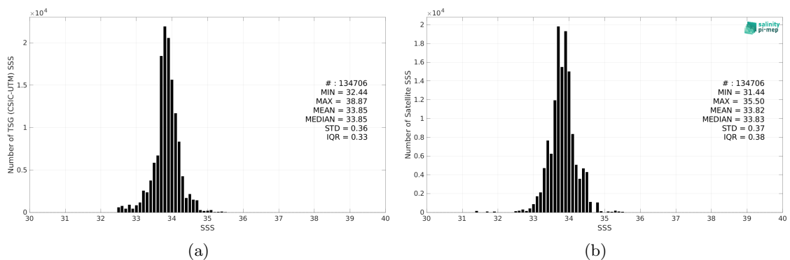
Figure 2: Histograms of SSS from TSG (CSIC-UTM) (a) and CCI SSS L4 POLAR SH Merged-OI v4.4 - 7-day running (ESA) (b) considering all match-up pairs per bins of 0.1 over the Global Ocean Pi-MEP region and for the full satellite product period.
