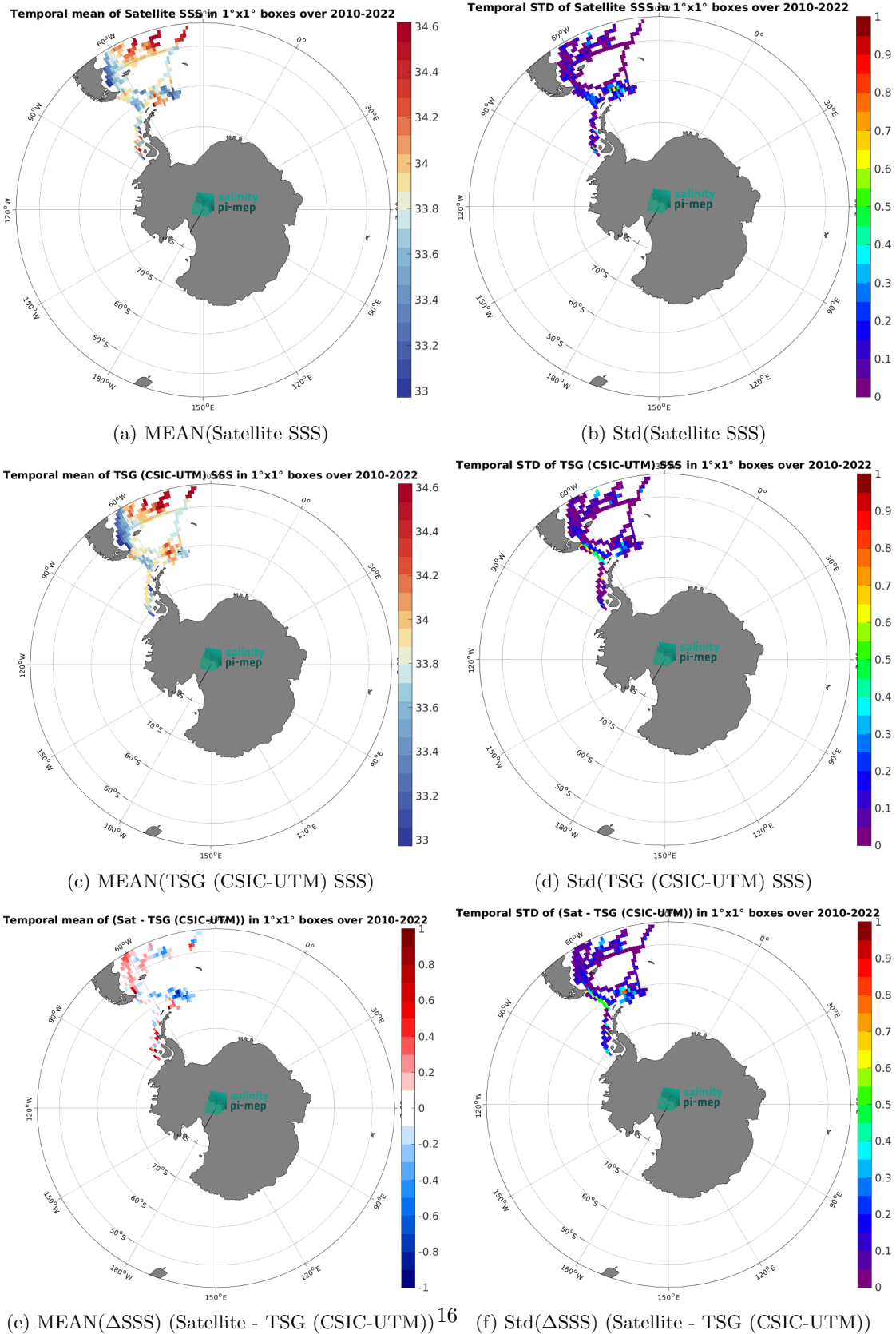
Figure 6: Temporal mean (left) and Std (right) of SSS from CCI SSS L4 POLAR SH Merged-OI v4.4 - 7-day running (ESA) (top), TSG (CSIC-UTM) (middle), and of \Delta SSS (Satellite - TSG (CSIC-UTM)). Only match-up pairs are used to generate these maps.
