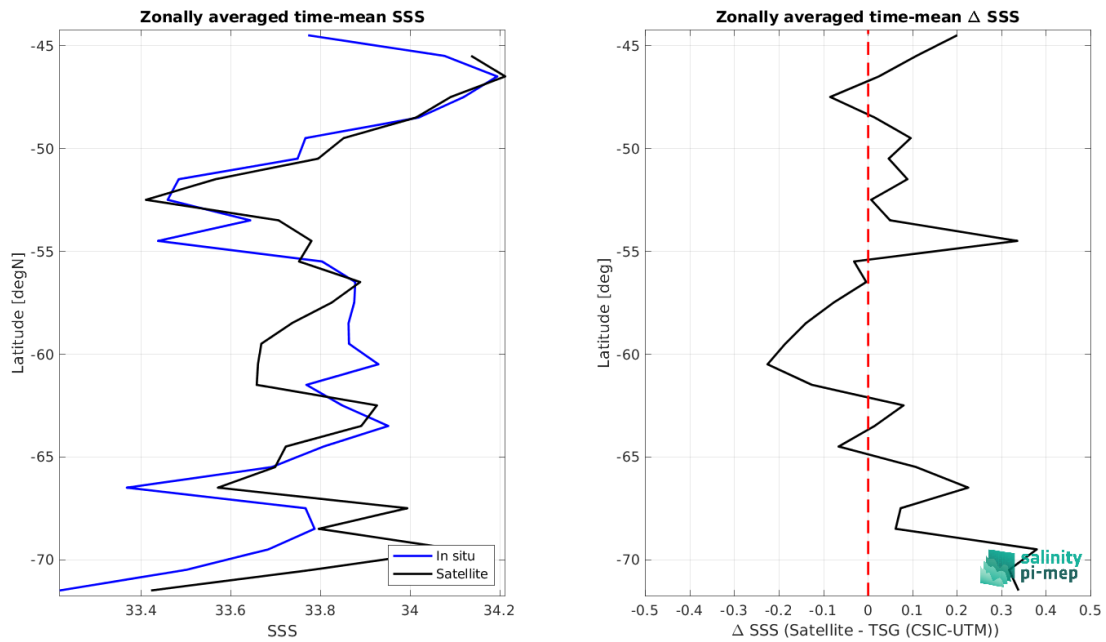
Figure 8: Left panel: Zonal mean SSS from CCI SSS L4 POLAR SH Merged-OI v4.4 - 7-day running (ESA) satellite product (black) and from TSG (CSIC-UTM) (blue). Right panel: Zonal mean of \Delta SSS (Satellite - TSG (CSIC-UTM)) for all the collected Pi-MEP match-up pairs estimated over the full satellite product period.
