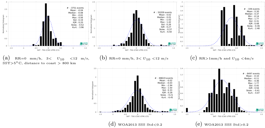
Figure 13: Normalized histogram of \Delta SSS (CCI SSS L4 POLAR SH Merged-OI v4.4 - 7-day running (ESA) - TSG (CSIC-UTM)) for 5 different subdatasets corresponding to: RR=0 mm/h, 3 < U_{10} < 12 m/s, SST>5°C, distance to coast > 800 km (a), RR=0 mm/h, 3 < U_{10} < 12 m/s (b), RR>1mm/h and U_{10} < 4 m/s (c), WOA2013 SSS Std<0.2 (d), WOA2013 SSS Std>0.2 (e).
