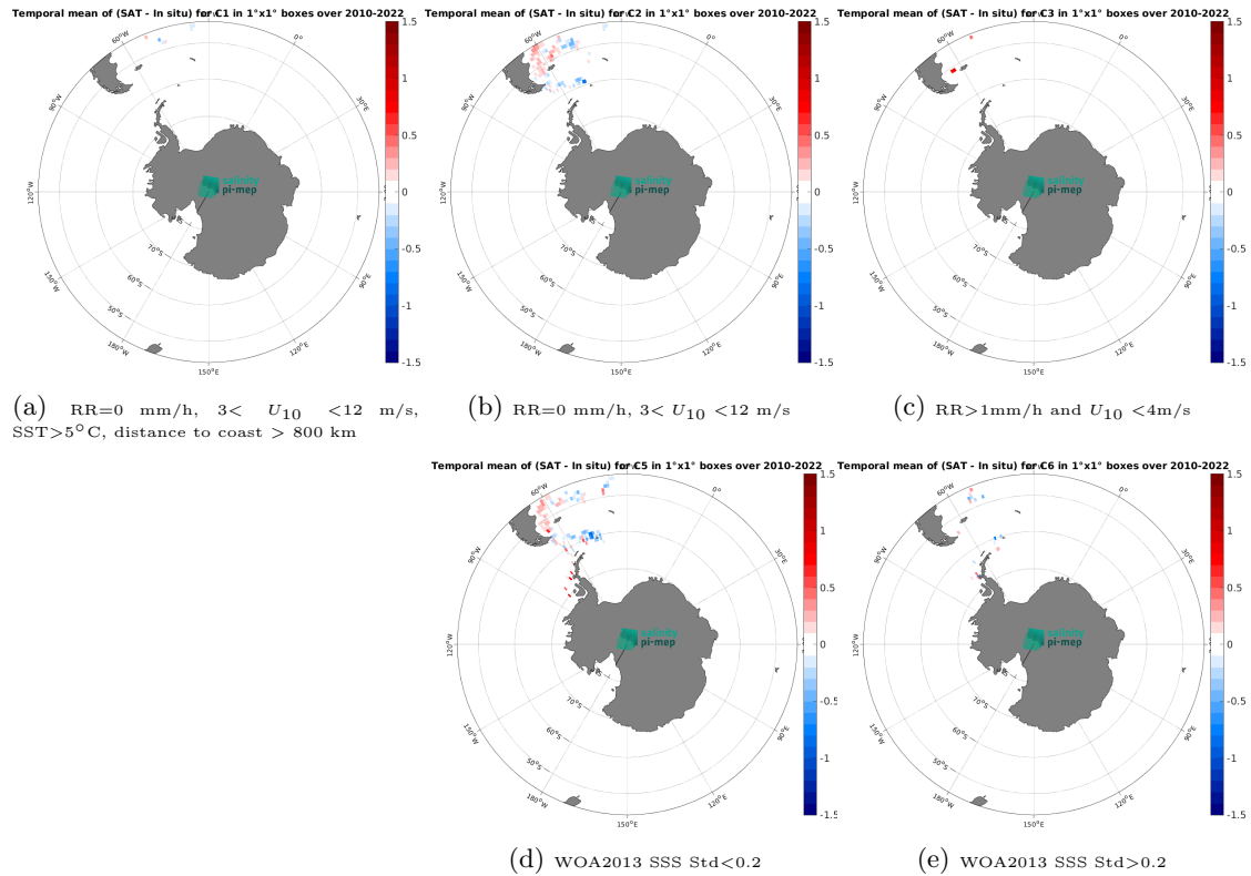
Figure 12: Temporal mean gridded over spatial boxes of size 1^{\circ}\times 1^{\circ} of \Delta\text{SSS} (CCI SSS L4 POLAR SH Merged-OI v4.4 - 7-day running (ESA) - TSG (CSIC-UTM)) for 5 different subdatasets corresponding to:RR=0 mm/h, 3 < U_{10} < 12 m/s, SST >5^{\circ}\text{C} , distance to coast > 800 km (a), RR=0 mm/h, 3 < U_{10} < 12 m/s (b), RR >1 mm/h and U_{10} < 4 m/s (c), WOA2013 SSS Std <0.2 (d), WOA2013 SSS Std >0.2 (e).
