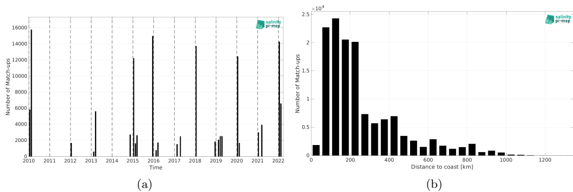
Figure 1: Number of match-ups between TSG (CSIC-UTM) and CCI SSS L4 POLAR SH Merged-OI v4.4 - 7-day running (ESA) SSS as a function of time (a) and as function of the distance to coast (b) over the Global Ocean Pi-MEP region and for the full satellite product period.
