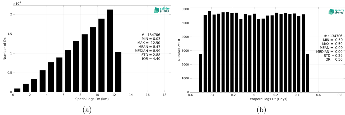
Figure 5: Histograms of the spatial (a) and temporal (b) lags between the location/time of the TSG (CSIC-UTM) measurement and the date of the corresponding CCI SSS L4 POLAR SH Merged-OI v4.4 - 7-day running (ESA) SSS pixel.
