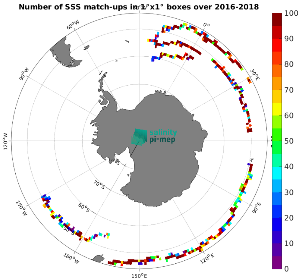
Figure 3: Number of SSS match-ups between Surface drifters SSS and the CCI SSS L4 POLAR SH Merged-OI v4.4 - 7-day running (ESA) SSS product for the Global Ocean Pi-MEP region over 1^\circ \times 1^\circ boxes and for the full satellite product period.
