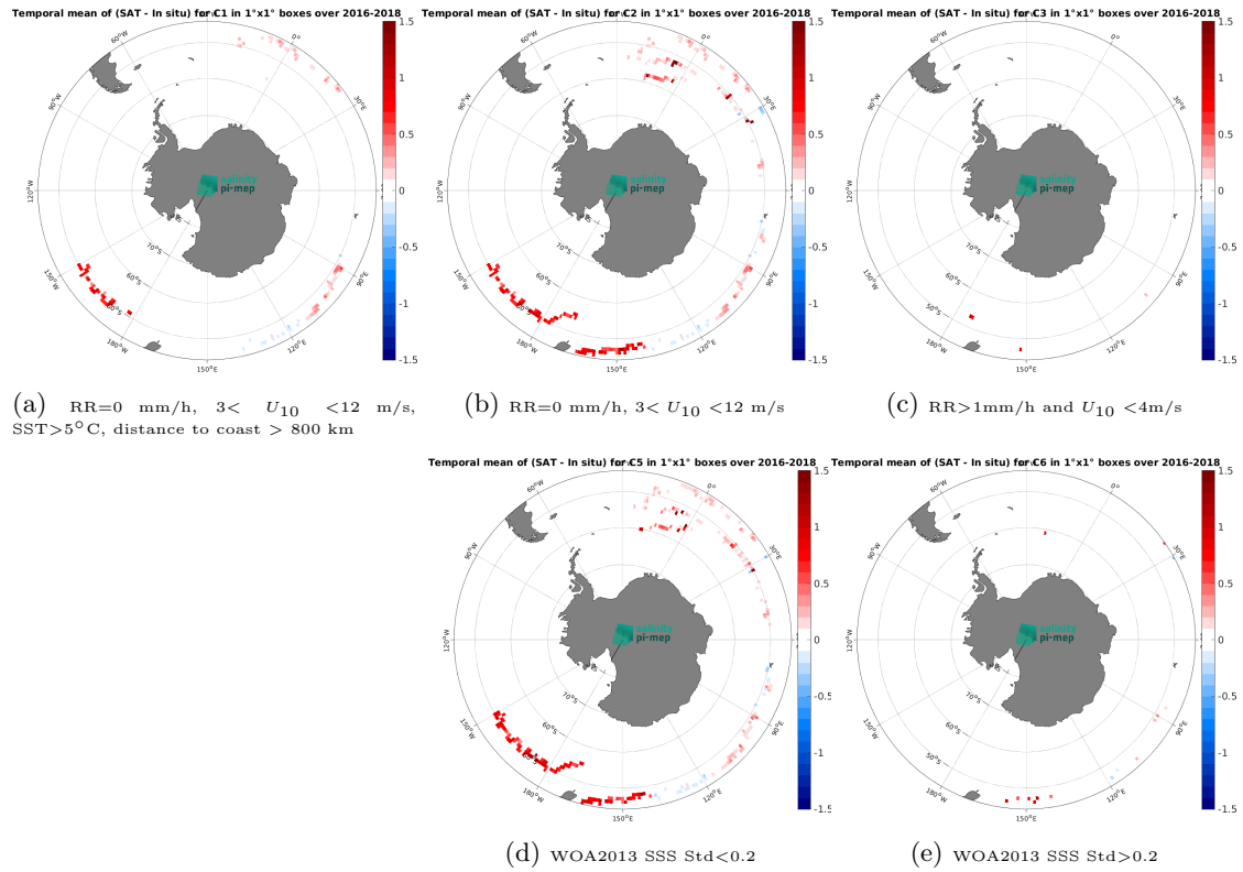
Figure 11: Temporal mean gridded over spatial boxes of size 1^{\circ}\times 1^{\circ} of \Delta\text{SSS} (CCI SSS L4 POLAR SH Merged-OI v4.4 - 7-day running (ESA) - Surface drifters) for 5 different subdatasets corresponding to:RR=0 mm/h, 3 < U_{10} < 12 m/s, SST > 5^{\circ}\text{C} , distance to coast > 800 km (a), RR=0 mm/h, 3 < U_{10} < 12 m/s (b), RR > 1 mm/h and U_{10} < 4 m/s (c), WOA2013 SSS Std < 0.2 (d), WOA2013 SSS Std > 0.2 (e).
