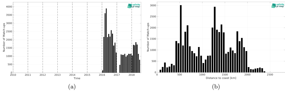
Figure 1: Number of match-ups between Surface drifters and CCI SSS L4 POLAR SH Merged-OI v4.4 - 7-day running (ESA) SSS as a function of time (a) and as function of the distance to coast (b) over the Global Ocean Pi-MEP region and for the full satellite product period.
