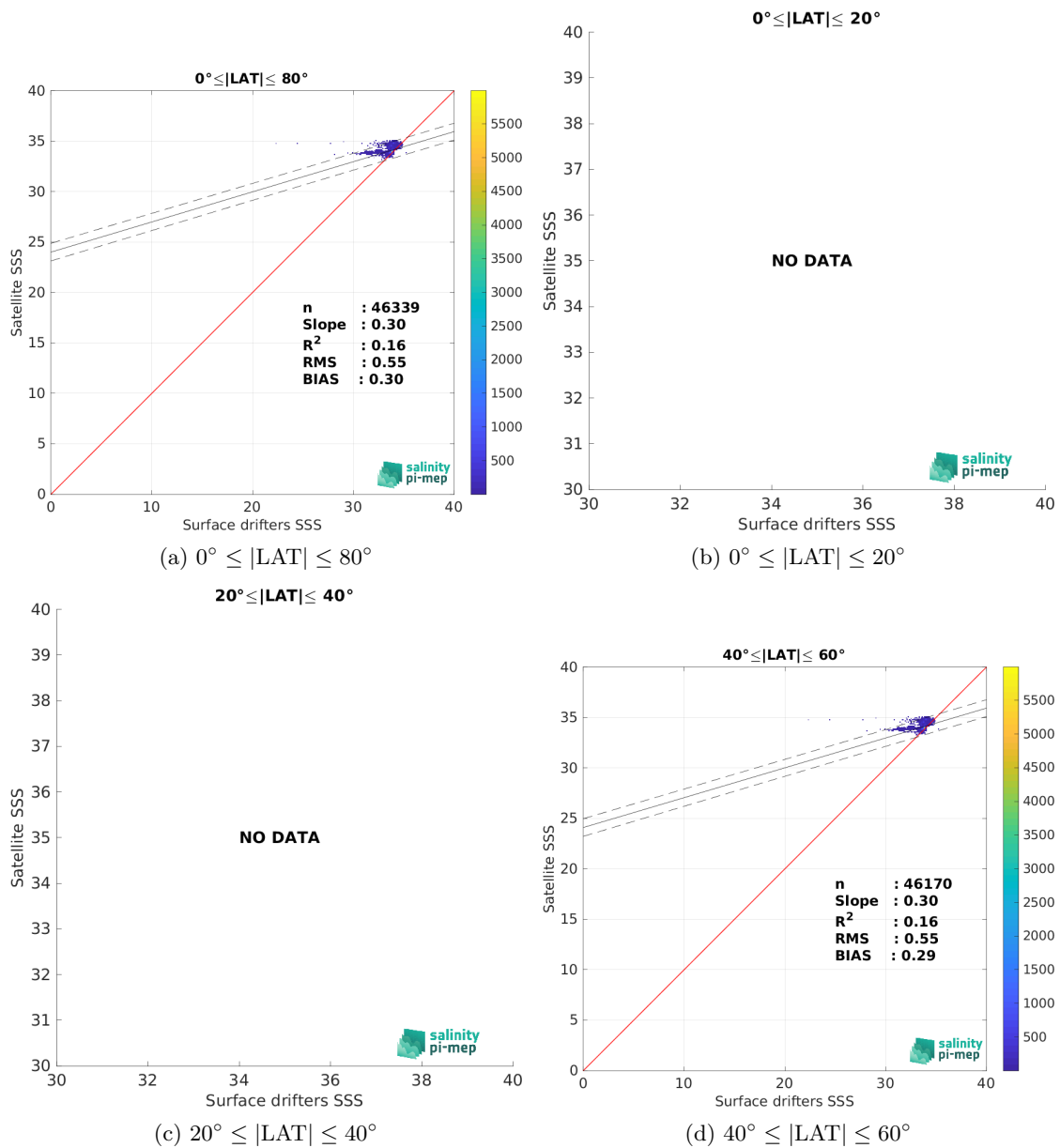
Figure 8: Contour maps of the concentration of CCI SSS L4 POLAR SH Merged-OI v4.4 - 7-day running (ESA) SSS (y-axis) versus Surface drifters SSS (x-axis) at match-up pairs for different latitude bands. For each plot, the red line shows x=y . The black thin and dashed lines indicate a linear fit through the data cloud and the \pm 95\% confidence levels, respectively. The number match-up pairs n , the slope and R^2 coefficient of the linear fit, the root mean square (RMS) and the mean bias between satellite and in situ data are indicated for each latitude band in each plots.
