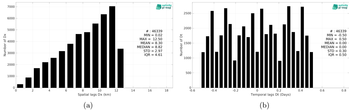
Figure 4: Histograms of the spatial (a) and temporal (b) lags between the location/time of the Surface drifters measurement and the date of the corresponding CCI SSS L4 POLAR SH Merged-OI v4.4 - 7-day running (ESA) SSS pixel.
