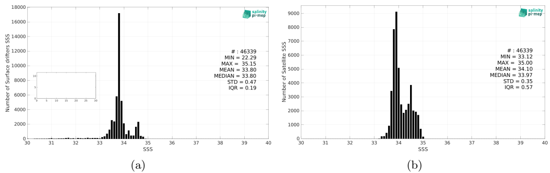
Figure 2: Histograms of SSS from Surface drifters (a) and CCI SSS L4 POLAR SH Merged-OI v4.4 - 7-day running (ESA) (b) considering all match-up pairs per bins of 0.1 over the Global Ocean Pi-MEP region and for the full satellite product period.
