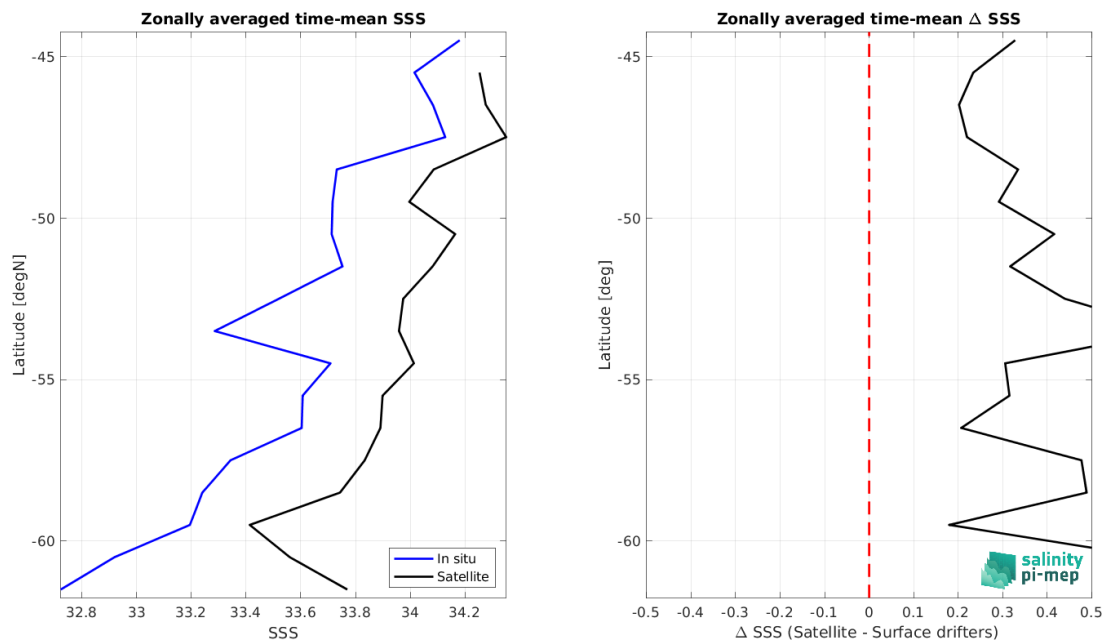
Figure 7: Left panel: Zonal mean SSS from CCI SSS L4 POLAR SH Merged-OI v4.4 - 7-day running (ESA) satellite product (black) and from Surface drifters (blue). Right panel: Zonal mean of \Delta SSS (Satellite - Surface drifters) for all the collected Pi-MEP match-up pairs estimated over the full satellite product period.
