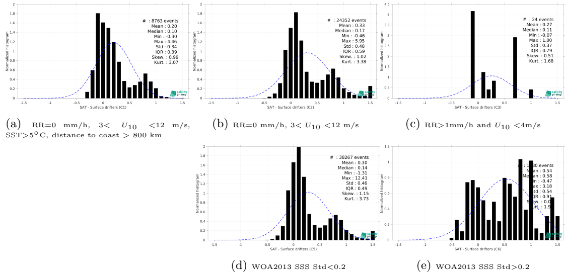
Figure 12: Normalized histogram of \Delta SSS (CCI SSS L4 POLAR SH Merged-OI v4.4 - 7-day running (ESA) - Surface drifters) for 5 different subdatasets corresponding to: RR=0 mm/h, 3 < U_{10} < 12 m/s, SST > 5°C, distance to coast > 800 km (a), RR=0 mm/h, 3 < U_{10} < 12 m/s (b), RR > 1mm/h and U_{10} < 4 m/s (c), WOA2013 SSS Std < 0.2 (d), WOA2013 SSS Std > 0.2 (e).
