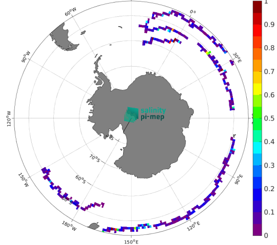
(e) MEAN( \Delta SSS) (Satellite - Surface drifters) 14
