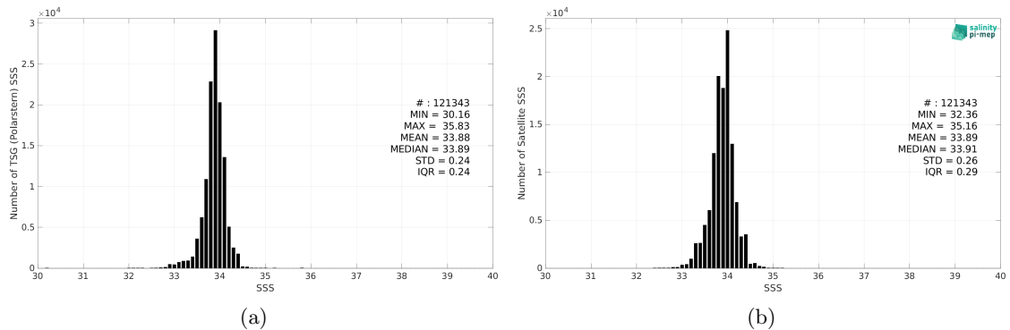
Figure 2: Histograms of SSS from TSG (Polarstern) (a) and CCI SSS L4 POLAR SH Merged-OI v4.4 - 30-day running (ESA) (b) considering all match-up pairs per bins of 0.1 over the Global Ocean Pi-MEP region and for the full satellite product period.
