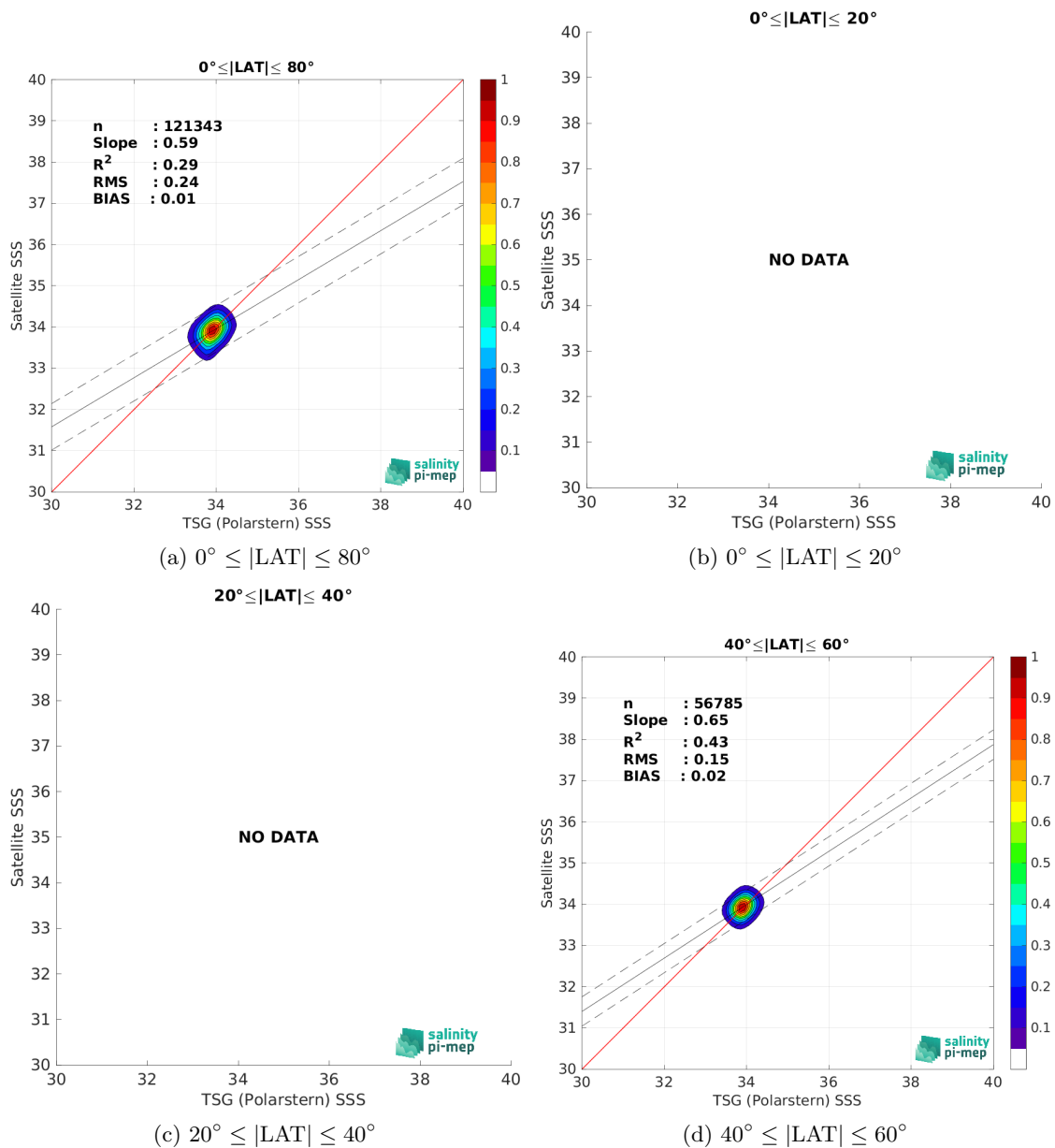
Figure 9: Contour maps of the concentration of CCI SSS L4 POLAR SH Merged-OI v4.4 - 30-day running (ESA) SSS (y-axis) versus TSG (Polarstern) SSS (x-axis) at match-up pairs for different latitude bands. For each plot, the red line shows x=y . The black thin and dashed lines indicate a linear fit through the data cloud and the \pm 95\% confidence levels, respectively. The number match-up pairs n , the slope and R^2 coefficient of the linear fit, the root mean square (RMS) and the mean bias between satellite and in situ data are indicated for each latitude band in each plots.
