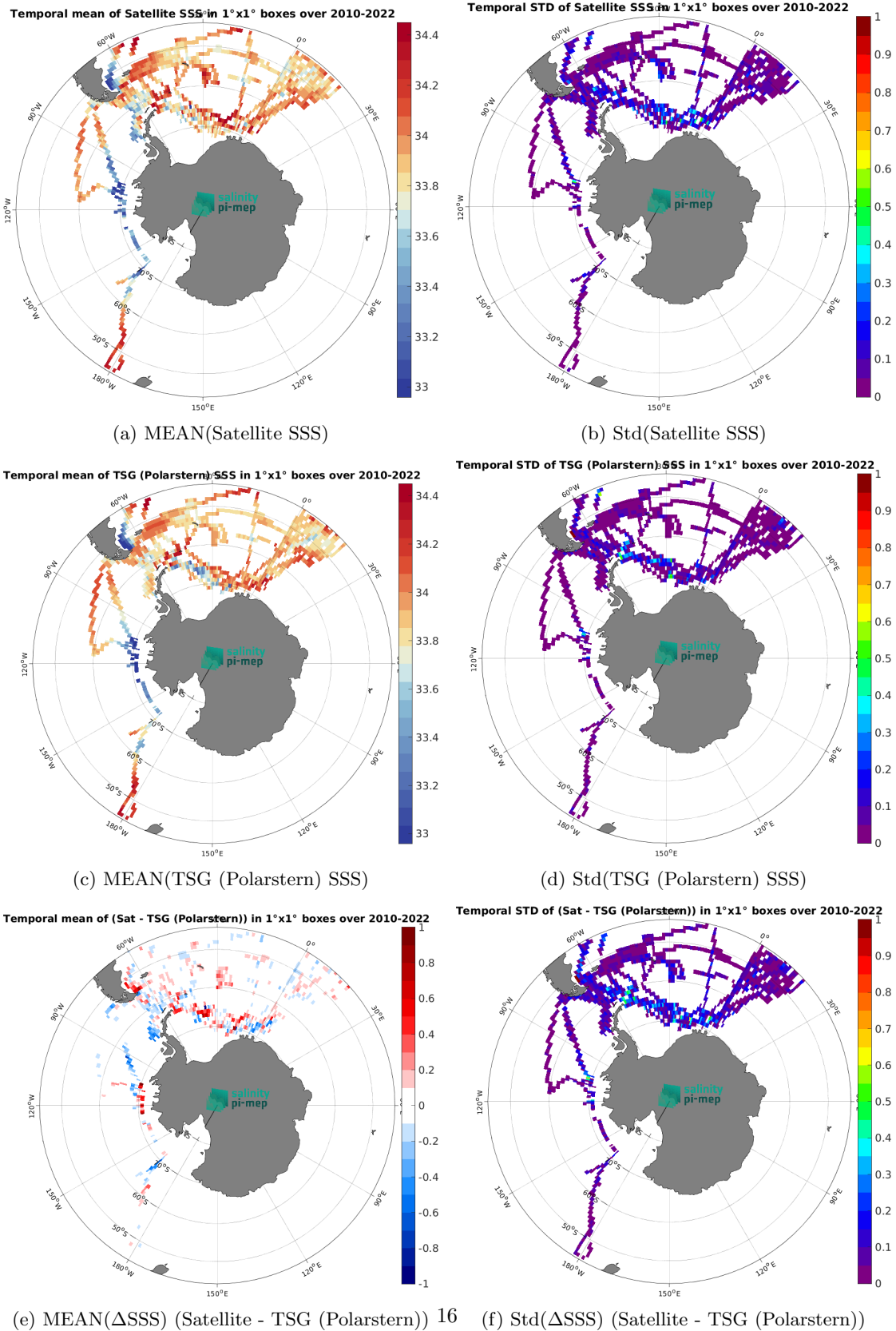
Figure 6: Temporal mean (left) and Std (right) of SSS from CCI SSS L4 POLAR SH Merged-OI v4.4 - 30-day running (ESA) (top), TSG (Polarstern) (middle), and of \Delta SSS (Satellite - TSG (Polarstern)). Only match-up pairs are used to generate these maps.
