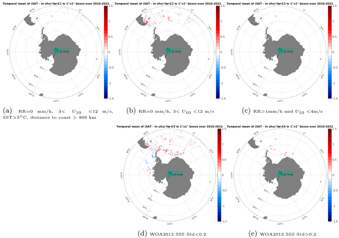
Figure 12: Temporal mean gridded over spatial boxes of size 1^{\circ}\times 1^{\circ} of \Delta\text{SSS} (CCI SSS L4 POLAR SH Merged-OI v4.4 - 30-day running (ESA) - TSG (Polarstern)) for 5 different subdatasets corresponding to:RR=0 mm/h, 3 < U_{10} < 12 m/s, SST > 5^{\circ}\text{C} , distance to coast > 800 km (a), RR=0 mm/h, 3 < U_{10} < 12 m/s (b), RR > 1 mm/h and U_{10} < 4 m/s (c), WOA2013 SSS Std < 0.2 (d), WOA2013 SSS Std > 0.2 (e).
