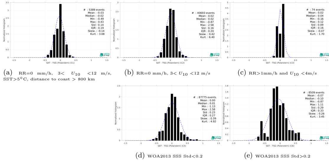
Figure 13: Normalized histogram of \Delta SSS (CCI SSS L4 POLAR SH Merged-OI v4.4 - 30-day running (ESA) - TSG (Polarstern)) for 5 different subdatasets corresponding to: RR=0 mm/h, 3 < U_{10} < 12 m/s, SST>5°C, distance to coast > 800 km (a), RR=0 mm/h, 3 < U_{10} < 12 m/s (b), RR>1mm/h and U_{10} < 4 m/s (c), WOA2013 SSS Std<0.2 (d), WOA2013 SSS Std>0.2 (e).
