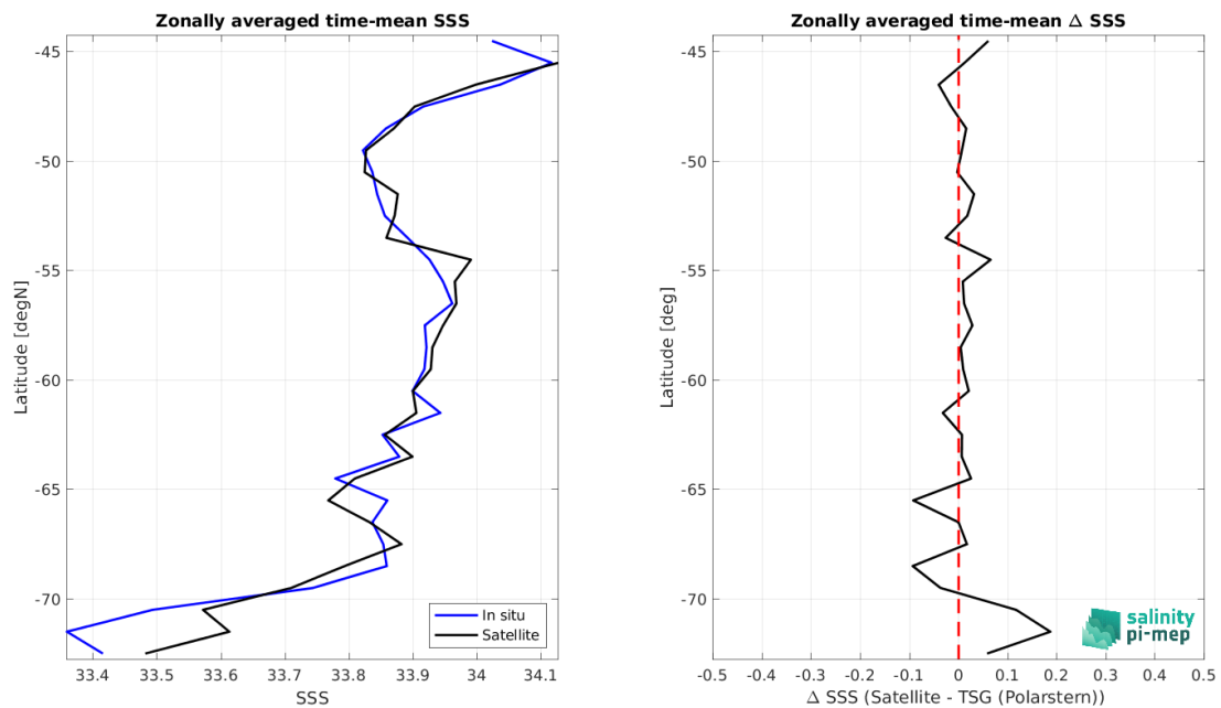
Figure 8: Left panel: Zonal mean SSS from CCI SSS L4 POLAR SH Merged-OI v4.4 - 30-day running (ESA) satellite product (black) and from TSG (Polarstern) (blue). Right panel: Zonal mean of \Delta SSS (Satellite - TSG (Polarstern)) for all the collected Pi-MEP match-up pairs estimated over the full satellite product period.
