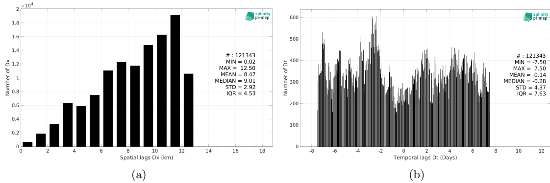
Figure 5: Histograms of the spatial (a) and temporal (b) lags between the location/time of the TSG (Polarstern) measurement and the date of the corresponding CCI SSS L4 POLAR SH Merged-OI v4.4 - 30-day running (ESA) SSS pixel.
