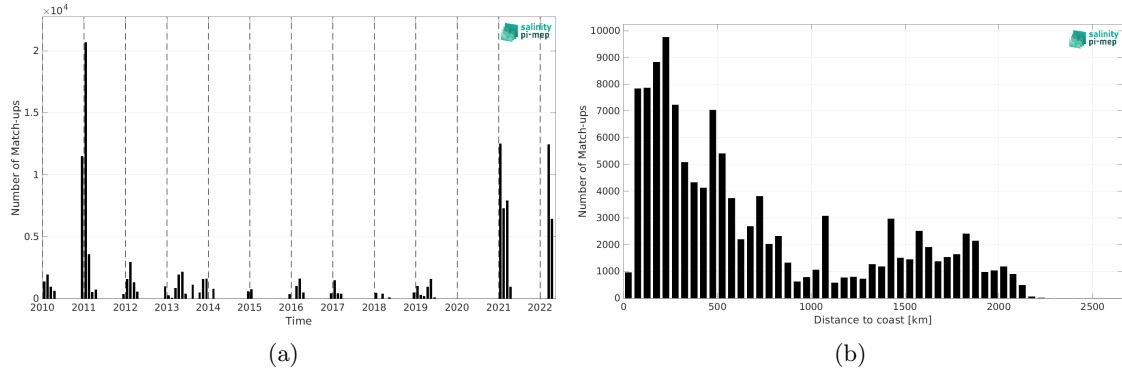
Figure 1: Number of match-ups between TSG (Polarstern) and CCI SSS L4 POLAR SH Merged-OI v4.4 - 30-day running (ESA) SSS as a function of time (a) and as function of the distance to coast (b) over the Global Ocean Pi-MEP region and for the full satellite product period.
