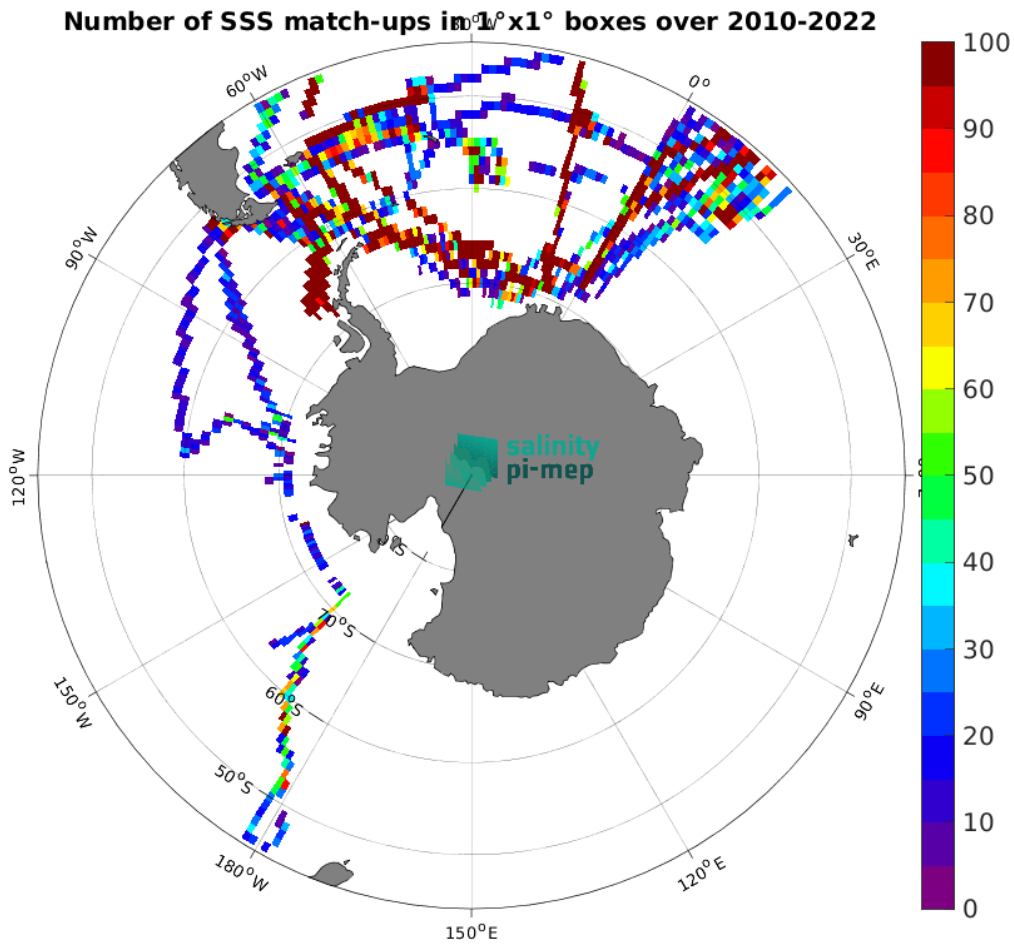
Figure 4: Number of SSS match-ups between TSG (Polarstern) SSS and the CCI SSS L4 POLAR SH Merged-OI v4.4 - 30-day running (ESA) SSS product for the Global Ocean Pi-MEP region over 1^\circ \times 1^\circ boxes and for the full satellite product period.
