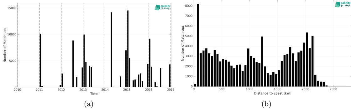
Figure 1: Number of match-ups between TSG (NCEI-0170743) and CCI SSS L4 POLAR SH Merged-OI v4.4 - 30-day running (ESA) SSS as a function of time (a) and as function of the distance to coast (b) over the Global Ocean Pi-MEP region and for the full satellite product period.
