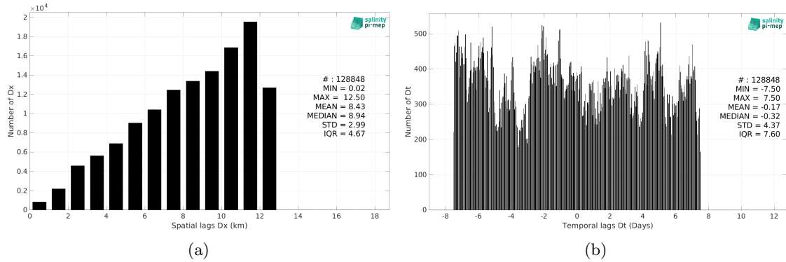
Figure 5: Histograms of the spatial (a) and temporal (b) lags between the location/time of the TSG (NCEI-0170743) measurement and the date of the corresponding CCI SSS L4 POLAR SH Merged-OI v4.4 - 30-day running (ESA) SSS pixel.
