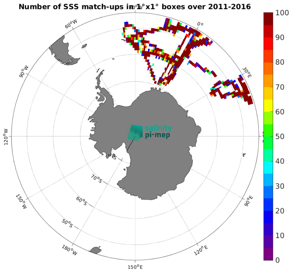
Figure 4: Number of SSS match-ups between TSG (NCEI-0170743) SSS and the CCI SSS L4 POLAR SH Merged-OI v4.4 - 30-day running (ESA) SSS product for the Global Ocean Pi-MEP region over 1^\circ \times 1^\circ boxes and for the full satellite product period.
