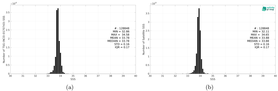
Figure 2: Histograms of SSS from TSG (NCEI-0170743) (a) and CCI SSS L4 POLAR SH Merged-OI v4.4 - 30-day running (ESA) (b) considering all match-up pairs per bins of 0.1 over the Global Ocean Pi-MEP region and for the full satellite product period.
