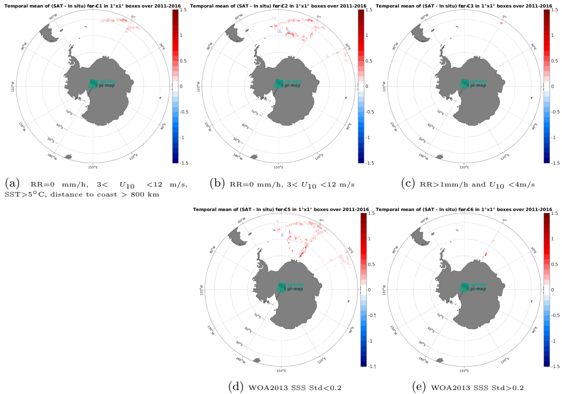
Figure 12: Temporal mean gridded over spatial boxes of size 1^{\circ}\times 1^{\circ} of \Delta\text{SSS} (CCI SSS L4 POLAR SH Merged-OI v4.4 - 30-day running (ESA) - TSG (NCEI-0170743)) for 5 different subdatasets corresponding to:RR=0 mm/h, 3 < U_{10} < 12 m/s, SST >5^{\circ}\text{C} , distance to coast > 800 km (a), RR=0 mm/h, 3 < U_{10} < 12 m/s (b), RR >1 mm/h and U_{10} < 4 m/s (c), WOA2013 SSS Std <0.2 (d), WOA2013 SSS Std >0.2 (e).
