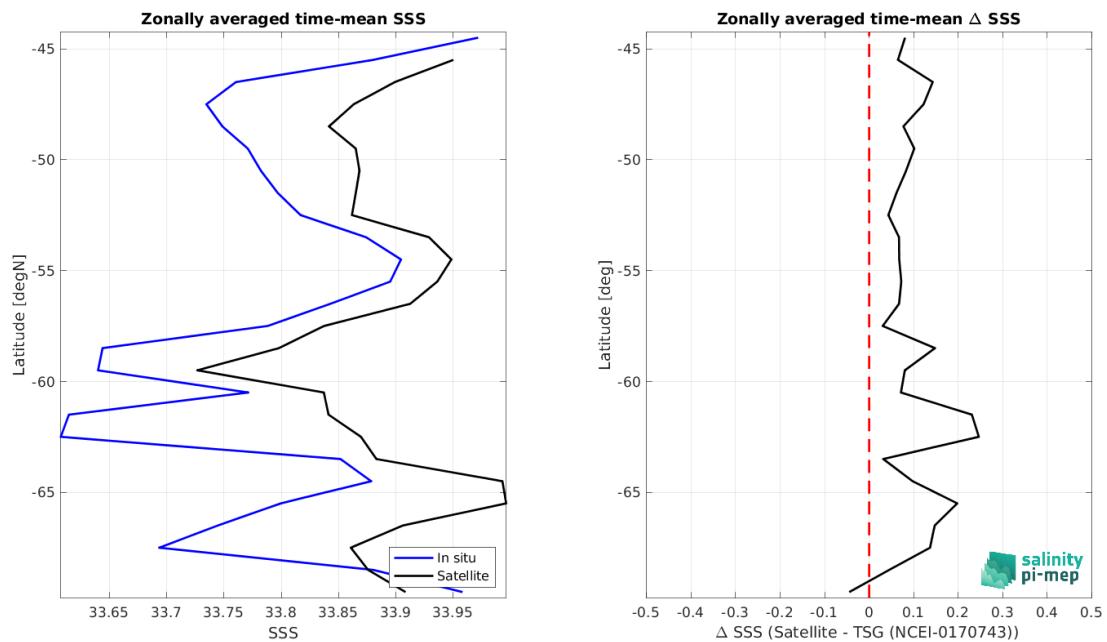
Figure 8: Left panel: Zonal mean SSS from CCI SSS L4 POLAR SH Merged-OI v4.4 - 30-day running (ESA) satellite product (black) and from TSG (NCEI-0170743) (blue). Right panel: Zonal mean of \Delta SSS (Satellite - TSG (NCEI-0170743)) for all the collected Pi-MEP match-up pairs estimated over the full satellite product period.
