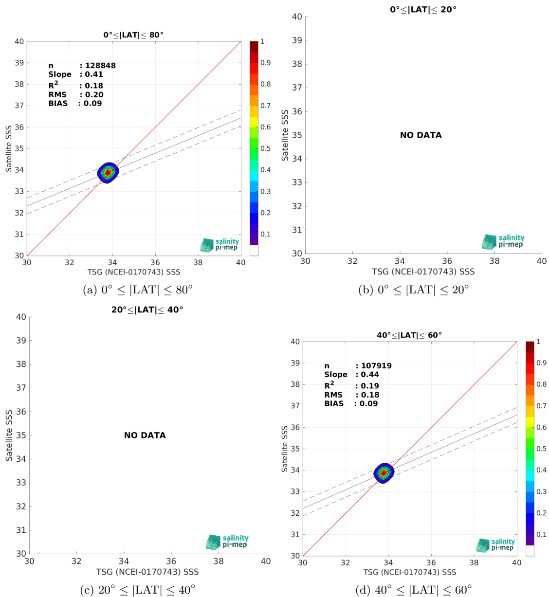
Figure 9: Contour maps of the concentration of CCI SSS L4 POLAR SH Merged-OI v4.4 - 30-day running (ESA) SSS (y-axis) versus TSG (NCEI-0170743) SSS (x-axis) at match-up pairs for different latitude bands. For each plot, the red line shows x=y . The black thin and dashed lines indicate a linear fit through the data cloud and the \pm 95\% confidence levels, respectively. The number match-up pairs n , the slope and R^2 coefficient of the linear fit, the root mean square (RMS) and the mean bias between satellite and in situ data are indicated for each latitude band in each plots.
