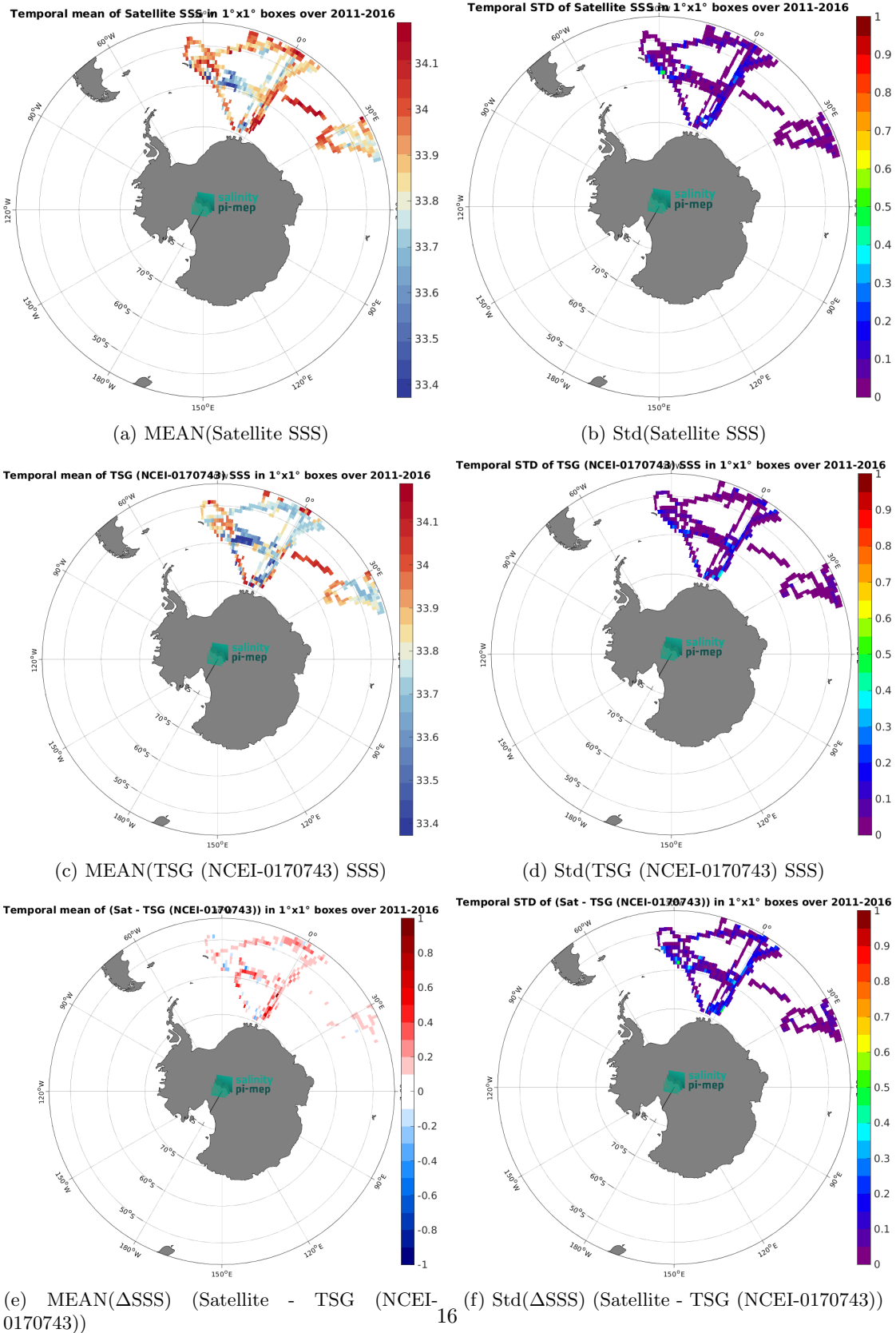
Figure 6: Temporal mean (left) and Std (right) of SSS from CCI SSS L4 POLAR SH Merged-OI v4.4 - 30-day running (ESA) (top), TSG (NCEI-0170743) (middle), and of \Delta SSS (Satellite - TSG (NCEI-0170743)). Only match-up pairs are used to generate these maps.
