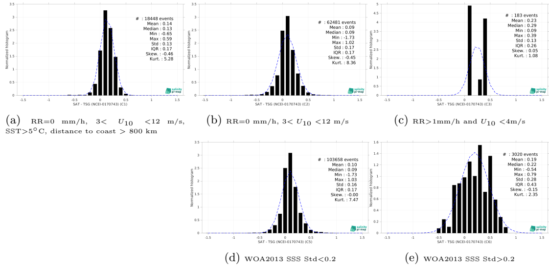
Figure 13: Normalized histogram of \Delta SSS (CCI SSS L4 POLAR SH Merged-OI v4.4 - 30-day running (ESA) - TSG (NCEI-0170743)) for 5 different subdatasets corresponding to: RR=0 mm/h, 3 < U_{10} < 12 m/s, SST > 5°C, distance to coast > 800 km (a), RR=0 mm/h, 3 < U_{10} < 12 m/s (b), RR > 1mm/h and U_{10} < 4 m/s (c), WOA2013 SSS Std < 0.2 (d), WOA2013 SSS Std > 0.2 (e).
