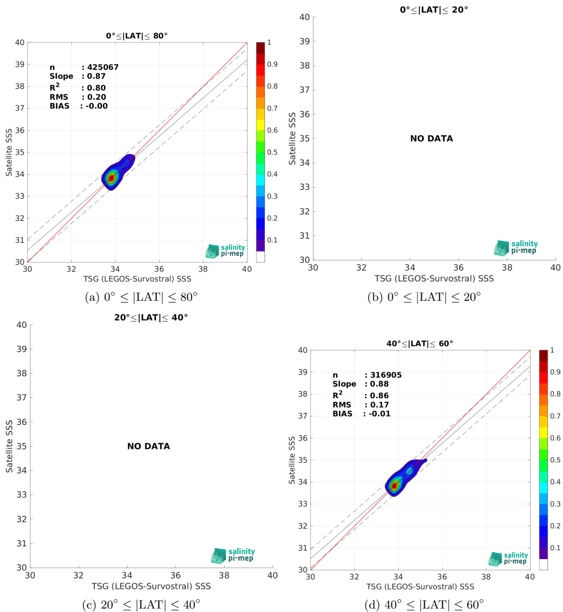
Figure 9: Contour maps of the concentration of CCI SSS L4 POLAR SH Merged-OI v4.4 - 30-day running (ESA) SSS (y-axis) versus TSG (LEGOS-Survostral) SSS (x-axis) at match-up pairs for different latitude bands. For each plot, the red line shows x=y . The black thin and dashed lines indicate a linear fit through the data cloud and the \pm 95\% confidence levels, respectively. The number match-up pairs n , the slope and R^2 coefficient of the linear fit, the root mean square (RMS) and the mean bias between satellite and in situ data are indicated for each latitude band in each plots.
