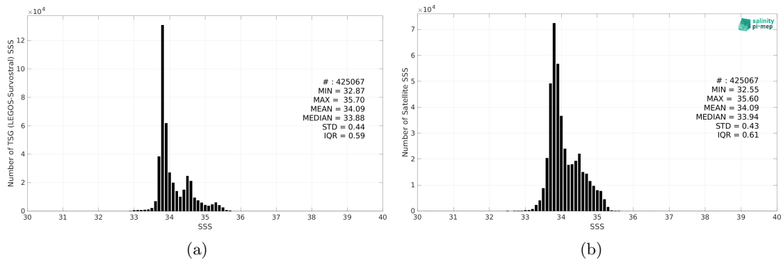
Figure 2: Histograms of SSS from TSG (LEGOS-Survostral) (a) and CCI SSS L4 POLAR SH Merged-OI v4.4 - 30-day running (ESA) (b) considering all match-up pairs per bins of 0.1 over the Global Ocean Pi-MEP region and for the full satellite product period.
