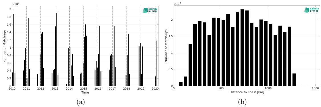
Figure 1: Number of match-ups between TSG (LEGOS-Survostral) and CCI SSS L4 POLAR SH Merged-OI v4.4 - 30-day running (ESA) SSS as a function of time (a) and as function of the distance to coast (b) over the Global Ocean Pi-MEP region and for the full satellite product period.
