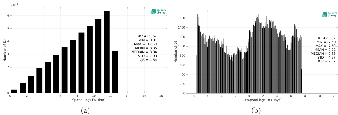
Figure 5: Histograms of the spatial (a) and temporal (b) lags between the location/time of the TSG (LEGOS-Survostral) measurement and the date of the corresponding CCI SSS L4 POLAR SH Merged-OI v4.4 - 30-day running (ESA) SSS pixel.
