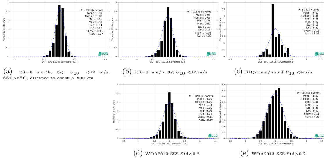
Figure 13: Normalized histogram of \Delta SSS (CCI SSS L4 POLAR SH Merged-OI v4.4 - 30-day running (ESA) - TSG (LEGOS-Survostral)) for 5 different subdatasets corresponding to: RR=0 mm/h, 3 < U_{10} < 12 m/s, SST>5°C, distance to coast > 800 km (a), RR=0 mm/h, 3 < U_{10} < 12 m/s (b), RR>1mm/h and U_{10} < 4 m/s (c), WOA2013 SSS Std<0.2 (d), WOA2013 SSS Std>0.2 (e).
