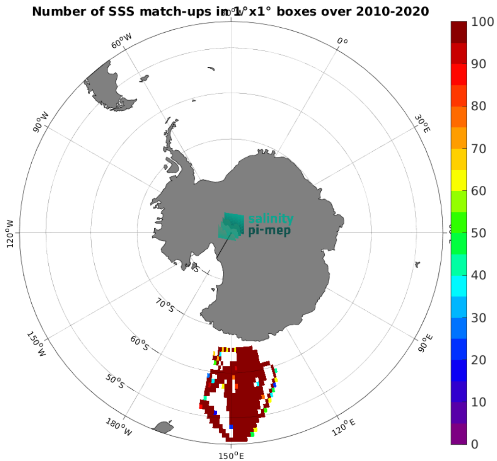
Figure 4: Number of SSS match-ups between TSG (LEGOS-Survostral) SSS and the CCI SSS L4 POLAR SH Merged-OI v4.4 - 30-day running (ESA) SSS product for the Global Ocean Pi-MEP region over 1^\circ \times 1^\circ boxes and for the full satellite product period.
