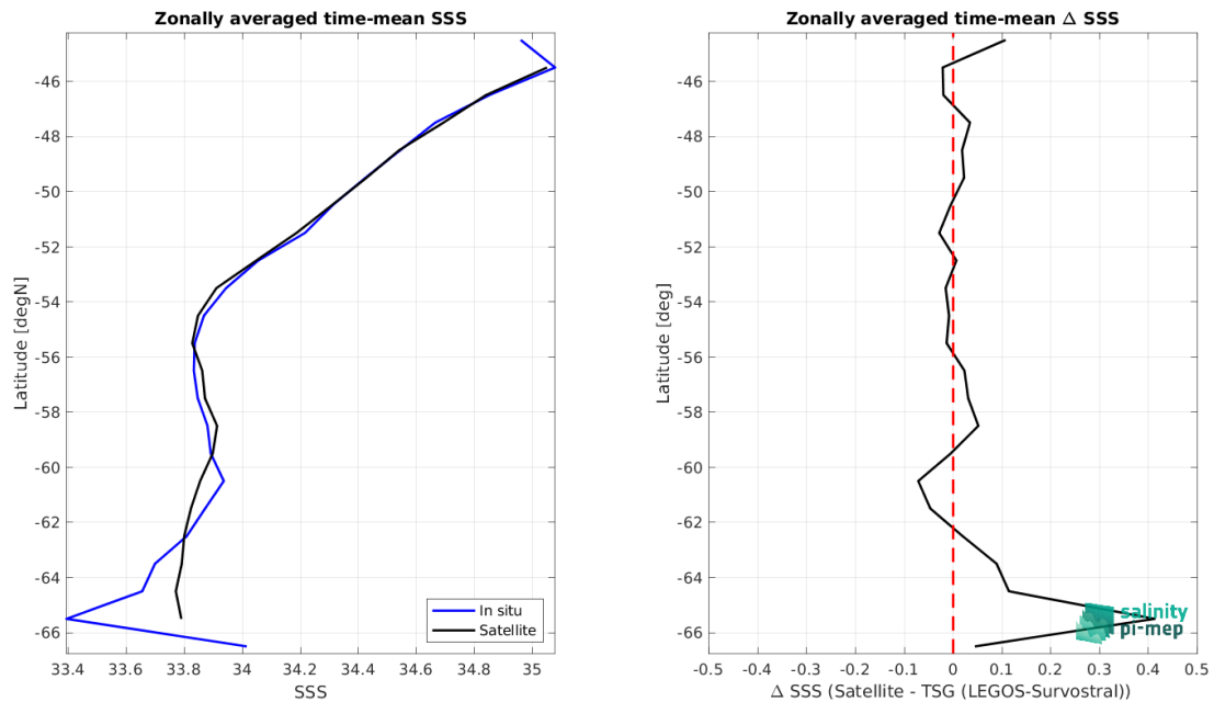
Figure 8: Left panel: Zonal mean SSS from CCI SSS L4 POLAR SH Merged-OI v4.4 - 30-day running (ESA) satellite product (black) and from TSG (LEGOS-Survostral) (blue). Right panel: Zonal mean of \Delta SSS (Satellite - TSG (LEGOS-Survostral)) for all the collected Pi-MEP match-up pairs estimated over the full satellite product period.
