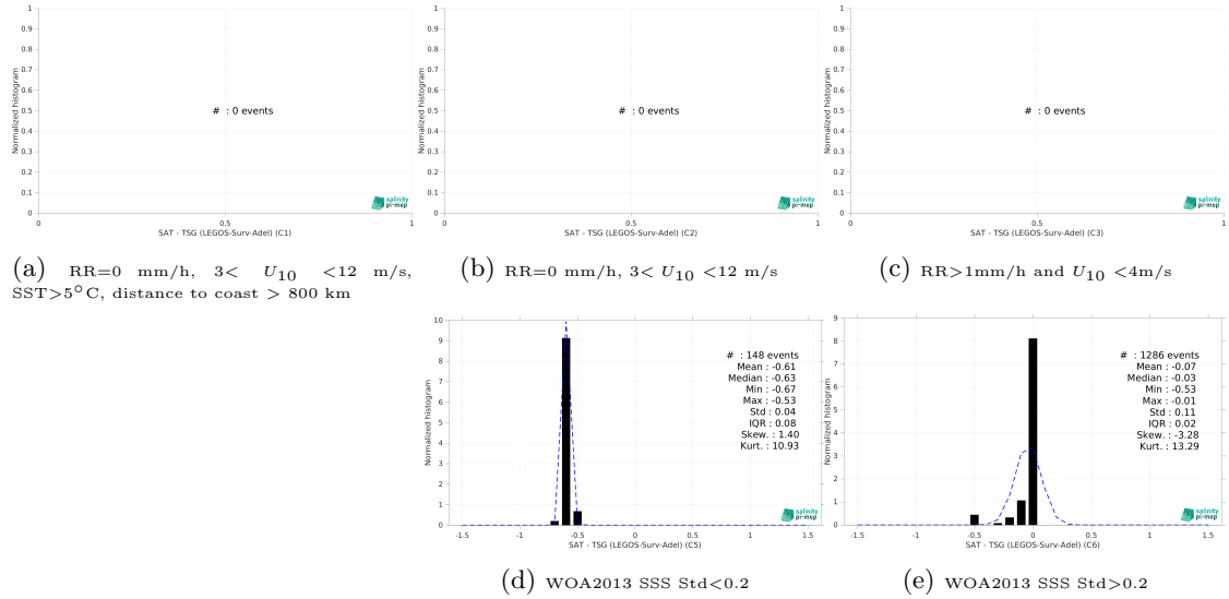
Figure 13: Normalized histogram of \Delta SSS (CCI SSS L4 POLAR SH Merged-OI v4.4 - 30-day running (ESA) - TSG (LEGOS-Surv-Adel)) for 5 different subdatasets corresponding to: RR=0 mm/h, 3 < U_{10} < 12 m/s, SST>5°C, distance to coast > 800 km (a), RR=0 mm/h, 3 < U_{10} < 12 m/s (b), RR>1mm/h and U_{10} < 4 m/s (c), WOA2013 SSS Std<0.2 (d), WOA2013 SSS Std>0.2 (e).
