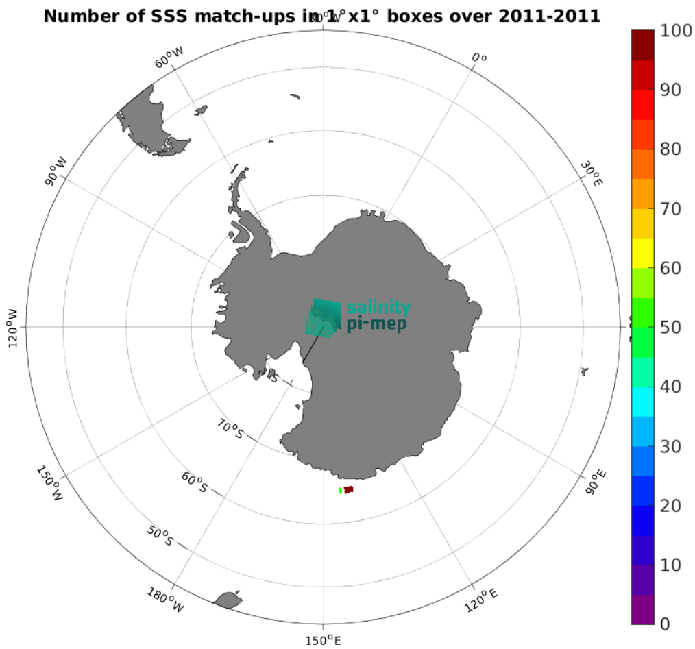
Figure 4: Number of SSS match-ups between TSG (LEGOS-Surv-Adel) SSS and the CCI SSS L4 POLAR SH Merged-OI v4.4 - 30-day running (ESA) SSS product for the Global Ocean Pi-MEP region over 1^\circ \times 1^\circ boxes and for the full satellite product period.
