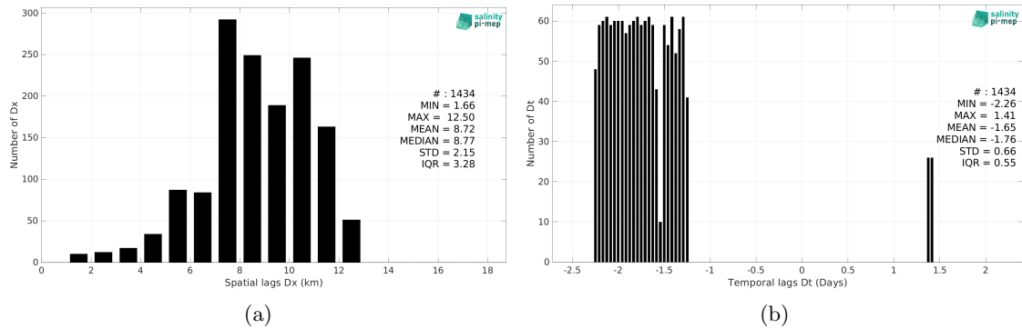
Figure 5: Histograms of the spatial (a) and temporal (b) lags between the location/time of the TSG (LEGOS-Surv-Adel) measurement and the date of the corresponding CCI SSS L4 POLAR SH Merged-OI v4.4 - 30-day running (ESA) SSS pixel.
