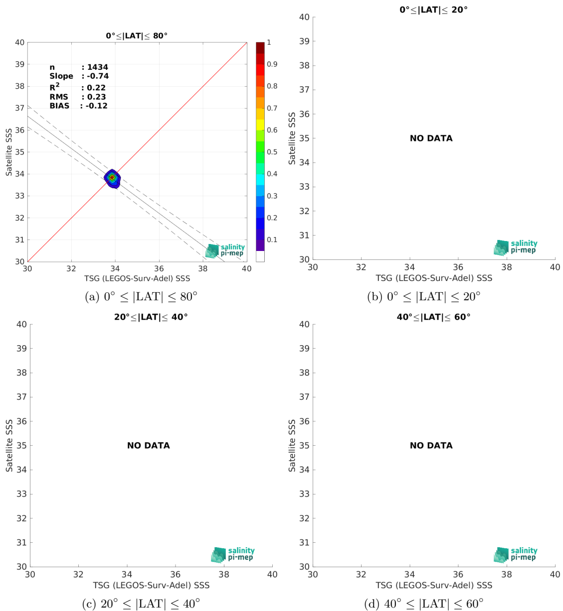
Figure 9: Contour maps of the concentration of CCI SSS L4 POLAR SH Merged-OI v4.4 - 30-day running (ESA) SSS (y-axis) versus TSG (LEGOS-Surv-Adel) SSS (x-axis) at match-up pairs for different latitude bands. For each plot, the red line shows x=y . The black thin and dashed lines indicate a linear fit through the data cloud and the \pm 95\% confidence levels, respectively. The number match-up pairs n , the slope and R^2 coefficient of the linear fit, the root mean square (RMS) and the mean bias between satellite and in situ data are indicated for each latitude band in each plots.
