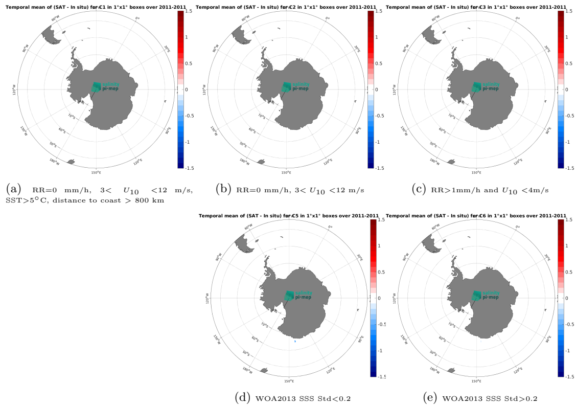
Figure 12: Temporal mean gridded over spatial boxes of size 1^\circ \times 1^\circ of \Delta SSS (CCI SSS L4 POLAR SH Merged-OI v4.4 - 30-day running (ESA) - TSG (LEGOS-Surv-Adel)) for 5 different subdatasets corresponding to:RR=0 mm/h, 3 < U_{10} < 12 m/s, SST>5°C, distance to coast > 800 km (a), RR=0 mm/h, 3 < U_{10} < 12 m/s (b), RR>1mm/h and U_{10} < 4 m/s (c), WOA2013 SSS Std<0.2 (d), WOA2013 SSS Std>0.2 (e).
