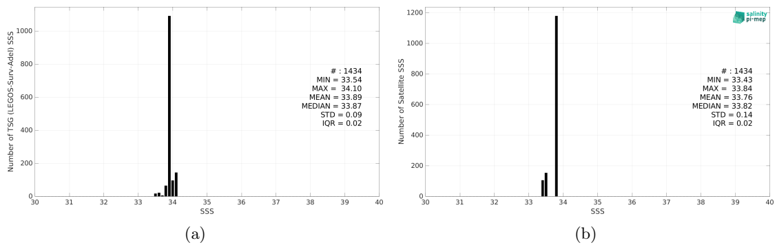
Figure 2: Histograms of SSS from TSG (LEGOS-Surv-Adel) (a) and CCI SSS L4 POLAR SH Merged-OI v4.4 - 30-day running (ESA) (b) considering all match-up pairs per bins of 0.1 over the Global Ocean Pi-MEP region and for the full satellite product period.
