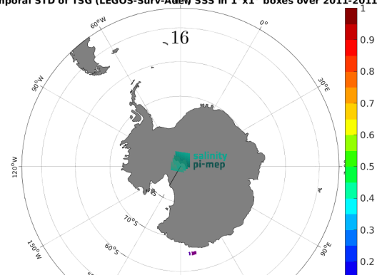
Temporal STD of TSG (LEGOS-Surv-Adel) SSS in 1°x1° boxes over 2011-2011
