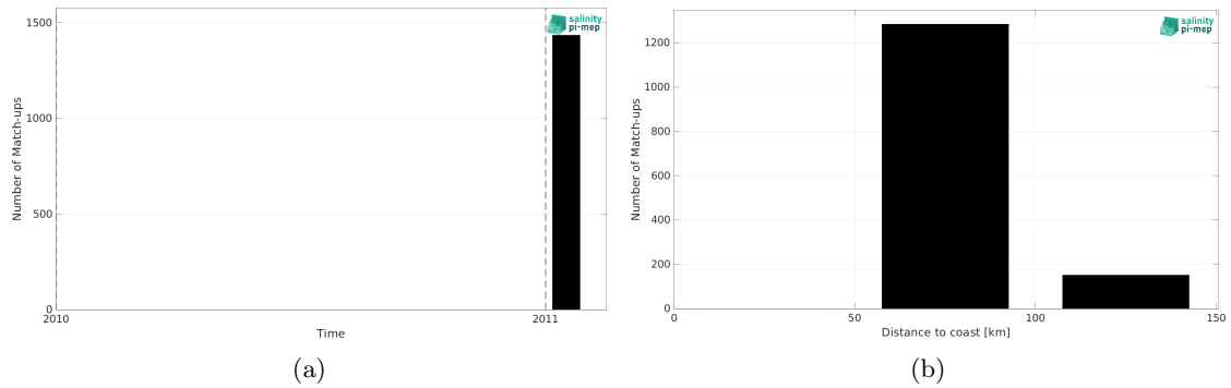
Figure 1: Number of match-ups between TSG (LEGOS-Surv-Adel) and CCI SSS L4 POLAR SH Merged-OI v4.4 - 30-day running (ESA) SSS as a function of time (a) and as function of the distance to coast (b) over the Global Ocean Pi-MEP region and for the full satellite product period.
