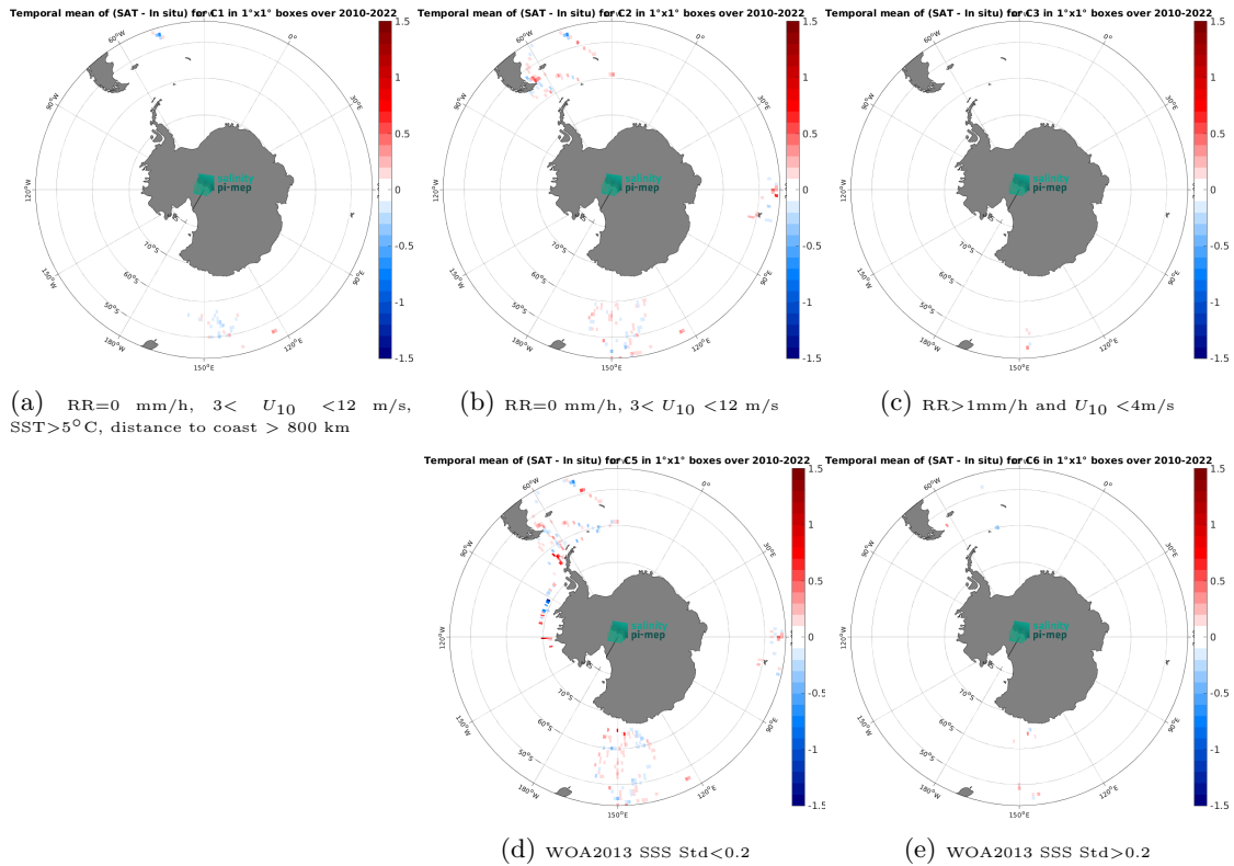
Figure 12: Temporal mean gridded over spatial boxes of size 1^{\circ}\times 1^{\circ} of \Delta\text{SSS} (CCI SSS L4 POLAR SH Merged-OI v4.4 - 30-day running (ESA) - TSG (LEGOS-DM)) for 5 different subdatasets corresponding to:RR=0 mm/h, 3 < U_{10} < 12 m/s, SST >5^{\circ}\text{C} , distance to coast > 800 km (a), RR=0 mm/h, 3 < U_{10} < 12 m/s (b), RR >1 mm/h and U_{10} < 4 m/s (c), WOA2013 SSS Std <0.2 (d), WOA2013 SSS Std >0.2 (e).
