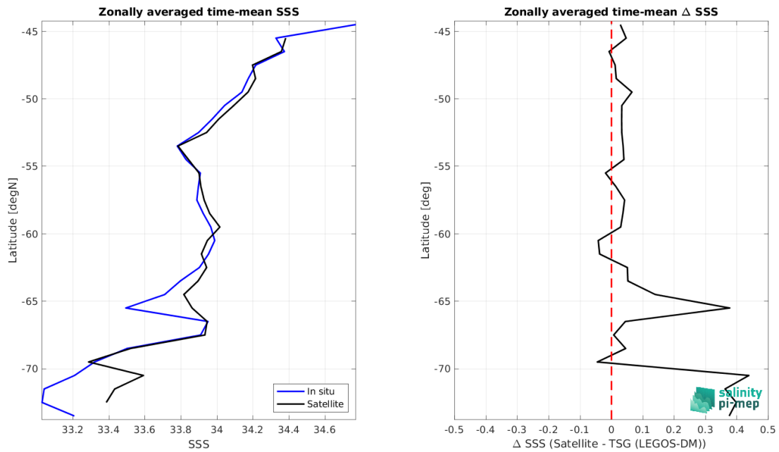
Figure 8: Left panel: Zonal mean SSS from CCI SSS L4 POLAR SH Merged-OI v4.4 - 30-day running (ESA) satellite product (black) and from TSG (LEGOS-DM) (blue). Right panel: Zonal mean of \Delta SSS (Satellite - TSG (LEGOS-DM)) for all the collected Pi-MEP match-up pairs estimated over the full satellite product period.
