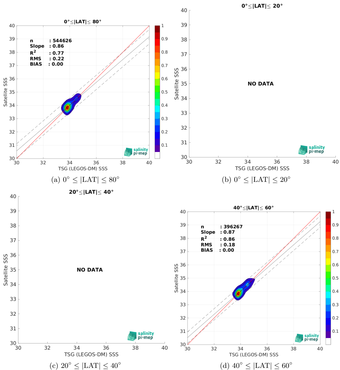
Figure 9: Contour maps of the concentration of CCI SSS L4 POLAR SH Merged-OI v4.4 - 30-day running (ESA) SSS (y-axis) versus TSG (LEGOS-DM) SSS (x-axis) at match-up pairs for different latitude bands. For each plot, the red line shows x=y . The black thin and dashed lines indicate a linear fit through the data cloud and the \pm 95\% confidence levels, respectively. The number match-up pairs n , the slope and R^2 coefficient of the linear fit, the root mean square (RMS) and the mean bias between satellite and in situ data are indicated for each latitude band in each plots.
