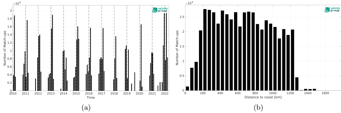
Figure 1: Number of match-ups between TSG (LEGOS-DM) and CCI SSS L4 POLAR SH Merged-OI v4.4 - 30-day running (ESA) SSS as a function of time (a) and as function of the distance to coast (b) over the Global Ocean Pi-MEP region and for the full satellite product period.
