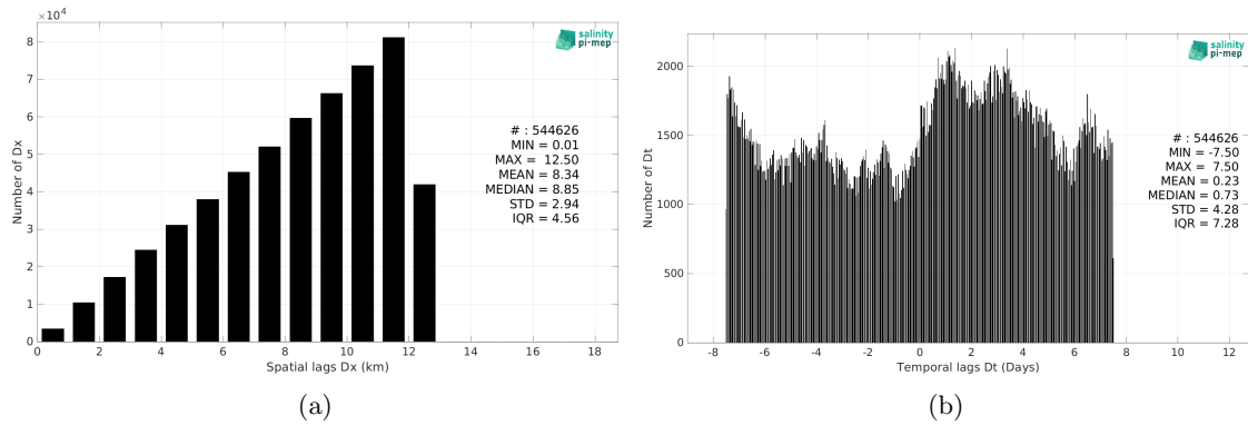
Figure 5: Histograms of the spatial (a) and temporal (b) lags between the location/time of the TSG (LEGOS-DM) measurement and the date of the corresponding CCI SSS L4 POLAR SH Merged-OI v4.4 - 30-day running (ESA) SSS pixel.
