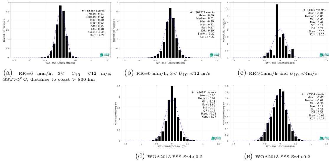
Figure 13: Normalized histogram of \Delta SSS (CCI SSS L4 POLAR SH Merged-OI v4.4 - 30-day running (ESA) - TSG (LEGOS-DM)) for 5 different subdatasets corresponding to: RR=0 mm/h, 3 < U_{10} < 12 m/s, SST>5°C, distance to coast > 800 km (a), RR=0 mm/h, 3 < U_{10} < 12 m/s (b), RR>1mm/h and U_{10} < 4 m/s (c), WOA2013 SSS Std<0.2 (d), WOA2013 SSS Std>0.2 (e).
