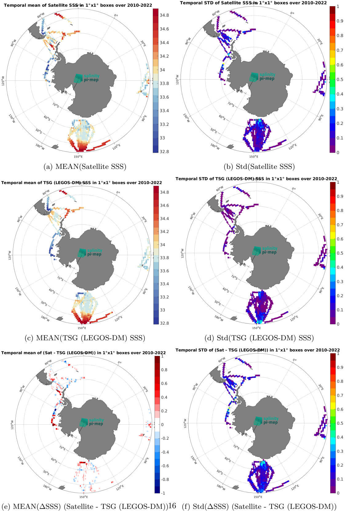
Figure 6: Temporal mean (left) and Std (right) of SSS from CCI SSS L4 POLAR SH Merged-OI v4.4 - 30-day running (ESA) (top), TSG (LEGOS-DM) (middle), and of \Delta SSS (Satellite - TSG (LEGOS-DM)). Only match-up pairs are used to generate these maps.
