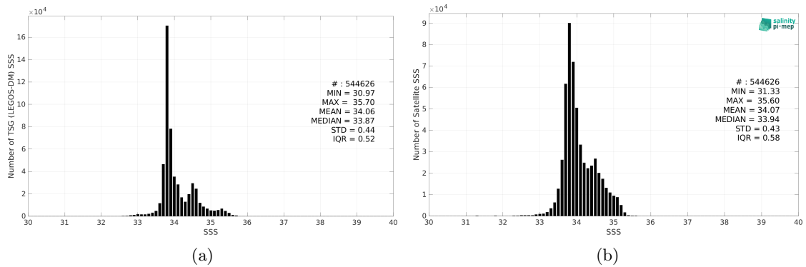
Figure 2: Histograms of SSS from TSG (LEGOS-DM) (a) and CCI SSS L4 POLAR SH Merged-OI v4.4 - 30-day running (ESA) (b) considering all match-up pairs per bins of 0.1 over the Global Ocean Pi-MEP region and for the full satellite product period.
