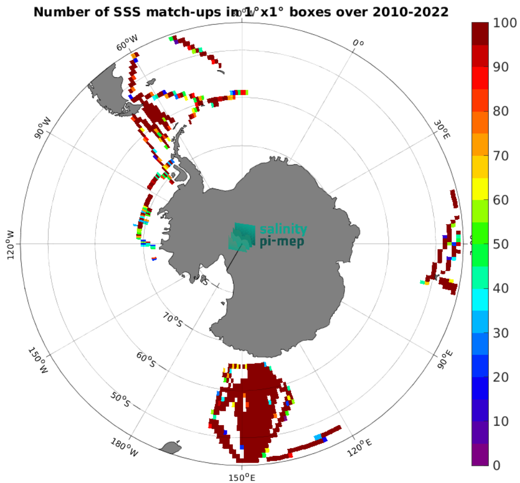
Figure 4: Number of SSS match-ups between TSG (LEGOS-DM) SSS and the CCI SSS L4 POLAR SH Merged-OI v4.4 - 30-day running (ESA) SSS product for the Global Ocean Pi-MEP region over 1^\circ \times 1^\circ boxes and for the full satellite product period.
