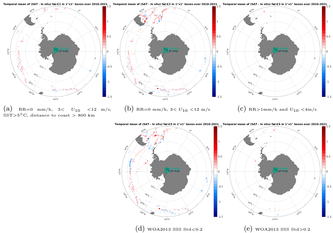
Figure 12: Temporal mean gridded over spatial boxes of size 1^\circ \times 1^\circ of \Delta SSS (CCI SSS L4 POLAR SH Merged-OI v4.4 - 30-day running (ESA) - TSG (GOSUD-Sailing-ship)) for 5 different subdatasets corresponding to: RR=0 mm/h, 3 < U_{10} < 12 m/s, SST>5°C, distance to coast > 800 km (a), RR=0 mm/h, 3 < U_{10} < 12 m/s (b), RR>1mm/h and U_{10} < 4 m/s (c), WOA2013 SSS Std<0.2 (d), WOA2013 SSS Std>0.2 (e).
