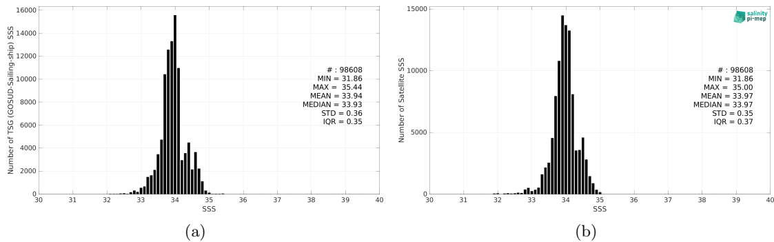
Figure 2: Histograms of SSS from TSG (GOSUD-Sailing-ship) (a) and CCI SSS L4 POLAR SH Merged-OI v4.4 - 30-day running (ESA) (b) considering all match-up pairs per bins of 0.1 over the Global Ocean Pi-MEP region and for the full satellite product period.
