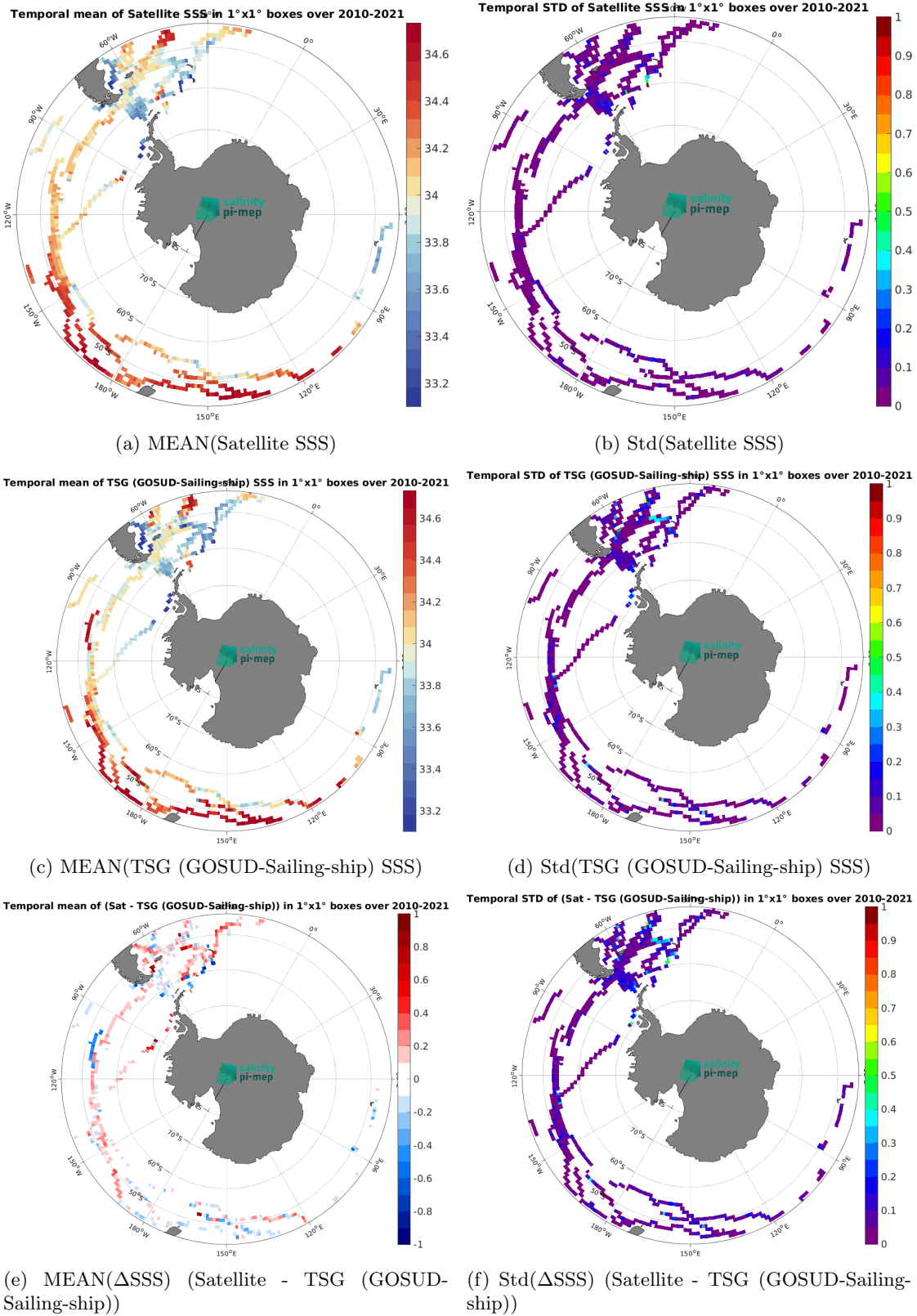
Figure 6: Temporal mean (left) and Std (right) of SSS from CCI SSS L4 POLAR SH Merged-OI v4.4 - 30-day running (ESA) (top), TSG (GOSUD-Sailing-ship) (middle), and of \Delta SSS (Satellite - TSG (GOSUD-Sailing-ship)). Only match-up pairs are used to generate these maps.
