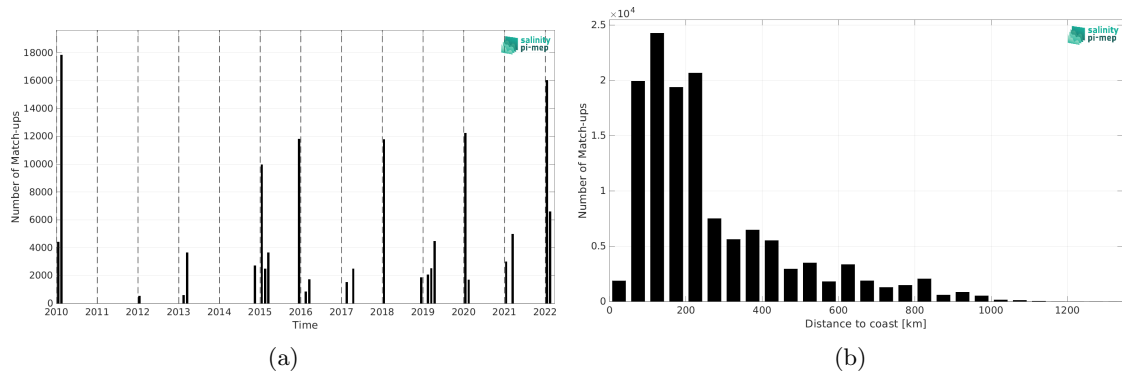
Figure 1: Number of match-ups between TSG (CSIC-UTM) and CCI SSS L4 POLAR SH Merged-OI v4.4 - 30-day running (ESA) SSS as a function of time (a) and as function of the distance to coast (b) over the Global Ocean Pi-MEP region and for the full satellite product period.
