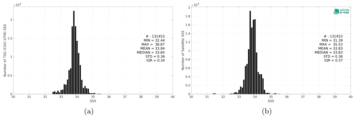
Figure 2: Histograms of SSS from TSG (CSIC-UTM) (a) and CCI SSS L4 POLAR SH Merged-OI v4.4 - 30-day running (ESA) (b) considering all match-up pairs per bins of 0.1 over the Global Ocean Pi-MEP region and for the full satellite product period.
