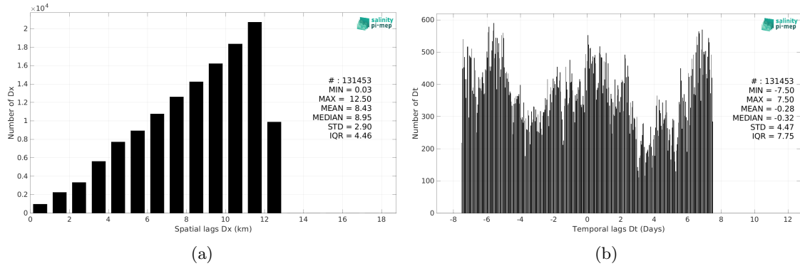
Figure 5: Histograms of the spatial (a) and temporal (b) lags between the location/time of the TSG (CSIC-UTM) measurement and the date of the corresponding CCI SSS L4 POLAR SH Merged-OI v4.4 - 30-day running (ESA) SSS pixel.
