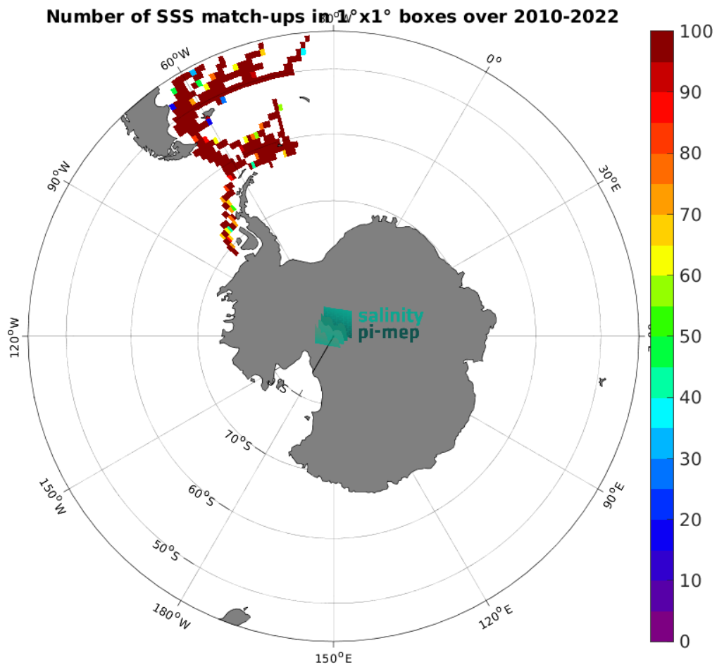
Figure 4: Number of SSS match-ups between TSG (CSIC-UTM) SSS and the CCI SSS L4 POLAR SH Merged-OI v4.4 - 30-day running (ESA) SSS product for the Global Ocean Pi-MEP region over 1^\circ \times 1^\circ boxes and for the full satellite product period.
