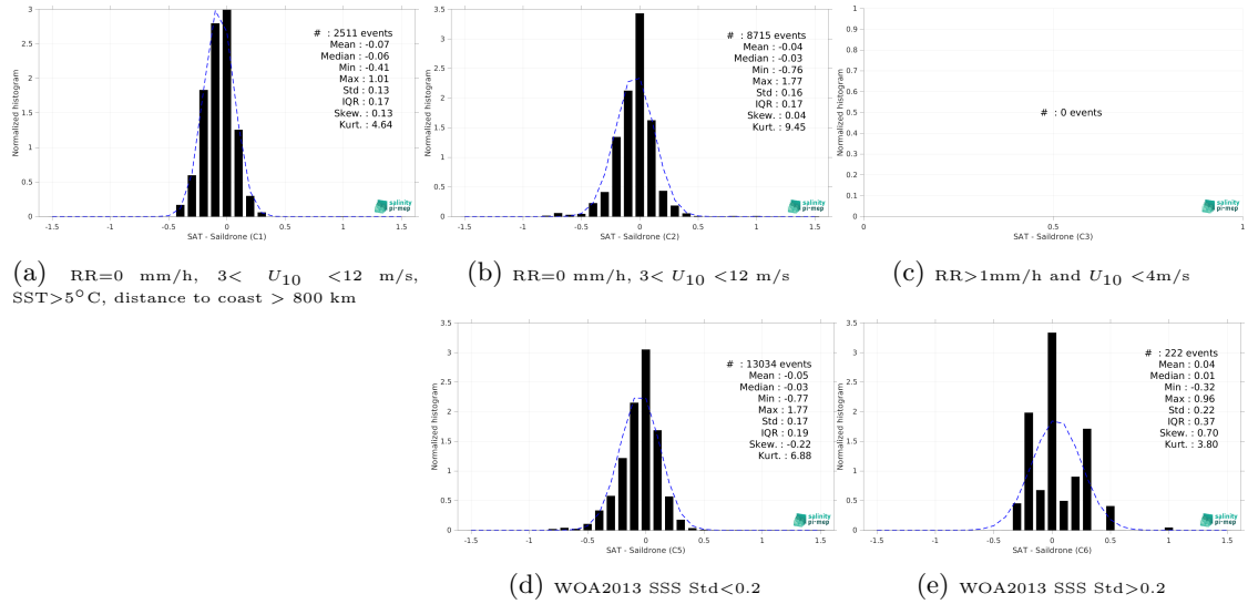
Figure 13: Normalized histogram of \Delta SSS (CCI SSS L4 POLAR SH Merged-OI v4.4 - 30-day running (ESA) - Saildrone) for 5 different subdatasets corresponding to: RR=0 mm/h, 3 < U_{10} < 12 m/s, SST > 5^\circ\text{C} , distance to coast > 800 km (a), RR=0 mm/h, 3 < U_{10} < 12 m/s (b), RR > 1\text{mm/h} and U_{10} < 4\text{m/s} (c), WOA2013 SSS Std < 0.2 (d), WOA2013 SSS Std > 0.2 (e).
