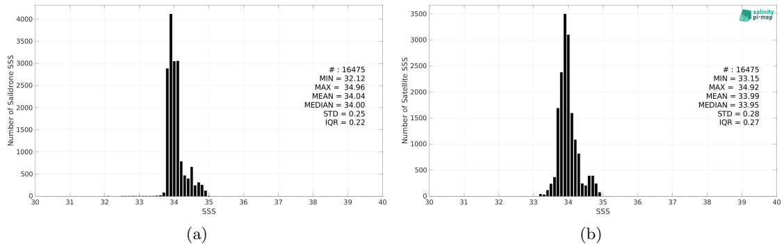
Figure 2: Histograms of SSS from Saildrone (a) and CCI SSS L4 POLAR SH Merged-OI v4.4 - 30-day running (ESA) (b) considering all match-up pairs per bins of 0.1 over the Global Ocean Pi-MEP region and for the full satellite product period.
