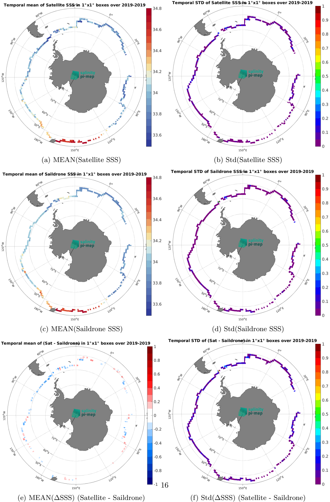
Figure 6: Temporal mean (left) and Std (right) of SSS from CCI SSS L4 POLAR SH Merged-OI v4.4 - 30-day running (ESA) (top), Saildrone (middle), and of \Delta SSS (Satellite - Saildrone). Only match-up pairs are used to generate these maps.
