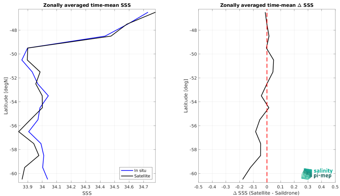
Figure 8: Left panel: Zonal mean SSS from CCI SSS L4 POLAR SH Merged-OI v4.4 - 30-day running (ESA) satellite product (black) and from Saildrone (blue). Right panel: Zonal mean of \Delta SSS (Satellite - Saildrone) for all the collected Pi-MEP match-up pairs estimated over the full satellite product period.
