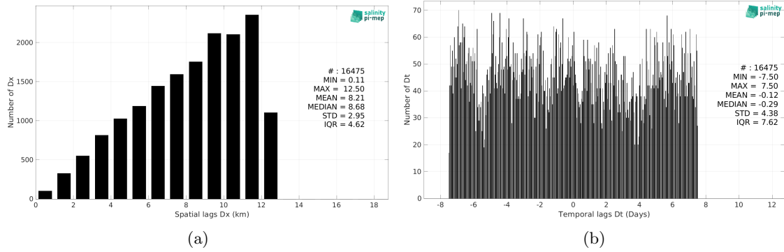
Figure 5: Histograms of the spatial (a) and temporal (b) lags between the location/time of the Saildrone measurement and the date of the corresponding CCI SSS L4 POLAR SH Merged-OI v4.4 - 30-day running (ESA) SSS pixel.
