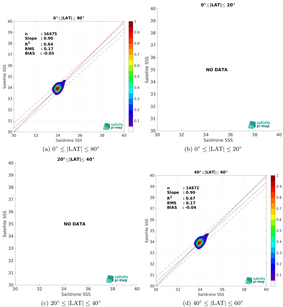
Figure 9: Contour maps of the concentration of CCI SSS L4 POLAR SH Merged-OI v4.4 - 30-day running (ESA) SSS (y-axis) versus Saildrone SSS (x-axis) at match-up pairs for different latitude bands. For each plot, the red line shows x=y . The black thin and dashed lines indicate a linear fit through the data cloud and the \pm 95\% confidence levels, respectively. The number match-up pairs n , the slope and R^2 coefficient of the linear fit, the root mean square (RMS) and the mean bias between satellite and in situ data are indicated for each latitude band in each plots.
