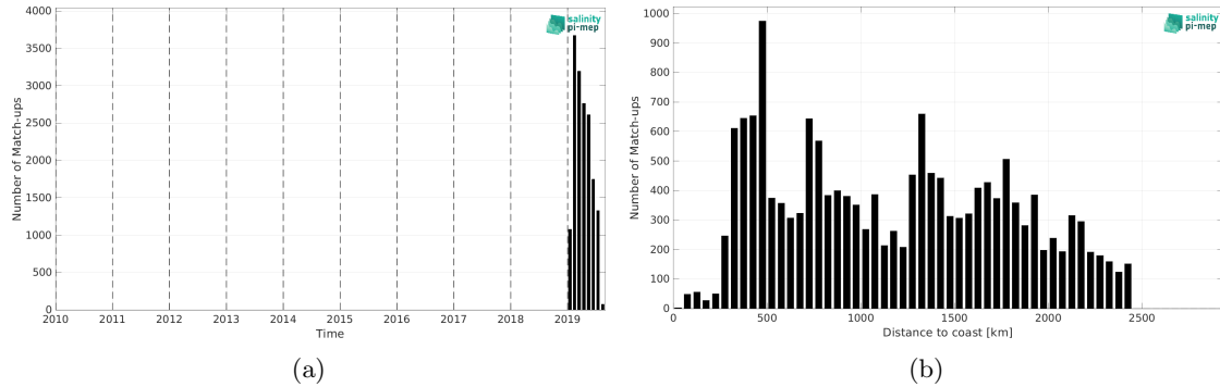
Figure 1: Number of match-ups between Saildrone and CCI SSS L4 POLAR SH Merged-OI v4.4 - 30-day running (ESA) SSS as a function of time (a) and as function of the distance to coast (b) over the Global Ocean Pi-MEP region and for the full satellite product period.
