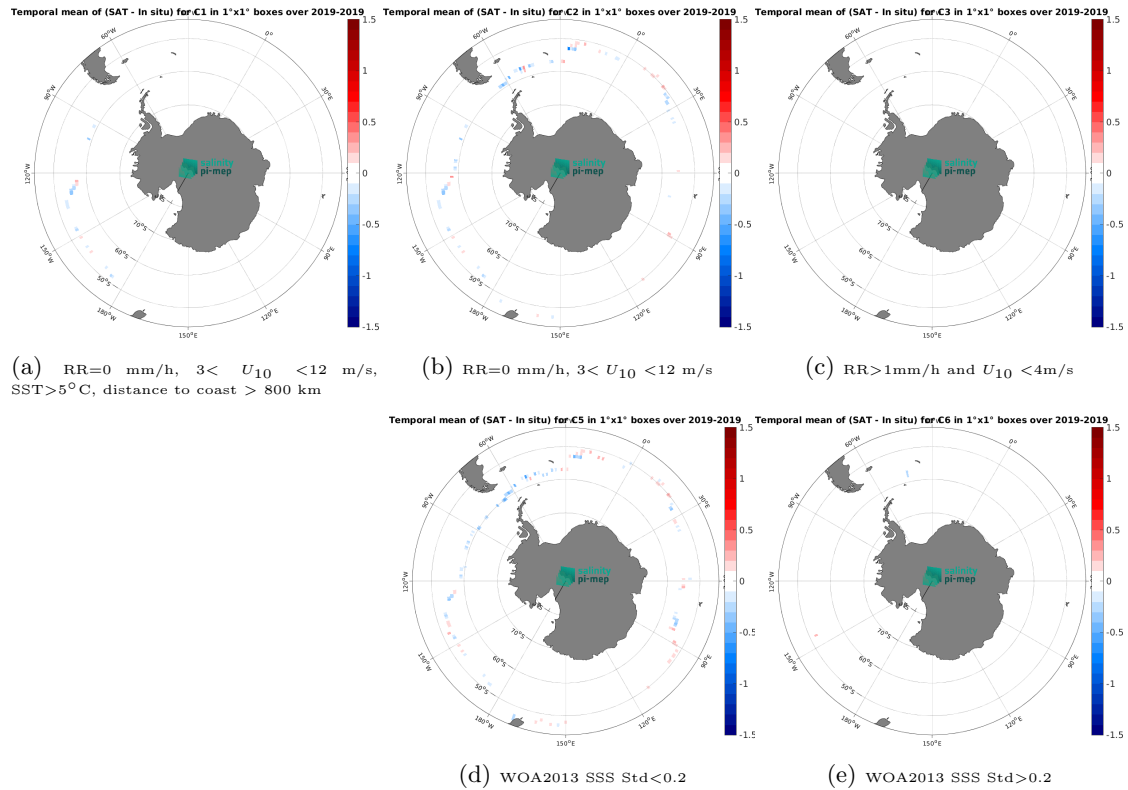
Figure 12: Temporal mean gridded over spatial boxes of size 1^{\circ}\times 1^{\circ} of \Delta\text{SSS} (CCI SSS L4 POLAR SH Merged-OI v4.4 - 30-day running (ESA) - Saldrone) for 5 different subdatasets corresponding to:RR=0 mm/h, 3 < U_{10} < 12 m/s, SST >5^{\circ}\text{C} , distance to coast > 800 km (a), RR=0 mm/h, 3 < U_{10} < 12 m/s (b), RR >1 mm/h and U_{10} < 4 m/s (c), WOA2013 SSS Std <0.2 (d), WOA2013 SSS Std >0.2 (e).
