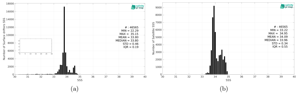
Figure 2: Histograms of SSS from Surface drifters (a) and CCI SSS L4 POLAR SH Merged-OI v4.4 - 30-day running (ESA) (b) considering all match-up pairs per bins of 0.1 over the Global Ocean Pi-MEP region and for the full satellite product period.
