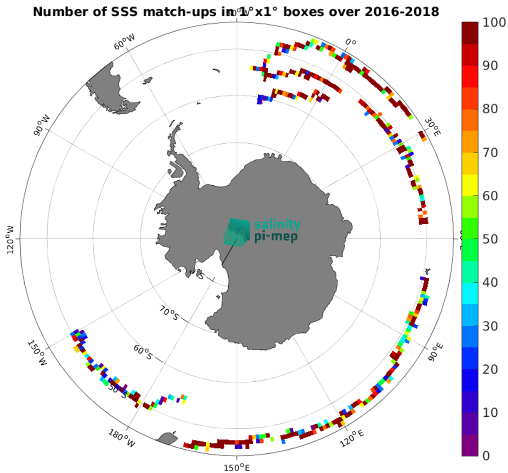
Figure 3: Number of SSS match-ups between Surface drifters SSS and the CCI SSS L4 POLAR SH Merged-OI v4.4 - 30-day running (ESA) SSS product for the Global Ocean Pi-MEP region over 1^\circ \times 1^\circ boxes and for the full satellite product period.
