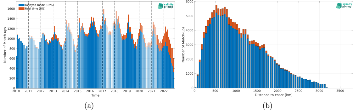
Figure 1: Number of match-ups between Argo and CCI SSS L4 POLAR SH Merged-OI v4.4 - 30-day running (ESA) SSS as a function of time (a) and as function of the distance to coast (b) over the Global Ocean Pi-MEP region and for the full satellite product period.
