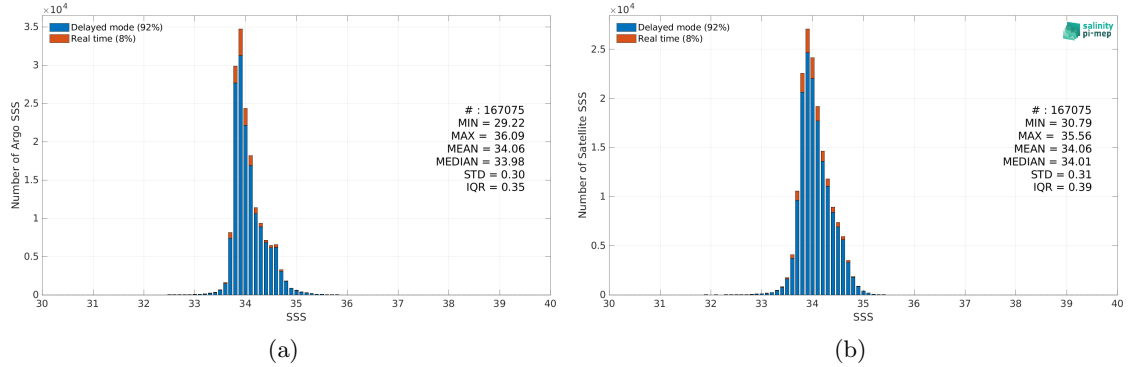
Figure 2: Histograms of SSS from Argo (a) and CCI SSS L4 POLAR SH Merged-OI v4.4 - 30-day running (ESA) (b) considering all match-up pairs per bins of 0.1 over the Global Ocean Pi-MEP region and for the full satellite product period.
