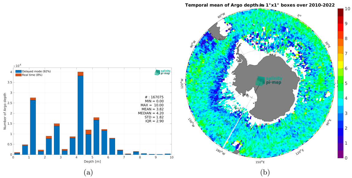
Figure 3: Histograms of the depth of the upper level SSS measurements from Argo in the Match-up DataBase for the Global Ocean Pi-MEP region (a) and temporal mean spatial distribution of pressure of the in situ SSS data over 1^\circ \times 1^\circ boxes and for the full satellite product period (b).
