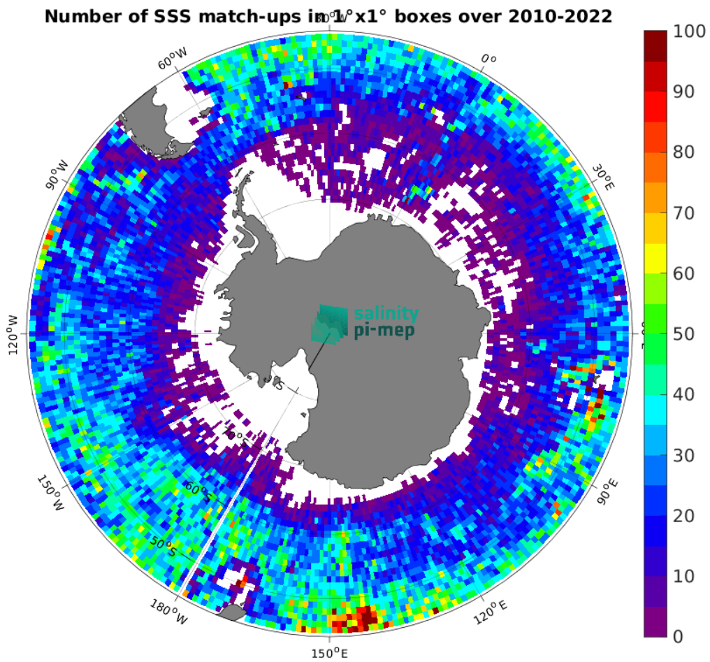
Figure 4: Number of SSS match-ups between Argo SSS and the CCI SSS L4 POLAR SH Merged-OI v4.4 - 30-day running (ESA) SSS product for the Global Ocean Pi-MEP region over 1^\circ \times 1^\circ boxes and for the full satellite product period.
