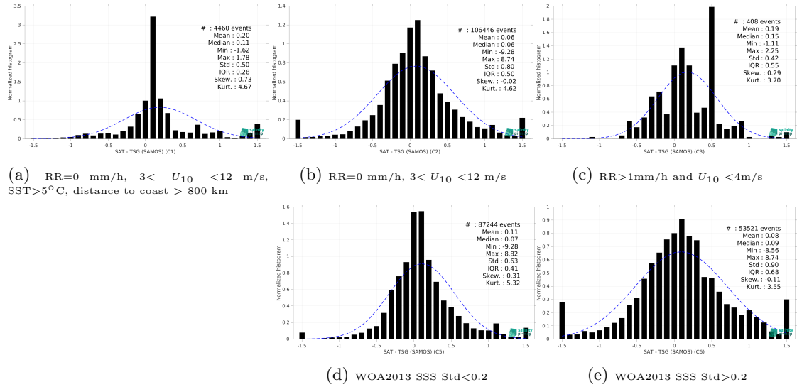
Figure 15: Normalized histogram of \Delta\text{SSS} (CCI SSS L4 POLAR NH Merged-OI v4.41 - 7-day running (ESA) - TSG (SAMOS)) for 5 different subdatasets corresponding to: RR=0 mm/h, 3 < U_{10} < 12 m/s, SST > 5^\circ\text{C} , distance to coast > 800 km (a), RR=0 mm/h, 3 < U_{10} < 12 m/s (b), RR > 1 mm/h and U_{10} < 4 m/s (c), WOA2013 SSS Std < 0.2 (d), WOA2013 SSS Std > 0.2 (e).
