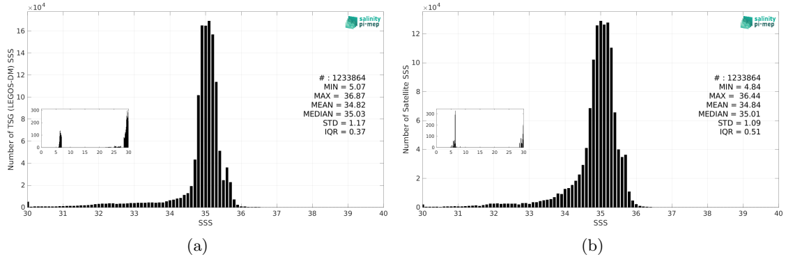
Figure 3: Histograms of SSS from TSG (LEGOS-DM) (a) and CCI SSS L4 POLAR NH Merged-OI v4.41 - 7-day running (ESA) (b) considering all match-up pairs per bins of 0.1 over the Global Ocean Pi-MEP region and for the full satellite product period.
