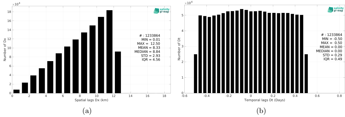
Figure 6: Histograms of the spatial (a) and temporal (b) lags between the location/time of the TSG (LEGOS-DM) measurement and the date of the corresponding CCI SSS L4 POLAR NH Merged-OI v4.41 - 7-day running (ESA) SSS pixel.
