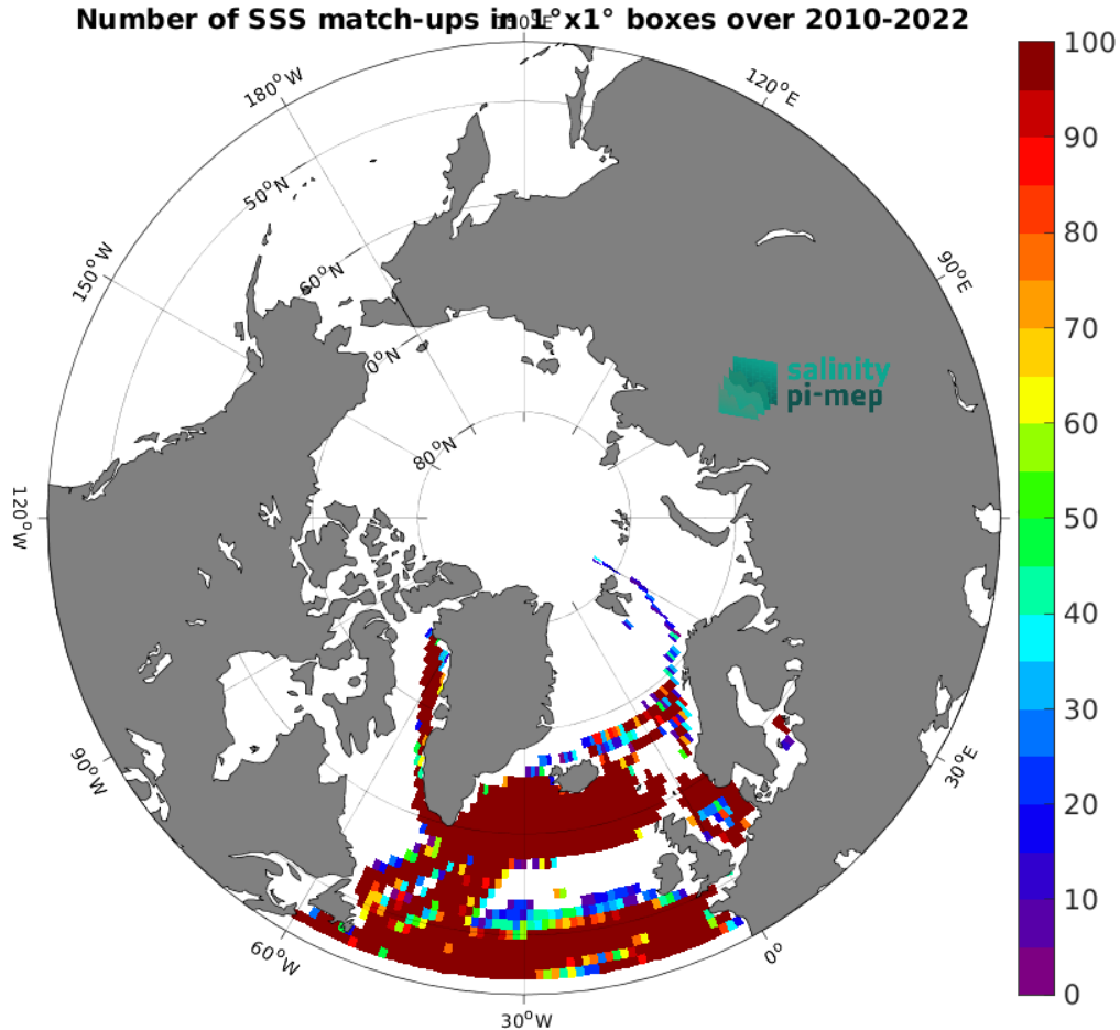
Figure 5: Number of SSS match-ups between TSG (LEGOS-DM) SSS and the CCI SSS L4 POLAR NH Merged-OI v4.41 - 7-day running (ESA) SSS product for the Global Ocean Pi-MEP region over 1^\circ \times 1^\circ boxes and for the full satellite product period.
