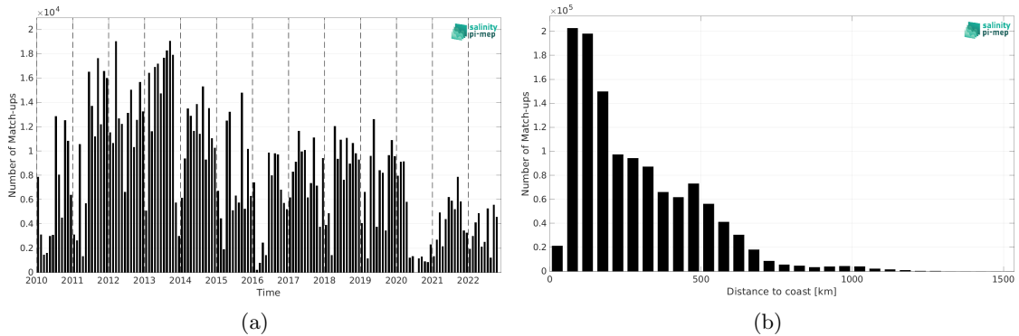
Figure 2: Number of match-ups between TSG (LEGOS-DM) and CCI SSS L4 POLAR NH Merged-OI v4.41 - 7-day running (ESA) SSS as a function of time (a) and as function of the distance to coast (b) over the Global Ocean Pi-MEP region and for the full satellite product period.
